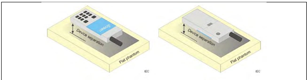
Test positions for body-worn device
