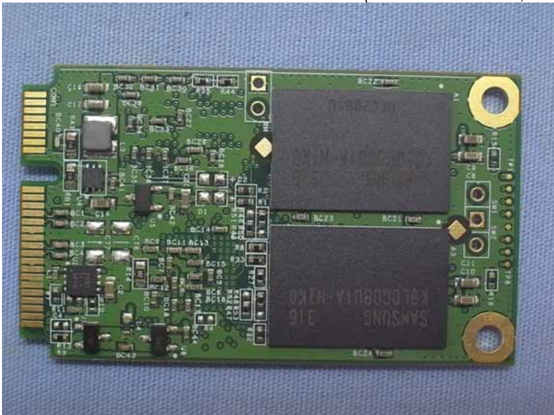
Photo 22 Internal View (Transcend SSD Card, Back View)
