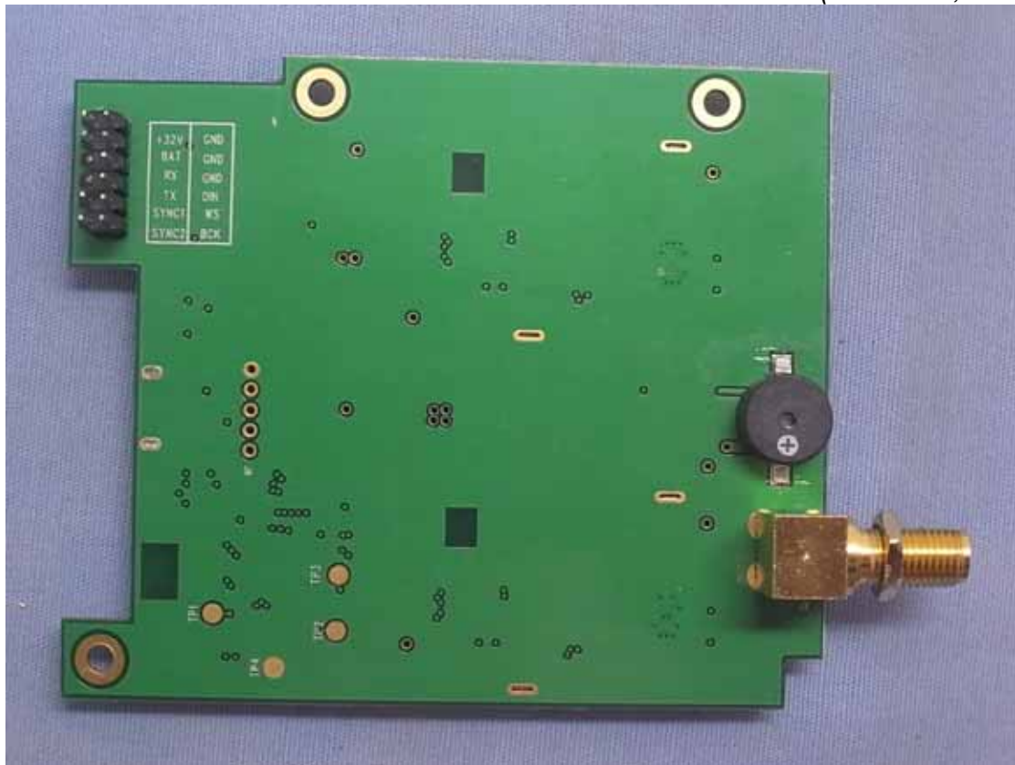
Photo 19 Internal View (RF Board, Back View)
