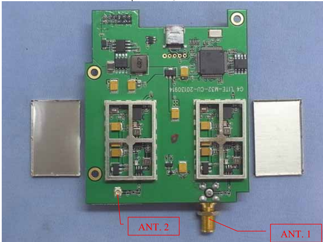
Internal View (RF Board, Front View With Removed Shielded Cover)
