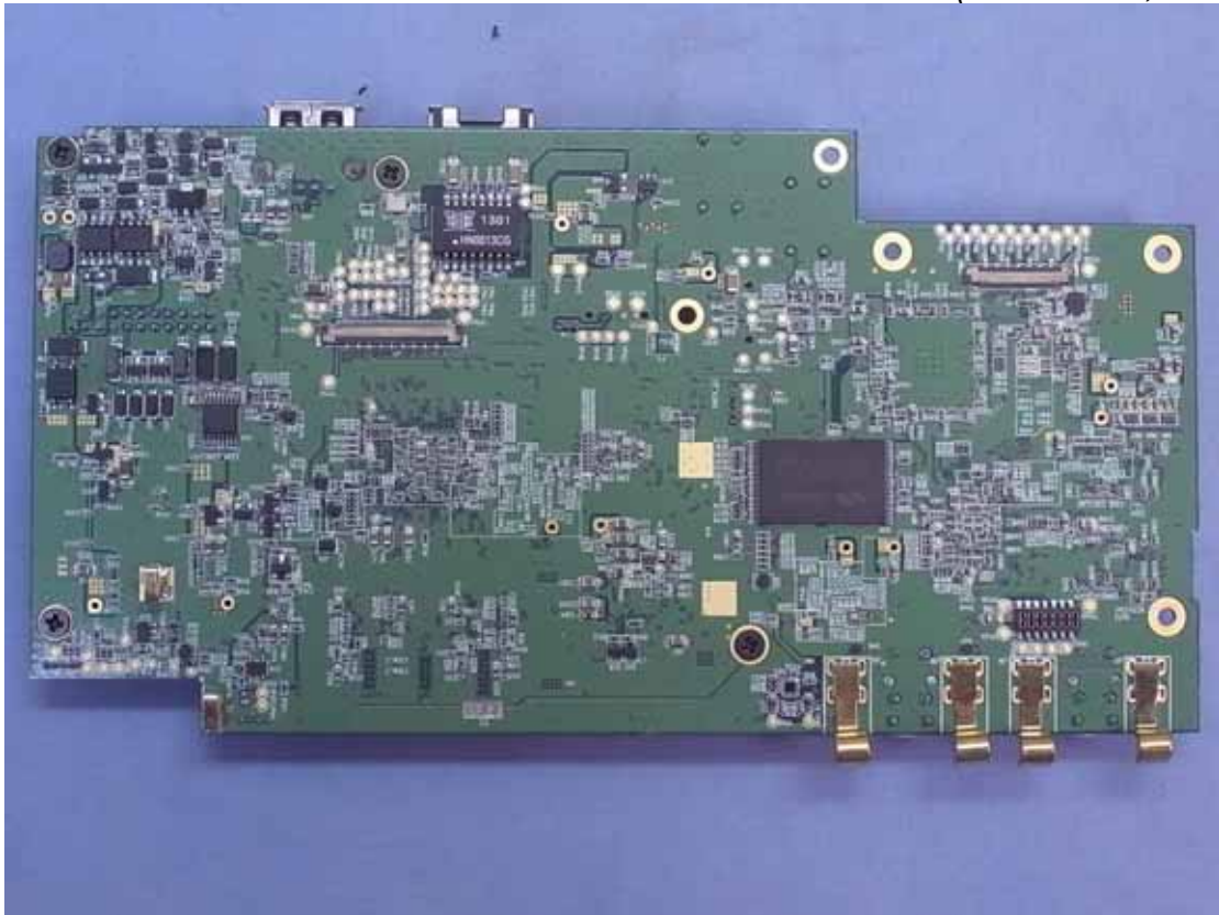
Photo 27 Internal View (Main Board, Back View)
