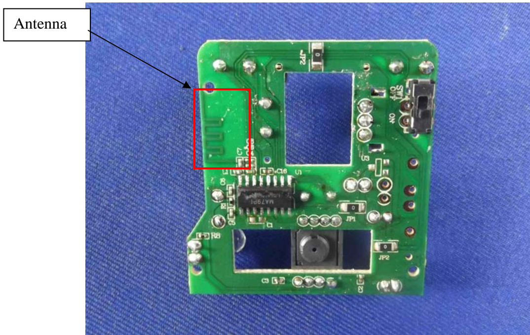
Figure 10 PCB of the EUT-Module View
