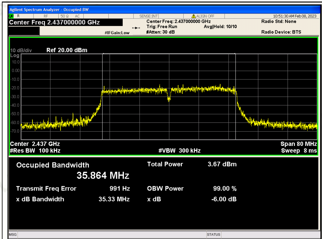
CH06: 2437MHz
