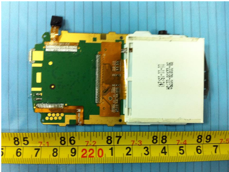
EUT – Main Board LCD Display off View
