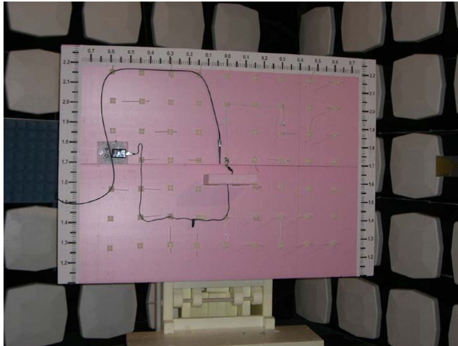
FCC Part 15C Radiated Emissions Test Setup
