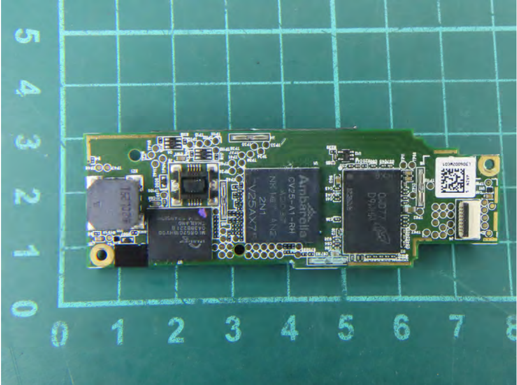
(23) EUT Photo
