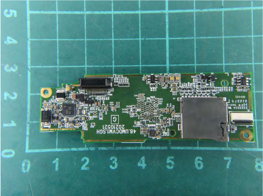
(26) EUT Photo
