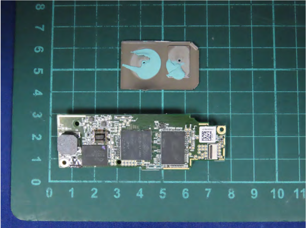
(22) EUT Photo
