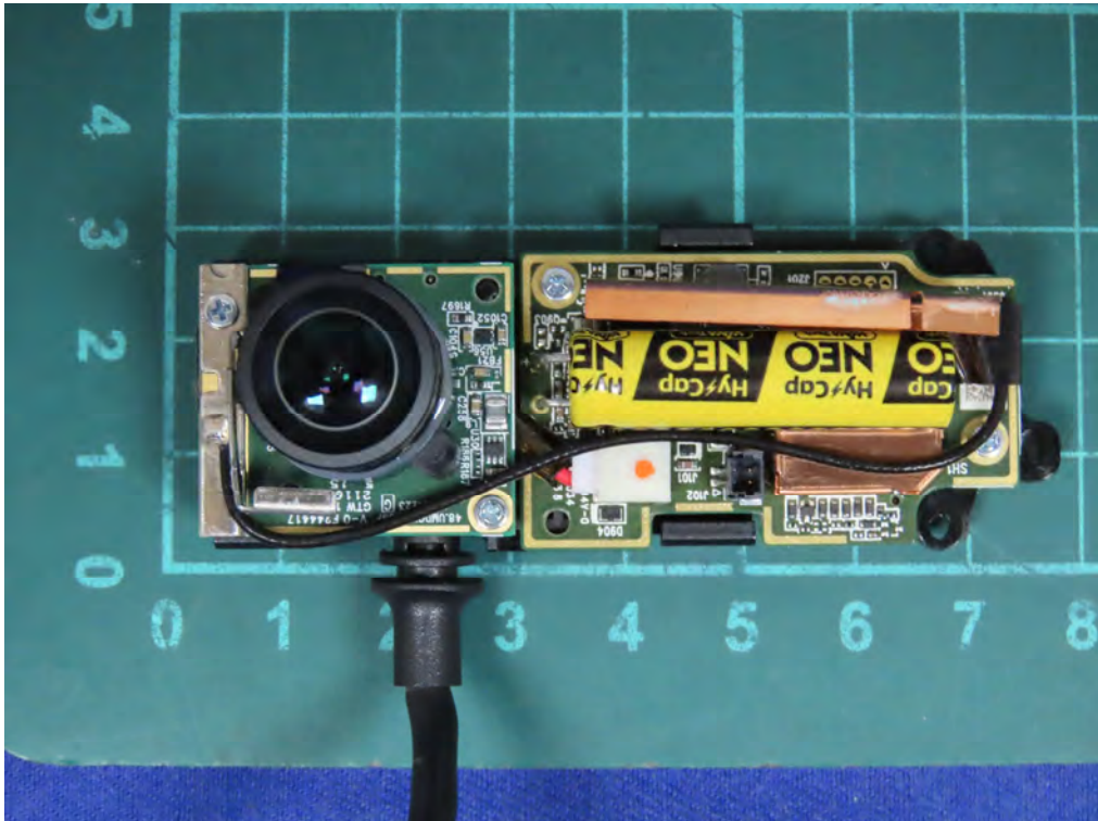
(29) EUT Photo
