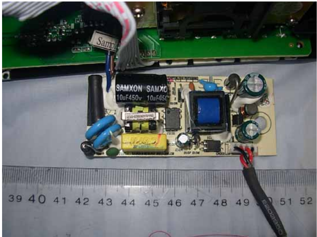
FIGURE 4 DIGITAL SET-TOP (M/N: CISCO 3413DVB) POWER BOARD #2 (COMPONENT SIDE)
