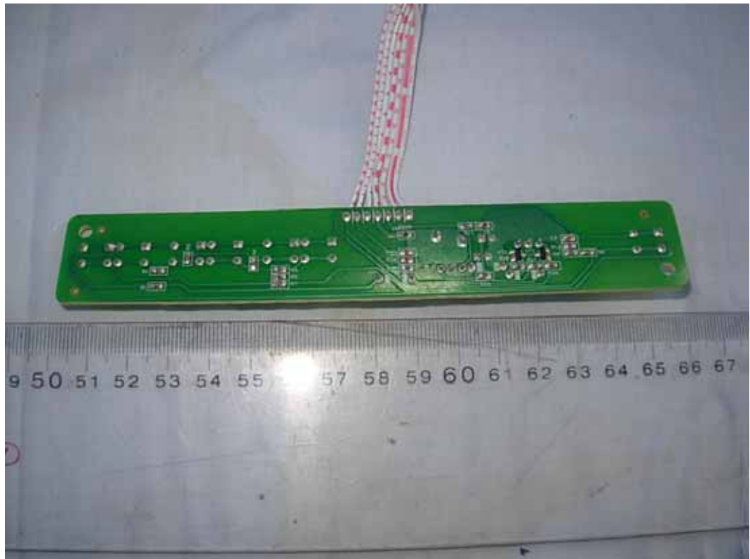
FIGURE 12 DIGITAL SET-TOP (M/N: CISCO 3413DVB) KEY BOARD (SOLDERED SIDE)
