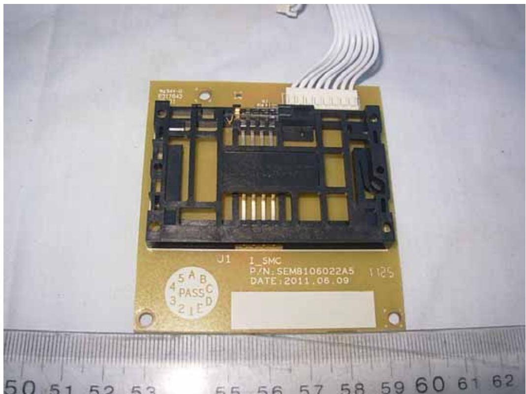
FIGURE 13 DIGITAL SET-TOP (M/N: CISCO 3413DVB) I_SMC BOARD (COMPONENT SIDE)
