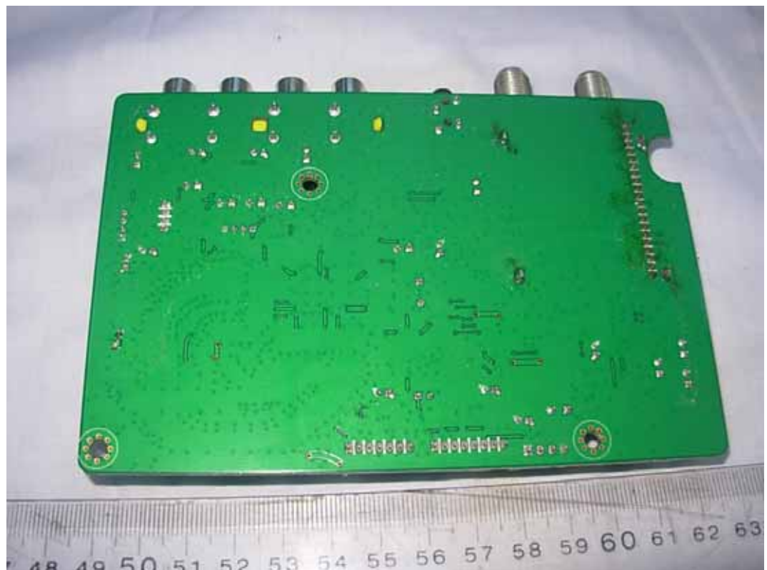
FIGURE 7 DIGITAL SET-TOP (M/N: CISCO 3413DVB) MAIN BOARD (SOLDERED SIDE)
