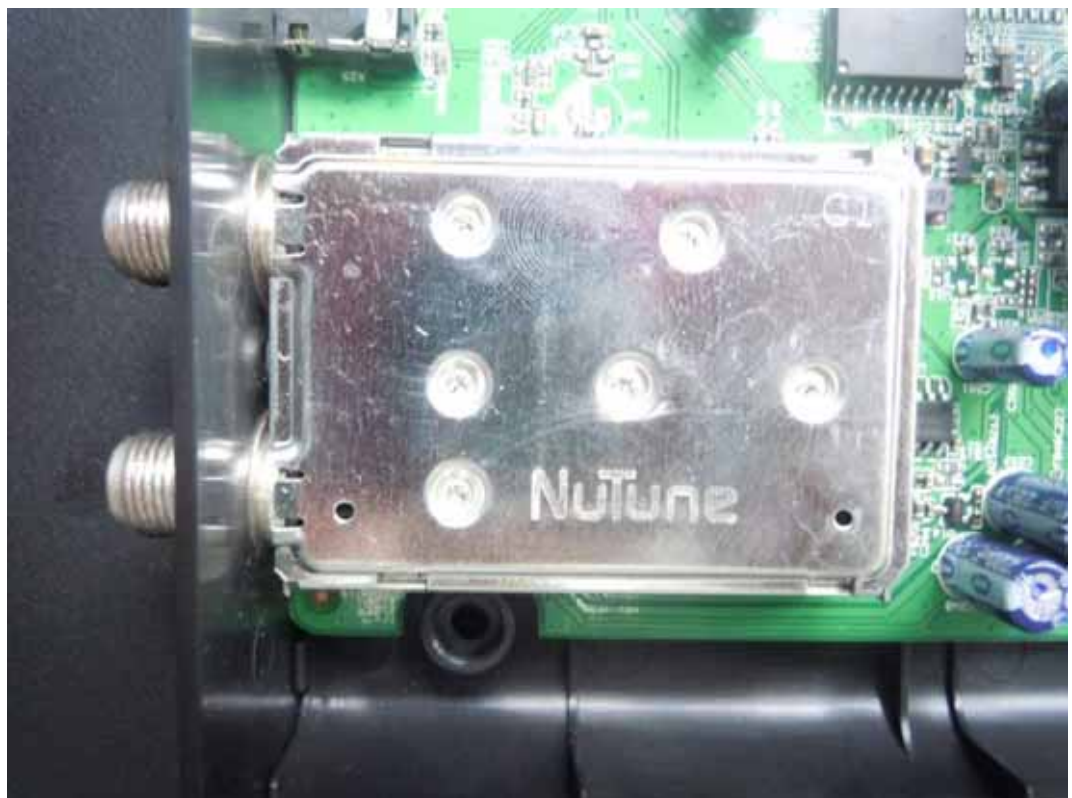
FIGURE 9 DIGITAL SET-TOP (M/N: CISCO 3413DVB) TUNER ON MAIN BOARD
