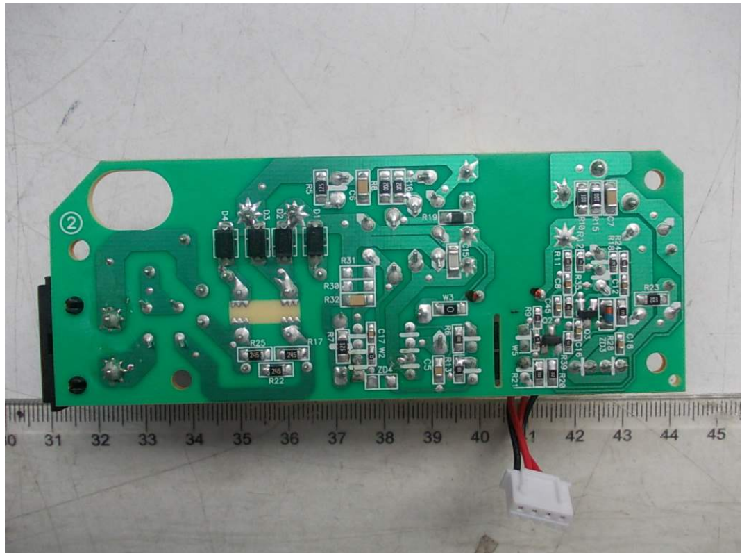
DIGITAL SET-TOP (M/N: PDS2100) POWER BOARD (SOLDERED SIDE)
