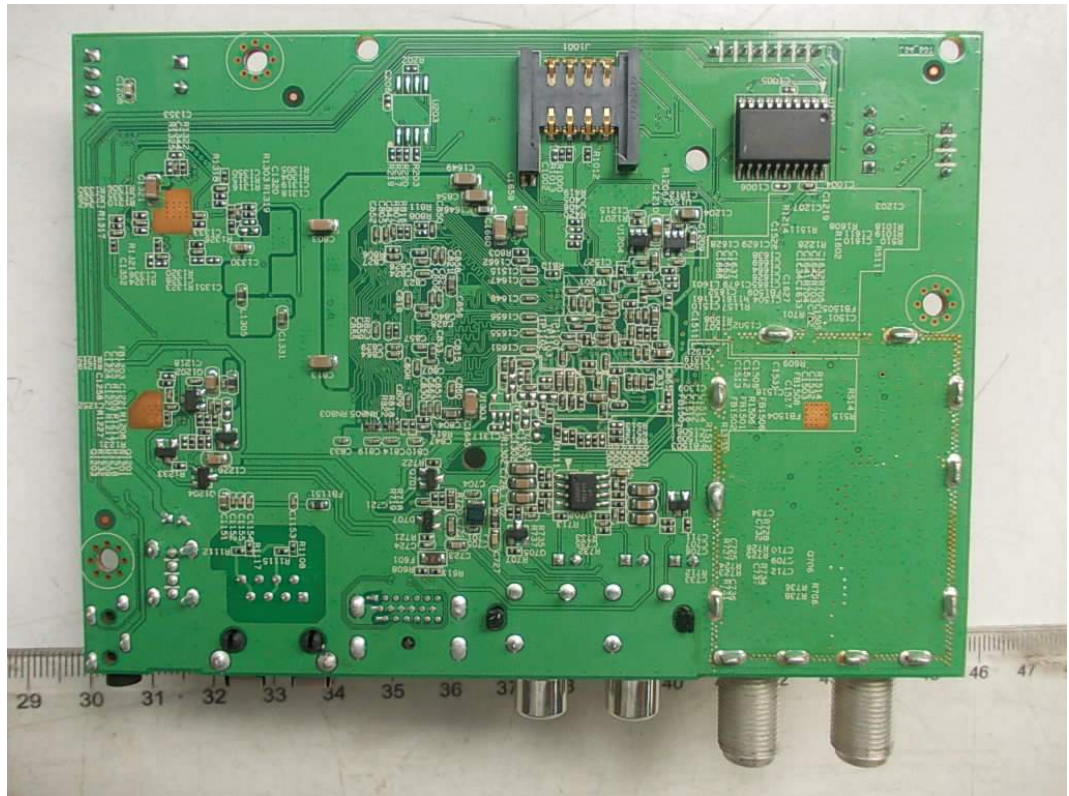
FIGURE 6 DIGITAL SET-TOP (M/N: PDS2100) CHIP & CRYSTAL ON MAIN BOARD
