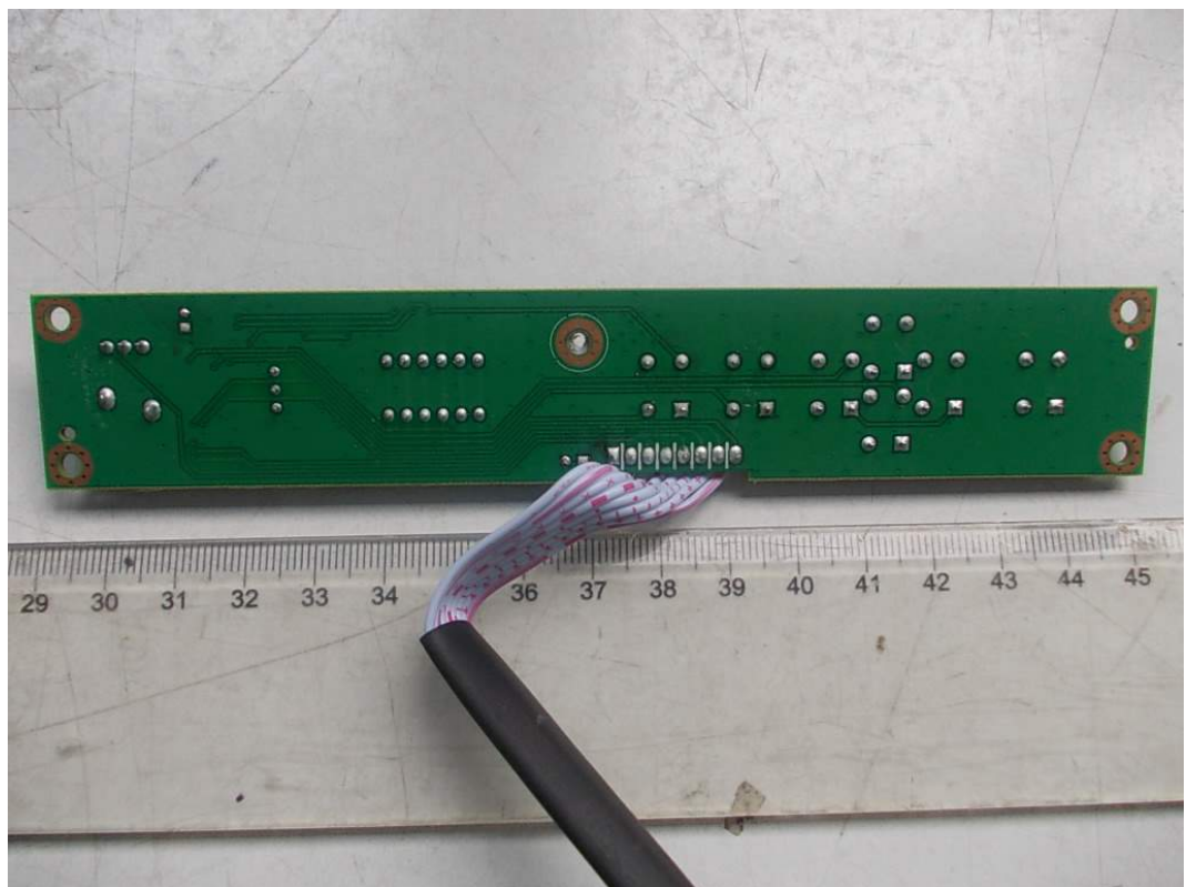
FIGURE 8 DIGITAL SET-TOP (M/N: PDS2100) KEY BOARD (SOLDERED SIDE)
