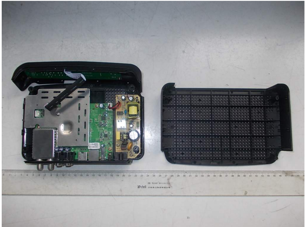
FIGURE 1 DIGITAL SET-TOP (M/N: PDS2100) COVER REMOVED
