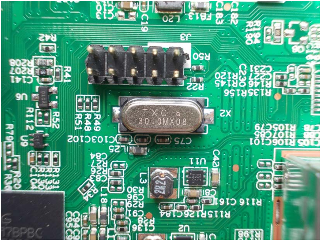
FIGURE 7 DIGITAL SET-TOP (M/N: PDS1100) CRYSTAL ON MAIN BOARD
