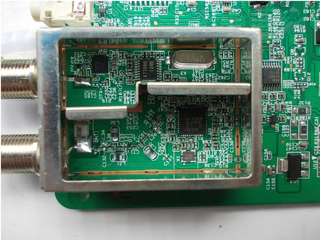
FIGURE 10 DIGITAL SET-TOP (M/N: PDS1100) TUNER (COVER REMOVED)
