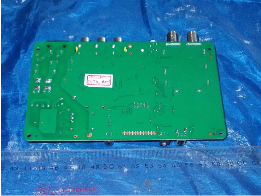
FIGURE 6 DIGITAL SET-TOP (M/N: PDS1100) MAIN BOARD (SOLDERED SIDE)
