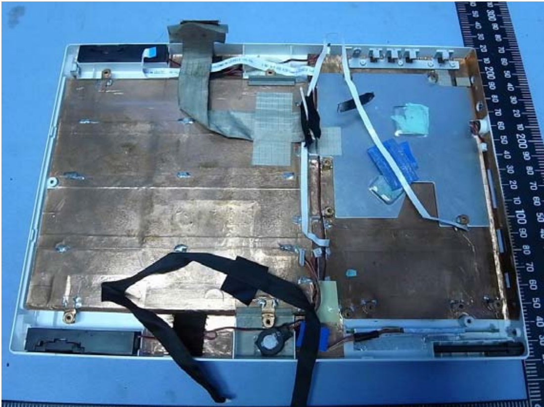
Figure 24 Internal View
