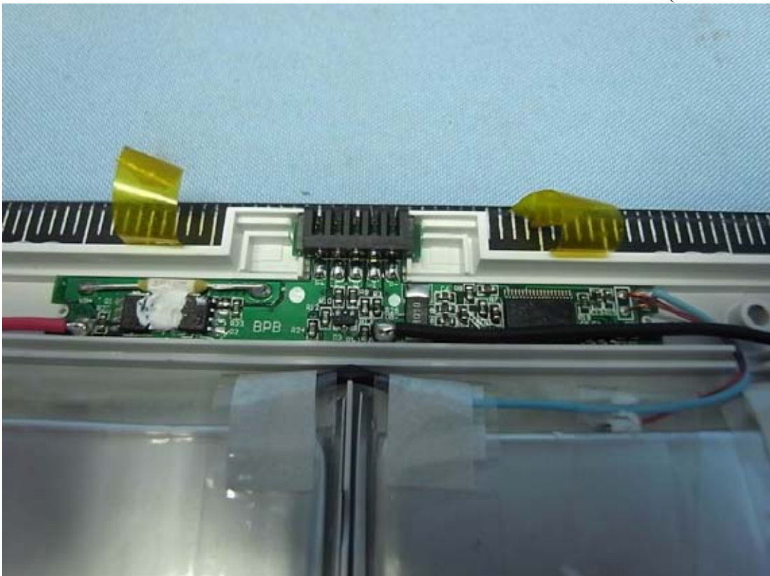
Figure 31 Internal View (Control Board)
