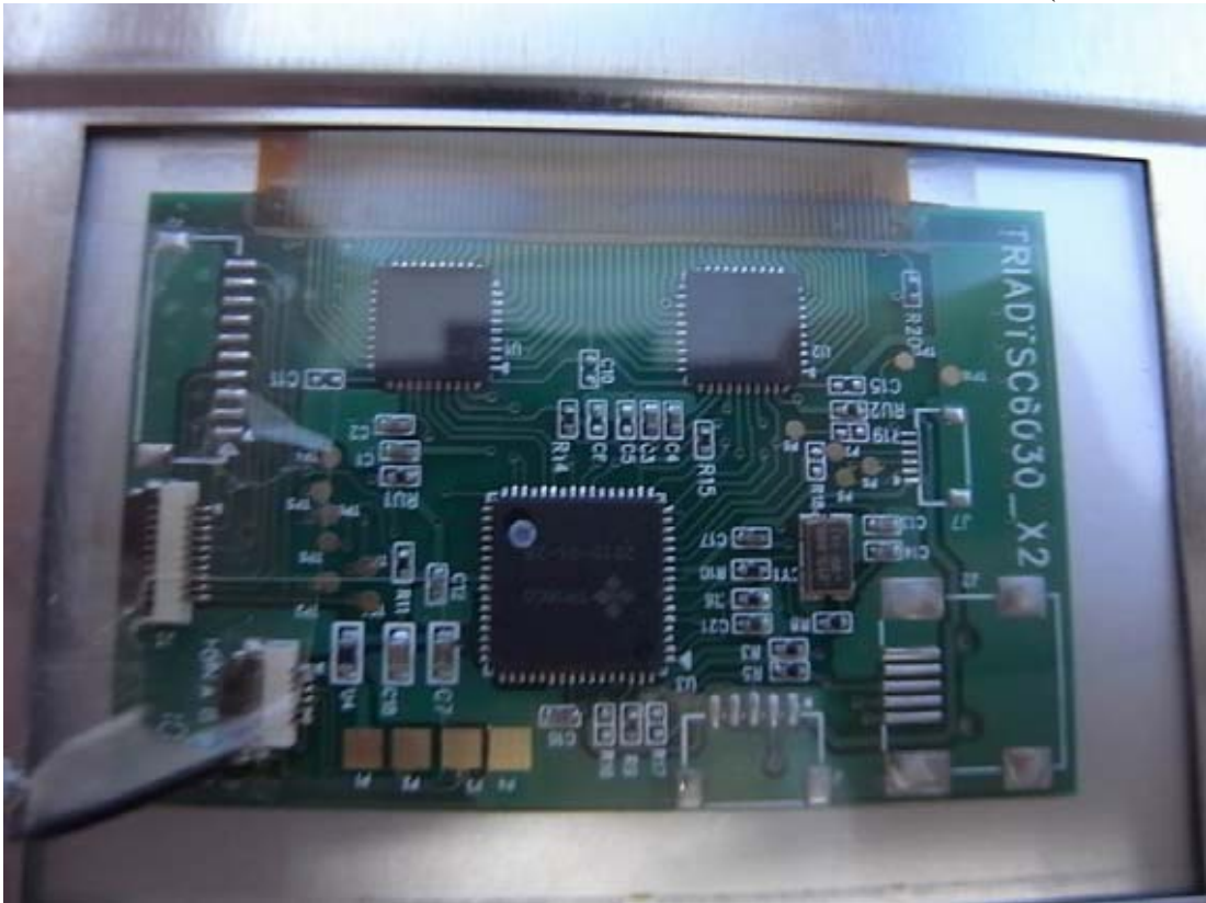
Figure 16 Internal View (Control Board)
