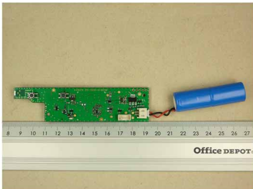
140898_10.jpg: Bottom view of PCB
