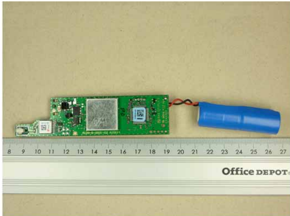
140898_9.jpg: Top view of PCB
