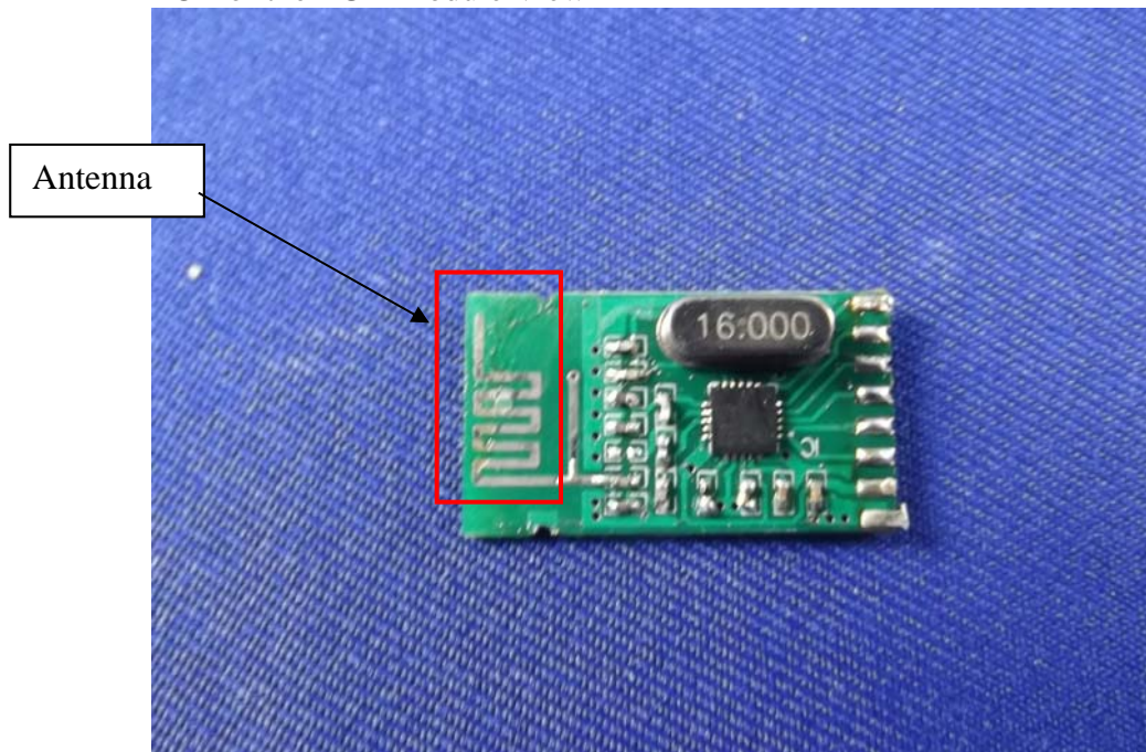
Figure 11 PCB of the EUT-Module View
