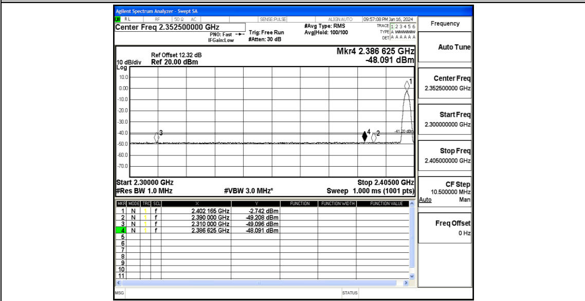
2DH5_Ant1_Low_2402_Peak
