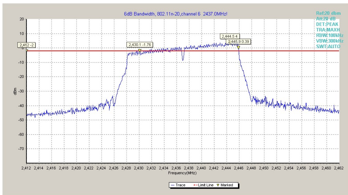
Fig.A.4.12 Occupied 6dB Bandwidth (802.11n-HT20, Ch 6)
