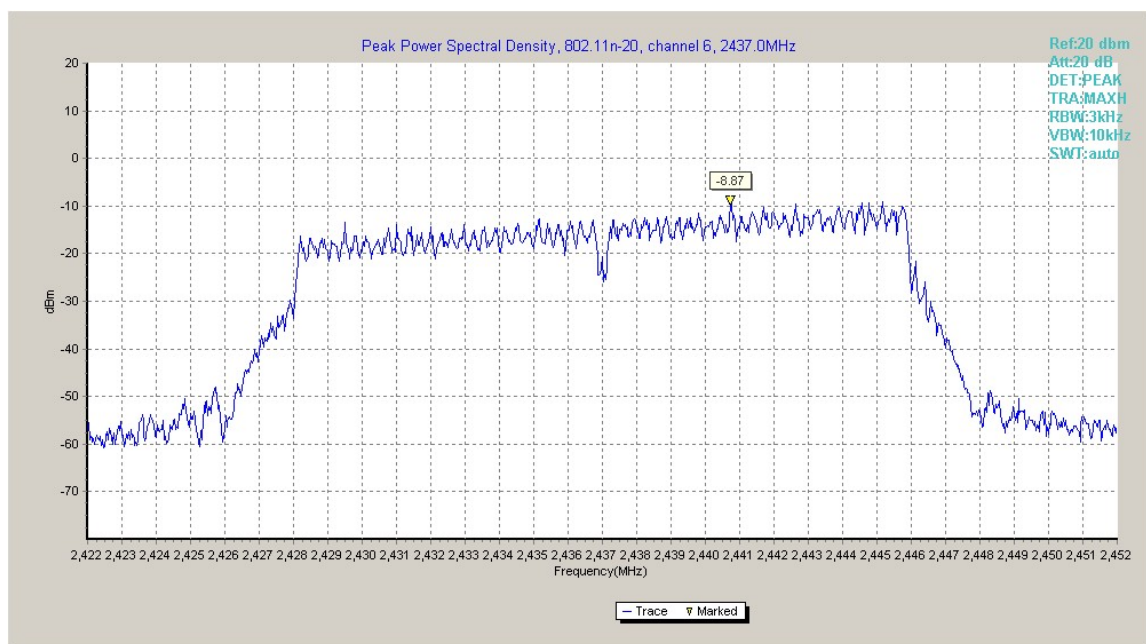
Fig.A.3.12 Power Spectral Density (802.11n-HT20, Ch 6)
