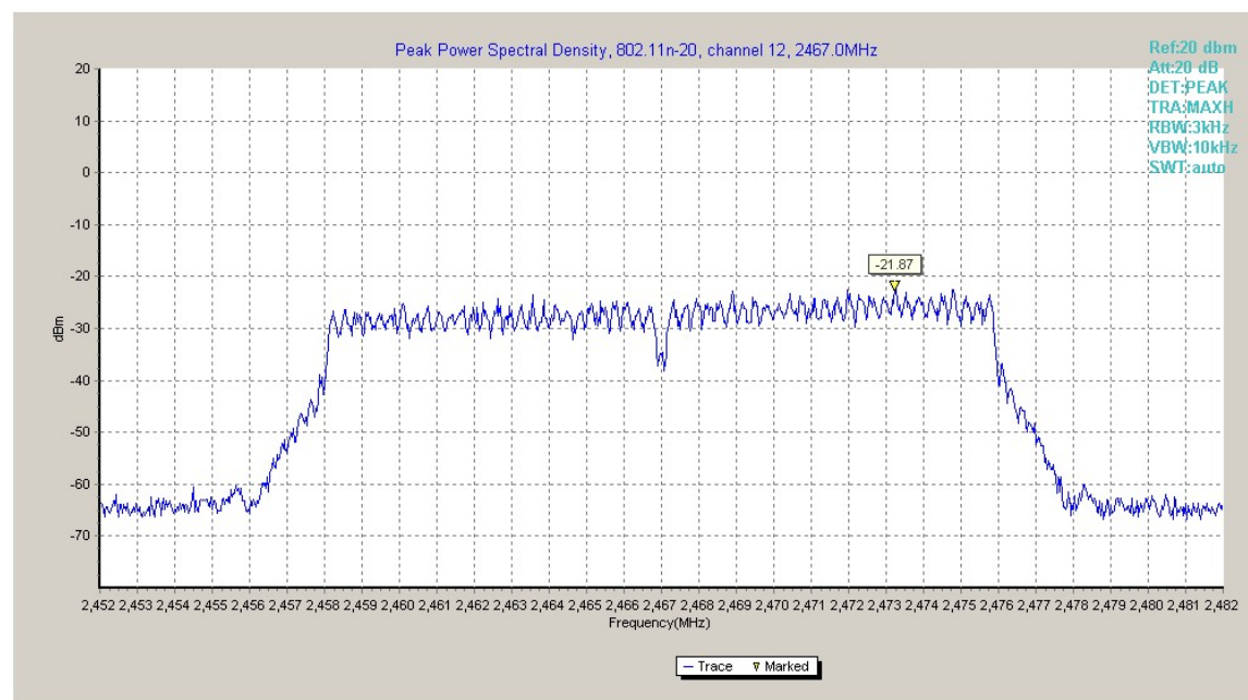
Fig.A.3.14 Power Spectral Density (802.11n-HT20, Ch 12)
