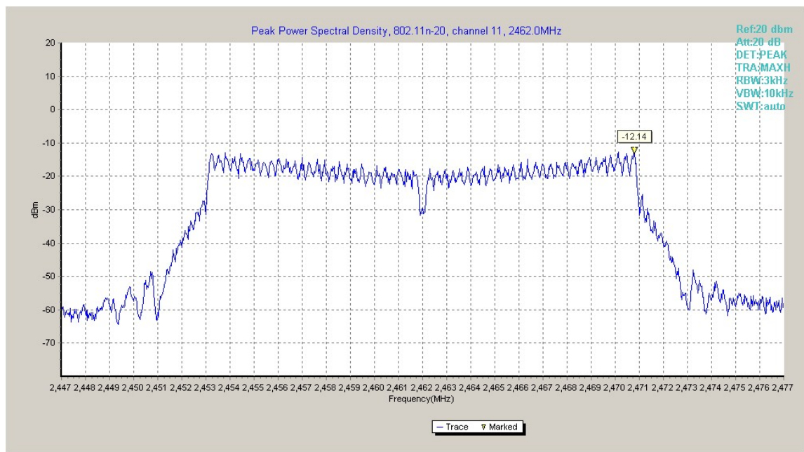
Fig.A.3.13 Power Spectral Density (802.11n-HT20, Ch 11)
