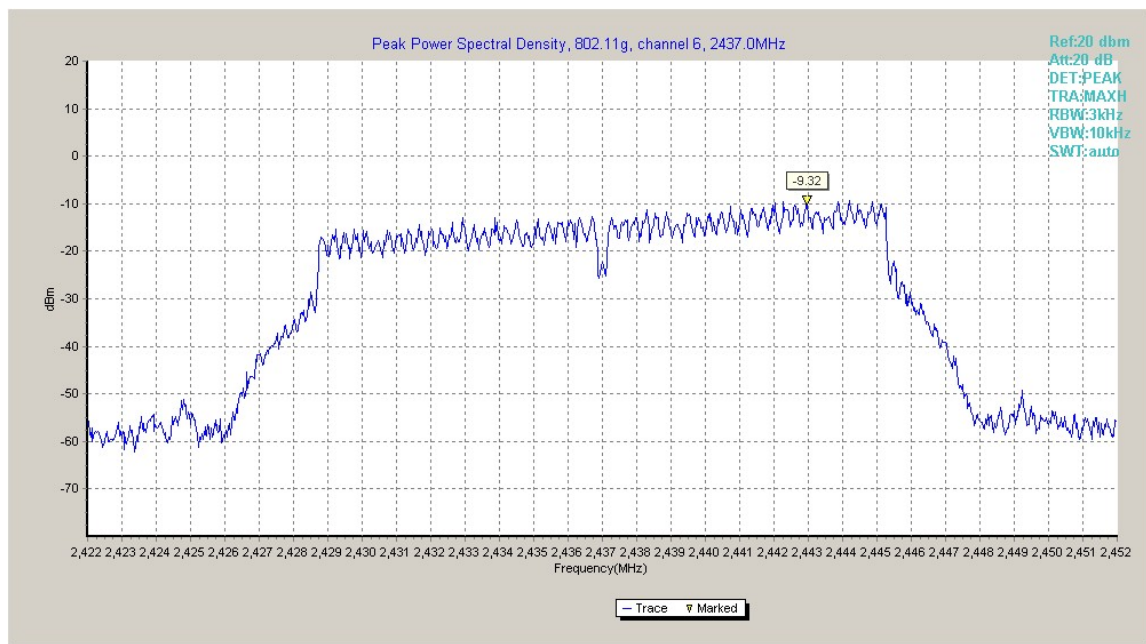
Fig.A.3.7 Power Spectral Density (802.11g, Ch 6)
