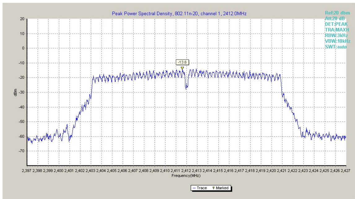
Fig.A.3.11 Power Spectral Density (802.11n-HT20, Ch 1)
