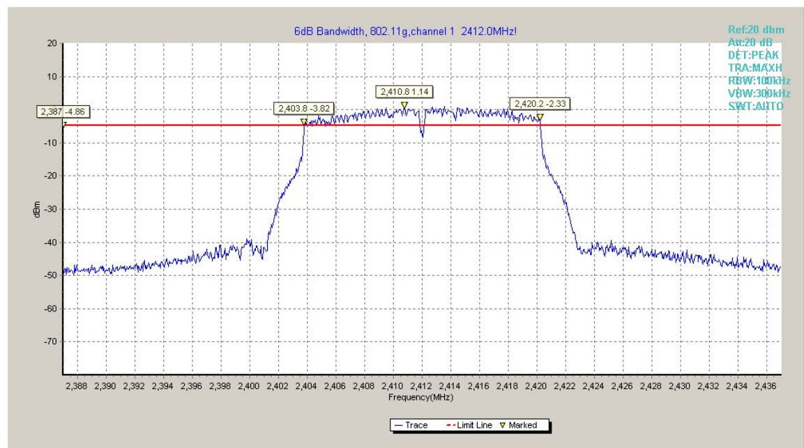
Fig.A.4.6 Occupied 6dB Bandwidth (802.11g, Ch 1)
