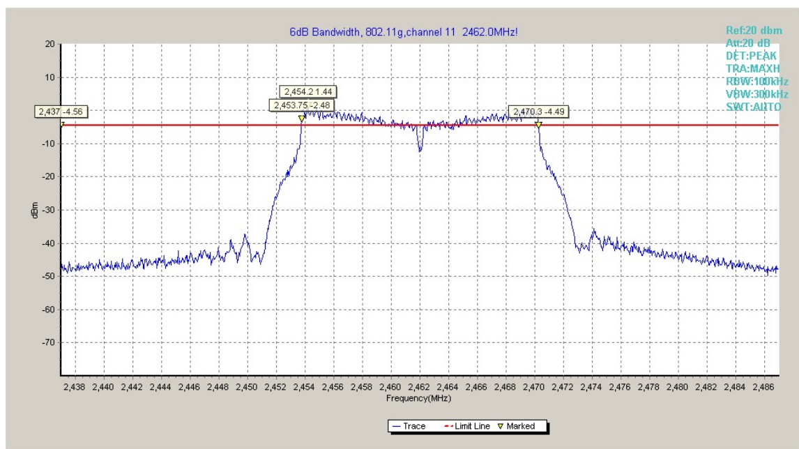
Fig.A.4.8 Occupied 6dB Bandwidth (802.11g, Ch 11)
