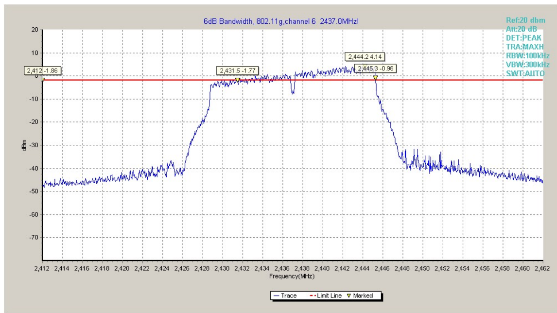
Fig.A.4.7 Occupied 6dB Bandwidth (802.11g, Ch 6)
