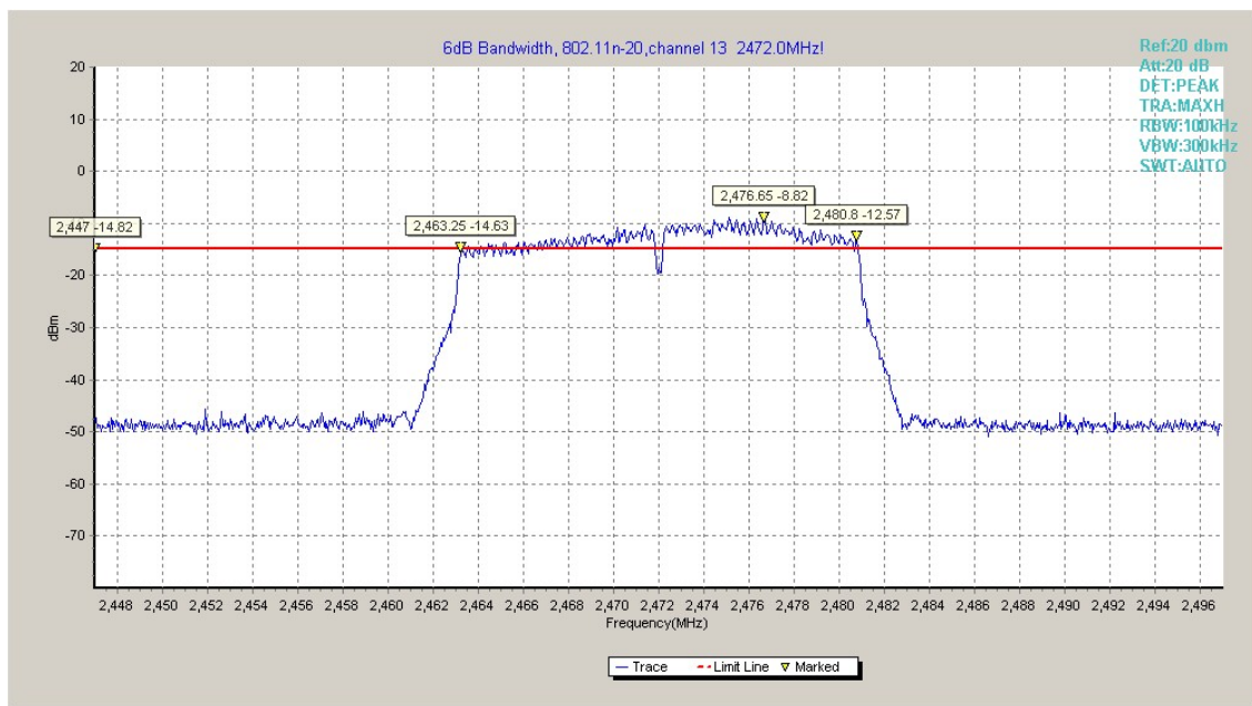
Fig.A.4.15 Occupied 6dB Bandwidth (802.11n-HT20, Ch 13)
