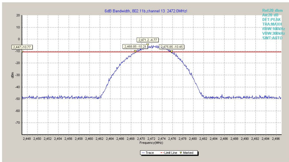
Fig.A.4.5 Occupied 6dB Bandwidth (802.11b, Ch 13)
