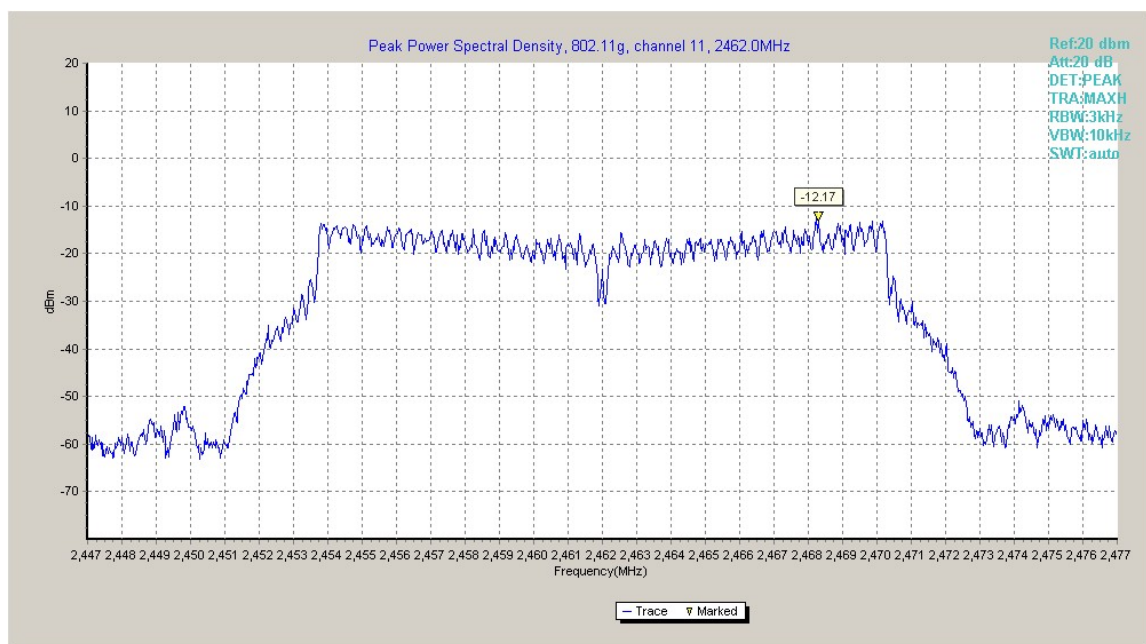
Fig.A.3.8 Power Spectral Density (802.11g, Ch 11)
