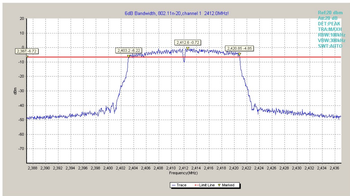
Fig.A.4.11 Occupied 6dB Bandwidth (802.11n-20MHz, Ch 1)
