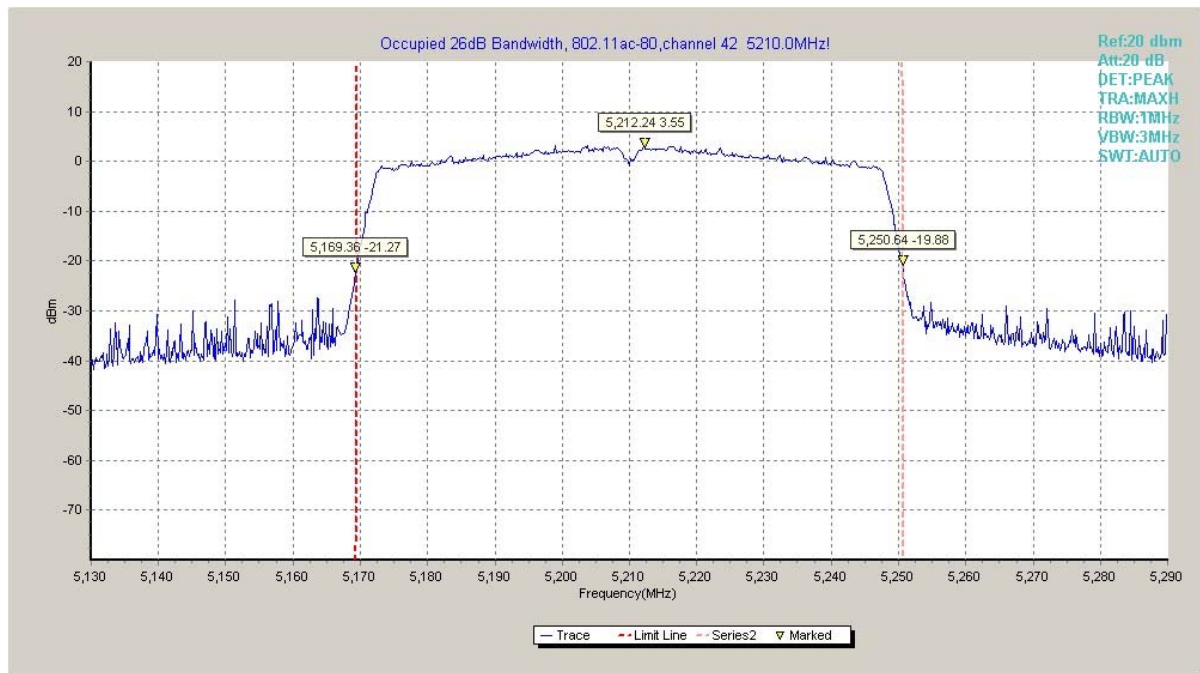
Fig. 47 Occupied 26dB Bandwidth (802.11ac80, 5210MHz)
