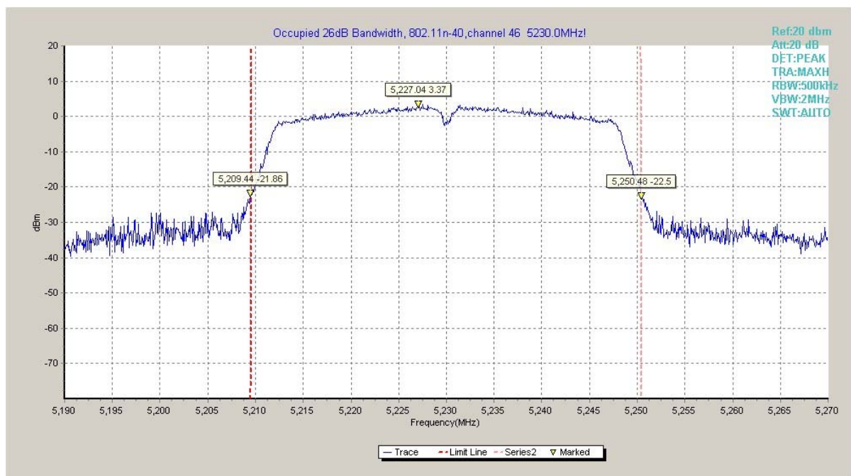
Fig. 32 Occupied 26dB Bandwidth (802.11n40, 5230MHz)
