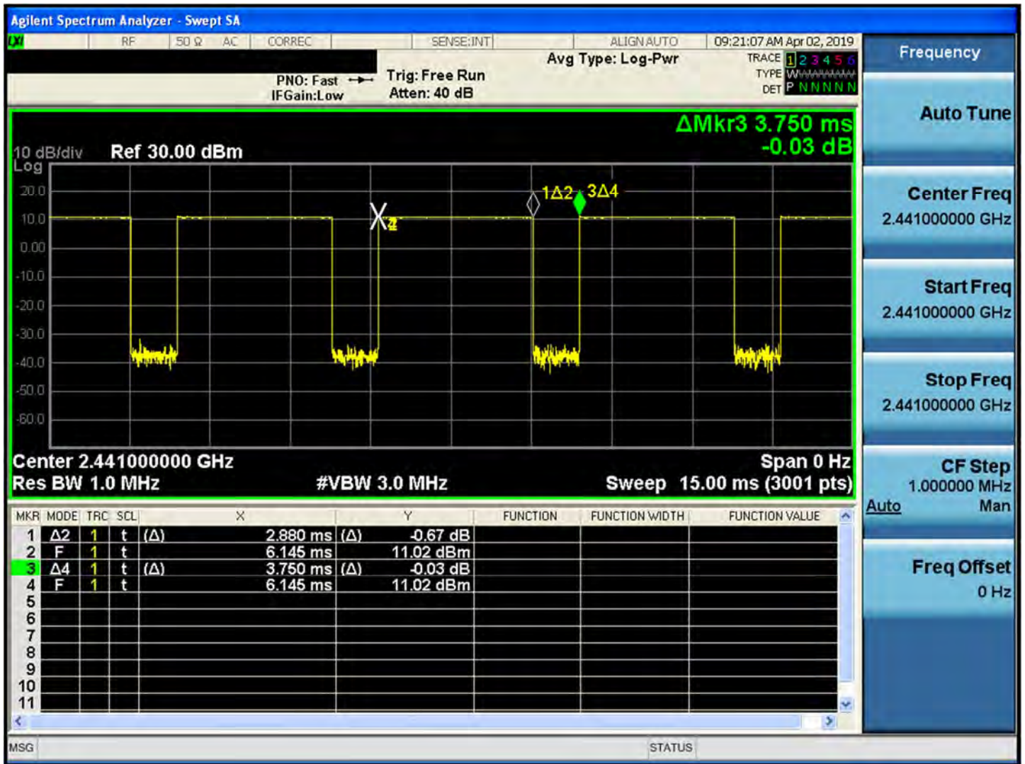
Figure 8.4.2 Bluetooth Transmission Plot
