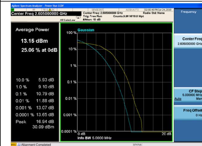
5MHz/16QAM/Mid CH
