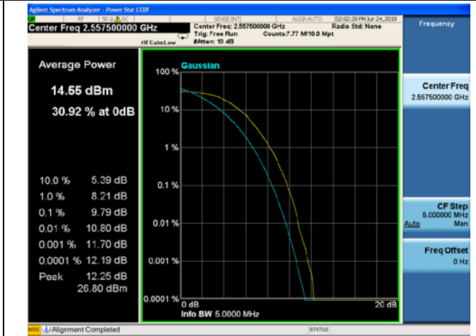
5MHz/QPSK/Mid CH
