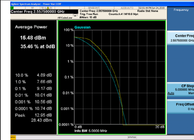
5MHz/64QAM/Low CH
