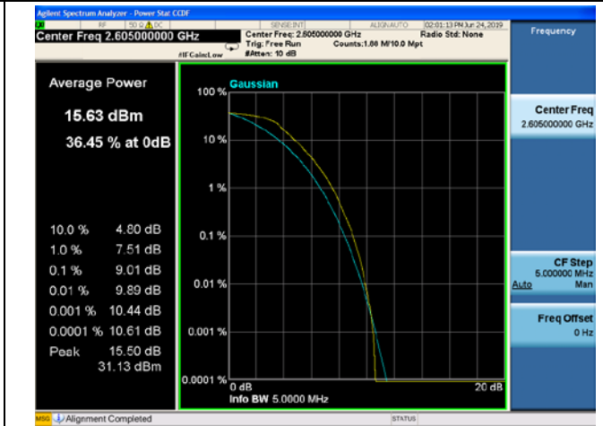
5MHz/64QAM/Mid CH
