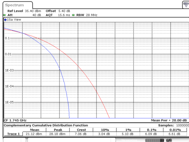
Band66_20MHz_16QAM_132322_100RB#
