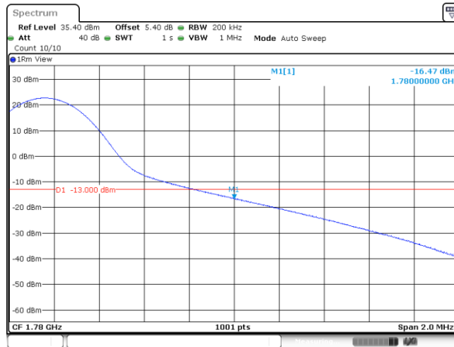
Band66_15MHz_QPSK_132597_75RB#0
