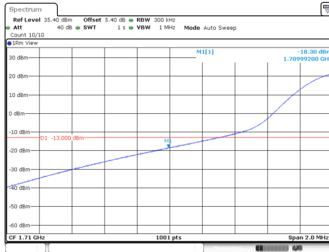
Band66_20MHz_16QAM_132072_100RB#0
