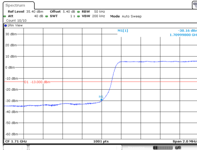
Band66_3MHz_QPSK_131987_15RB#0
