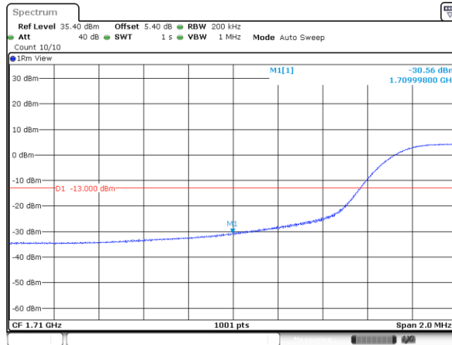
Band66_15MHz_QPSK_132047_75RB#0
