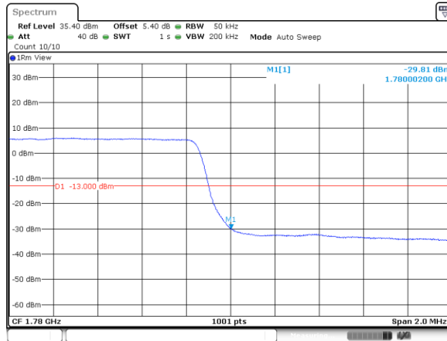
Band66_3MHz_QPSK_132657_15RB#0
