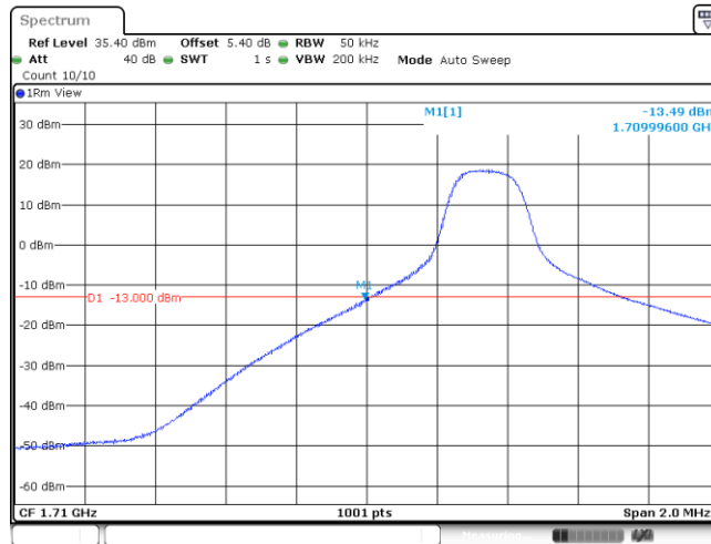
Band66_5MHz_QPSK_131997_25RB#0
