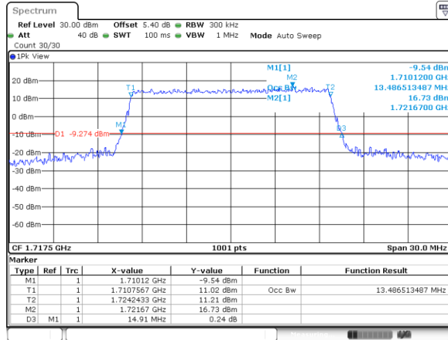
Band66_15MHz_16QAM_132047_75RB#0
