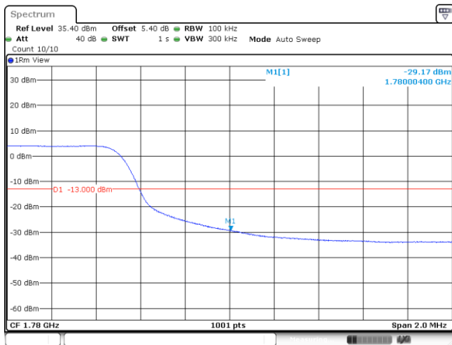
Band66_10MHz_QPSK_132622_50RB#0
