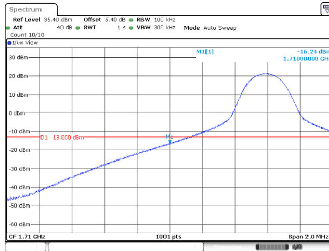
Band66_10MHz_QPSK_132022_50RB#0
