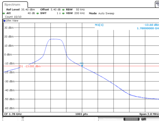
Band66_5MHz_16QAM_132647_25RB#0
