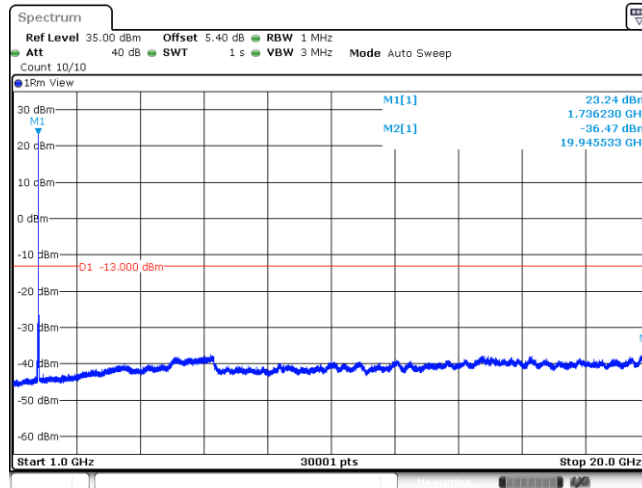
Band66_20MHz_16QAM_132322_1RB#0
