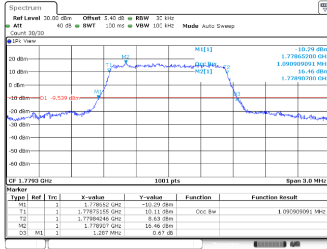
Band66_1.4MHz_16QAM_132665_6RB#0
