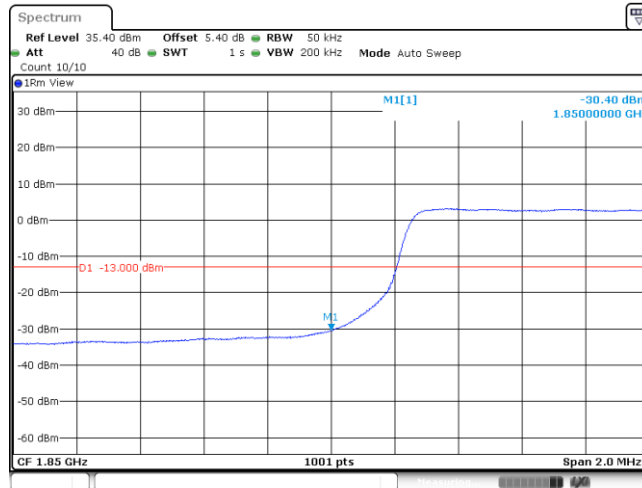
Band2_5MHz_16QAM_18625_25RB#0
