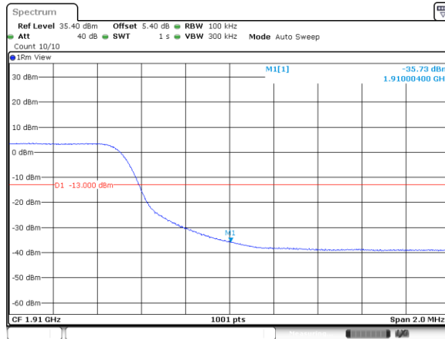
Band2_10MHz_QPSK_19150_50RB#0
