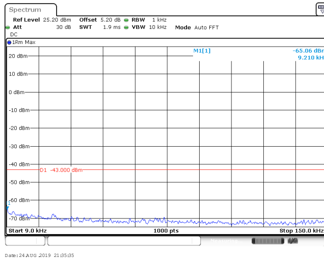
Band IV_1513
