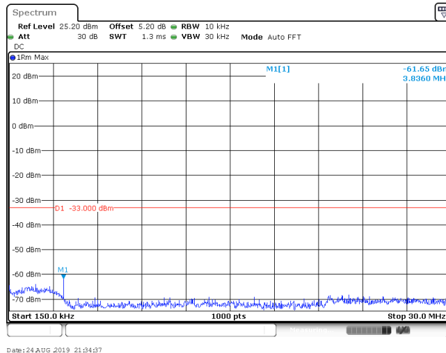
Band IV_1413
