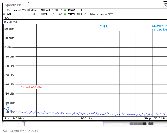
Band IV_1413
