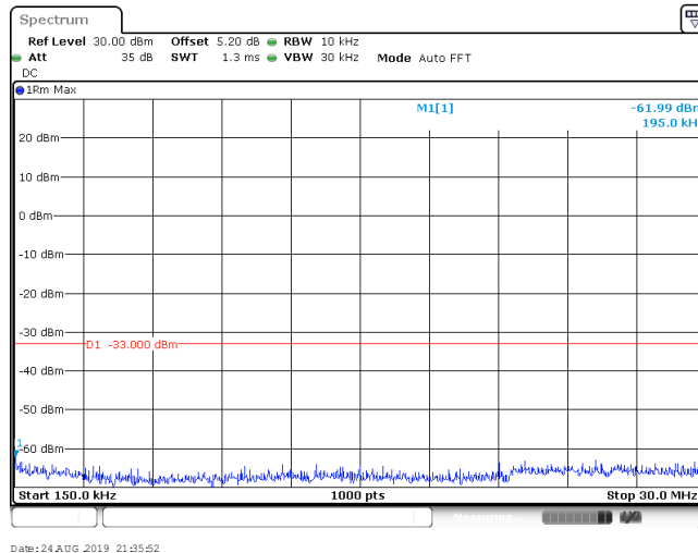
Band IV_1513
