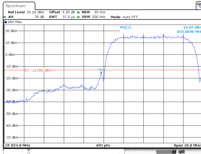
Band V_16QAM_4132
