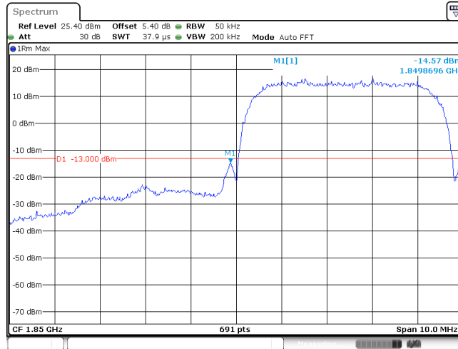
Band II_16QAM_9262
