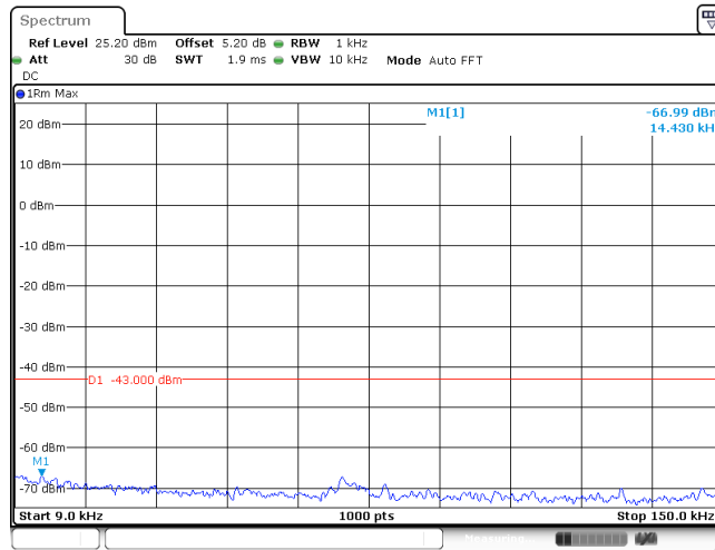
Band V_4233
