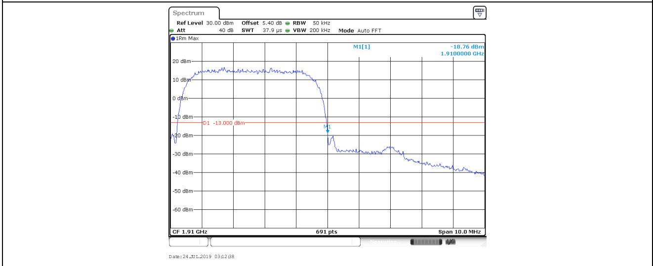
Band II_QPSK_9538
