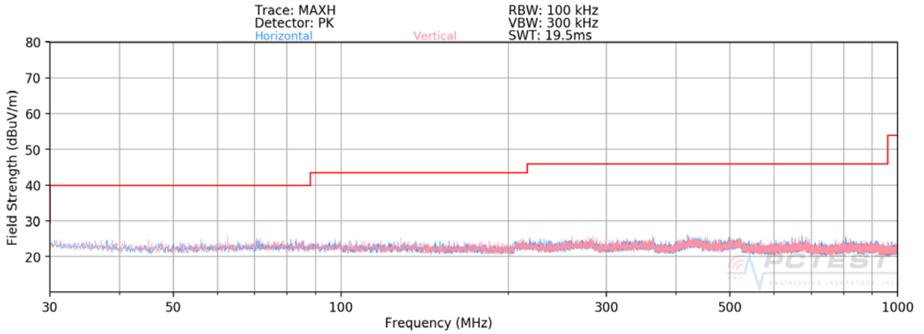
Plot 7-55. Radiated Spurious Plot below 1GHz
