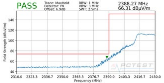
Plot 7-48. Radiated Restricted Lower Band Edge Measurement (Peak)
