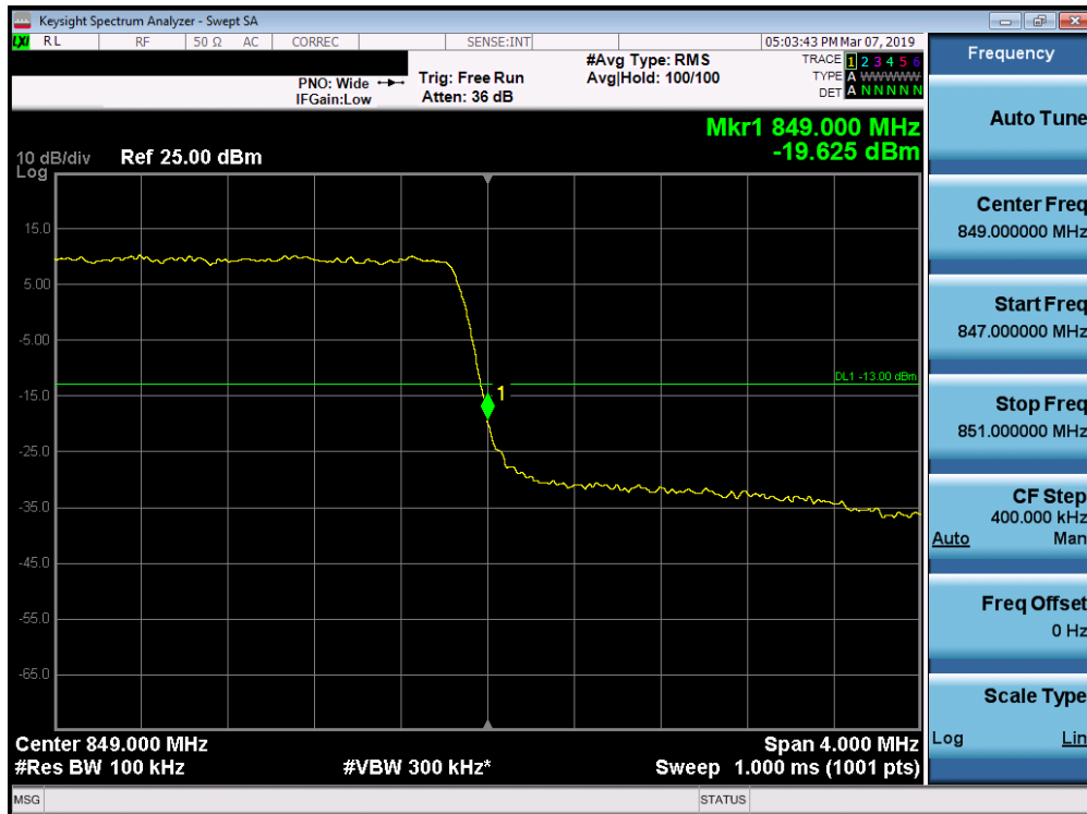
Plot 7-120. Upper Band Edge Plot (Band 5 - 3.0MHz QPSK - Full RB Configuration)
