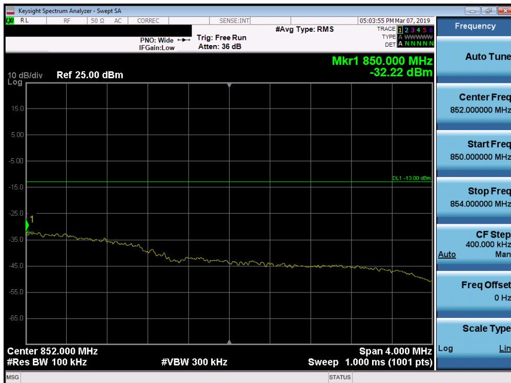
Plot 7-121. Upper Extended Band Edge Plot (Band 5 - 3.0MHz QPSK - Full RB Configuration)
