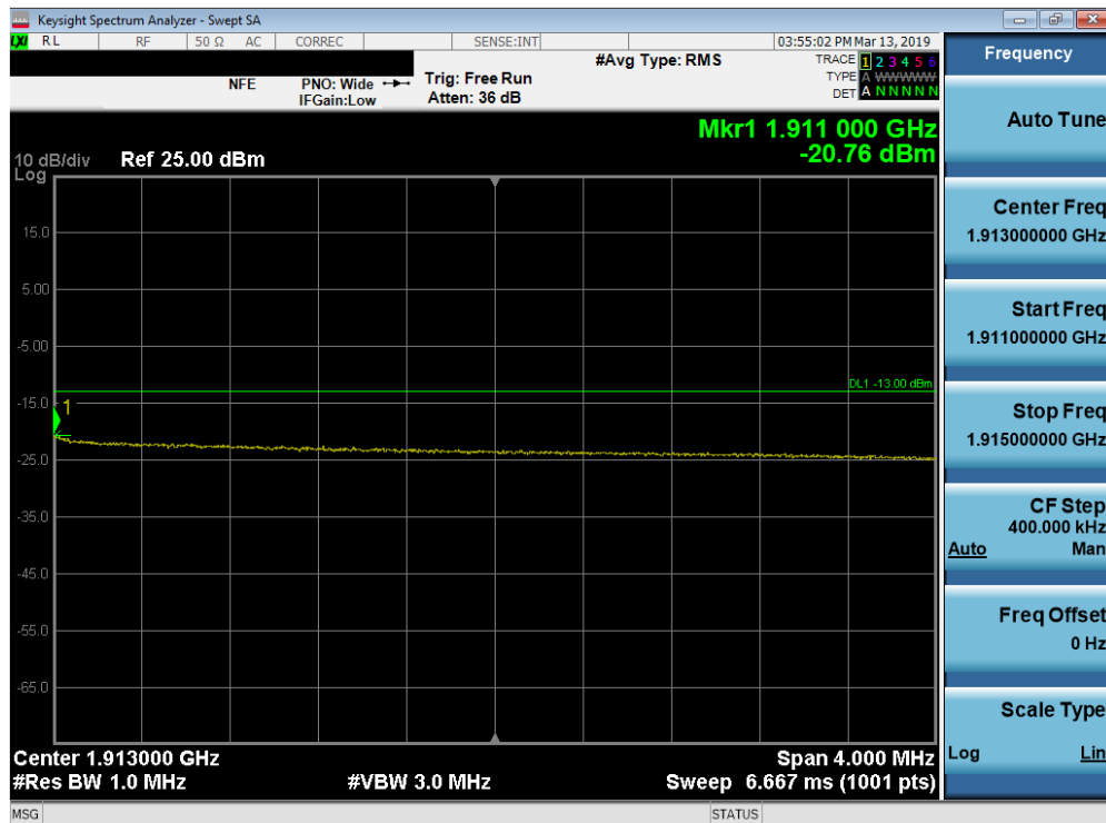
Plot 7-175. Upper Extended Band Edge Plot (Band 2 - 10.0MHz QPSK - Full RB Configuration)
