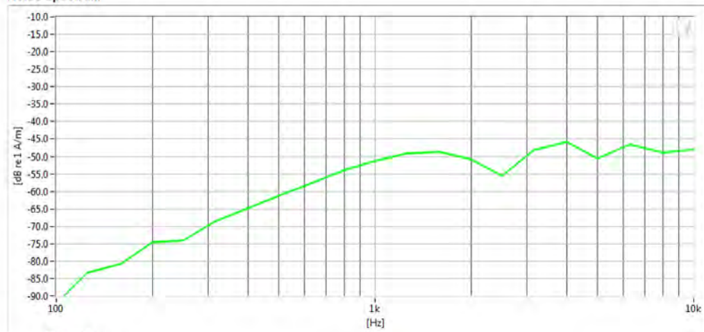
Noise Spectrum
