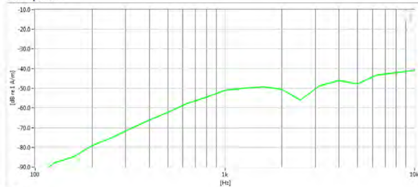
Noise Spectrum
