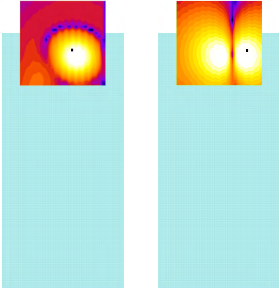
Figure 8-1 CMRS T-Coil Scan Overlay Magnetic Field Distributions
