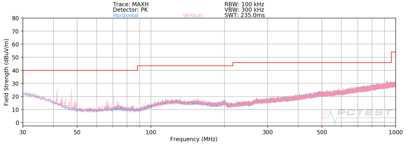
Plot 7-43. Radiated Spurious Plot below 1GHz ANT1
