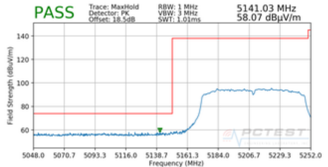
Plot 7-98. Radiated Lower Band Edge Plot (Peak – UNII Band 1)
