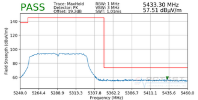
Plot 7-100. Radiated Upper Band Edge Plot (Peak – UNII Band 2A)
