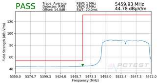
Plot 7-110. Radiated Lower Band Edge Plot (Average – UNII Band 2C)
