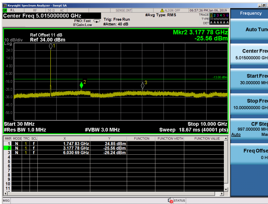
LTE Band 66, 4 / 15MHz / QPSK - RB Size/Offset (36/18) – Mid Channel
