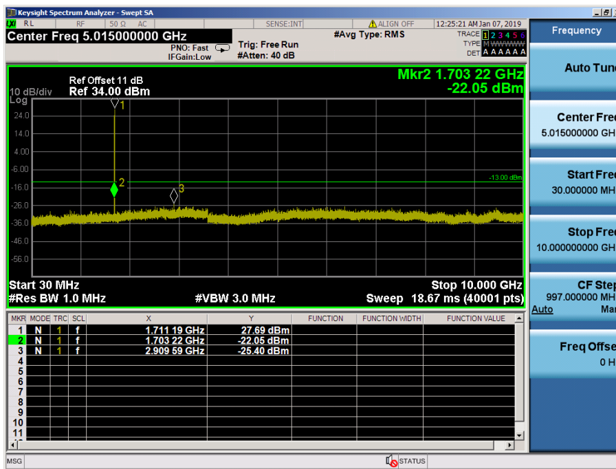
LTE Band 66, 4 / 1.4MHz / 64QAM - RB Size/Offset (6/0) – Low Channel
