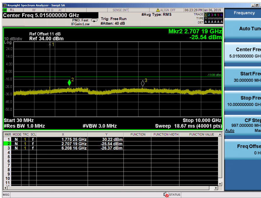
LTE Band 66, 4 / 10MHz / QPSK - RB Size/Offset (1/25) – High Channel
