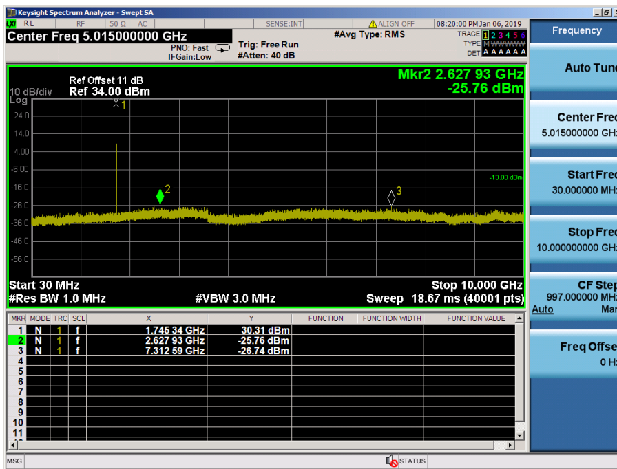
LTE Band 66, 4 / 1.4MHz / 16QAM - RB Size/Offset (3/2) – Mid Channel
