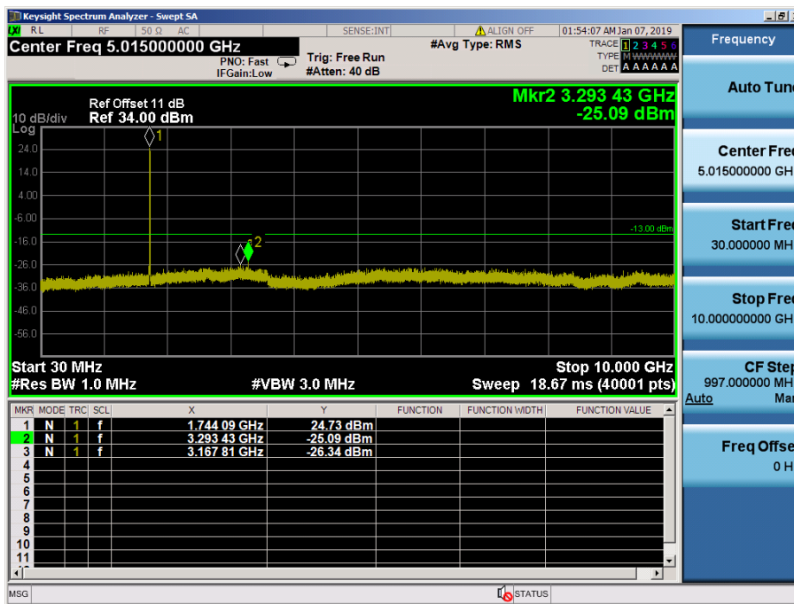
LTE Band 66, 4 / 5MHz / 64QAM - RB Size/Offset (25/0) – Mid Channel
