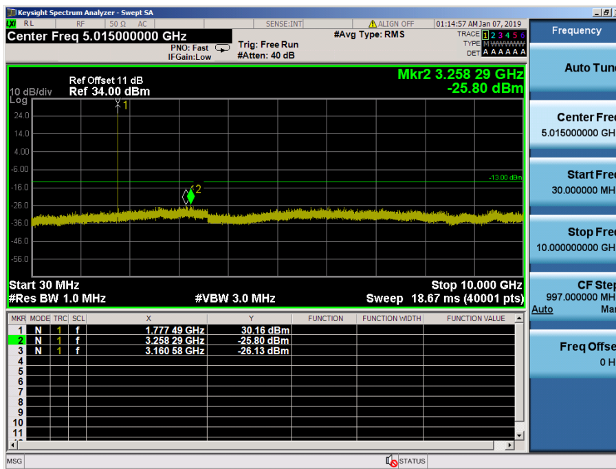
LTE Band 66, 4 / 3MHz / 64QAM - RB Size/Offset (1/0) – High Channel
