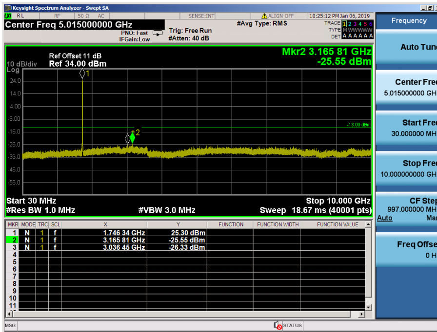
LTE Band 66, 4 / 10MHz / 16QAM - RB Size/Offset (25/12) – Mid Channel
