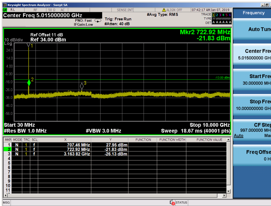
LTE Band 12 / 3MHz / 16QAM - RB Size/Offset (15/0) – Mid Channel
