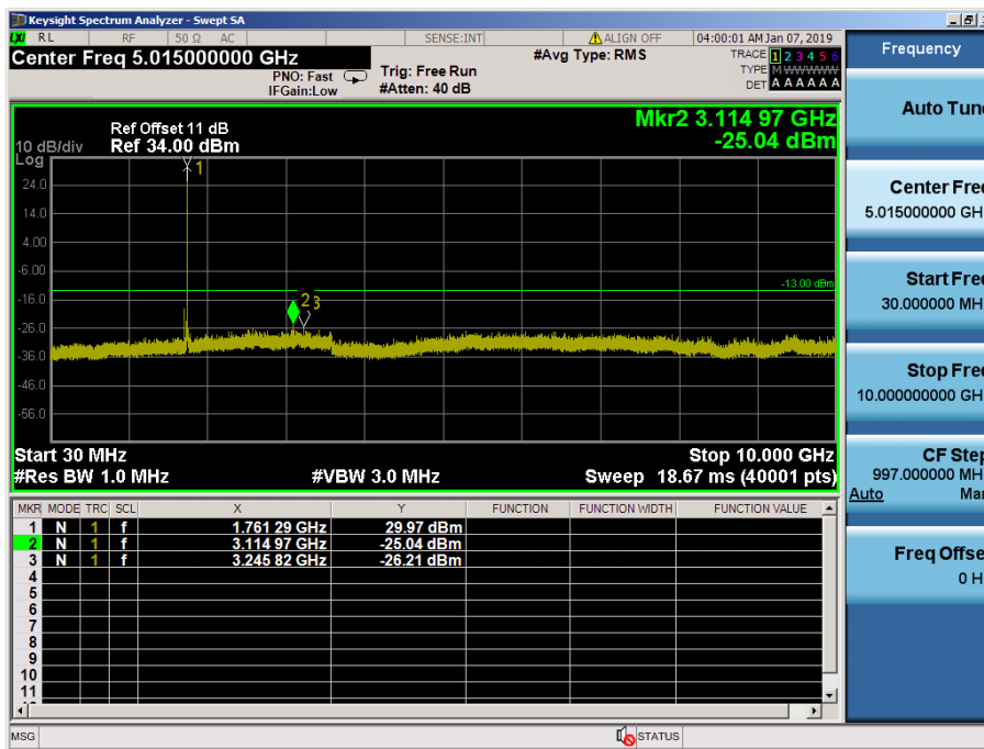
LTE Band 66, 4 / 20MHz / 64QAM - RB Size/Offset (1/0) – High Channel
