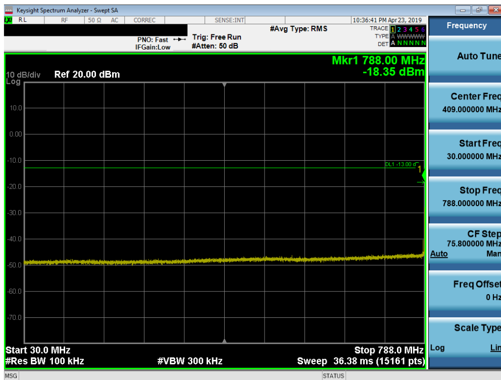
Plot 7-5. Conducted Spurious Plot (LTE Band 14, 10.0 MHz QPSK – RB Size 1, RB Offset 0 – Mid Channel)
