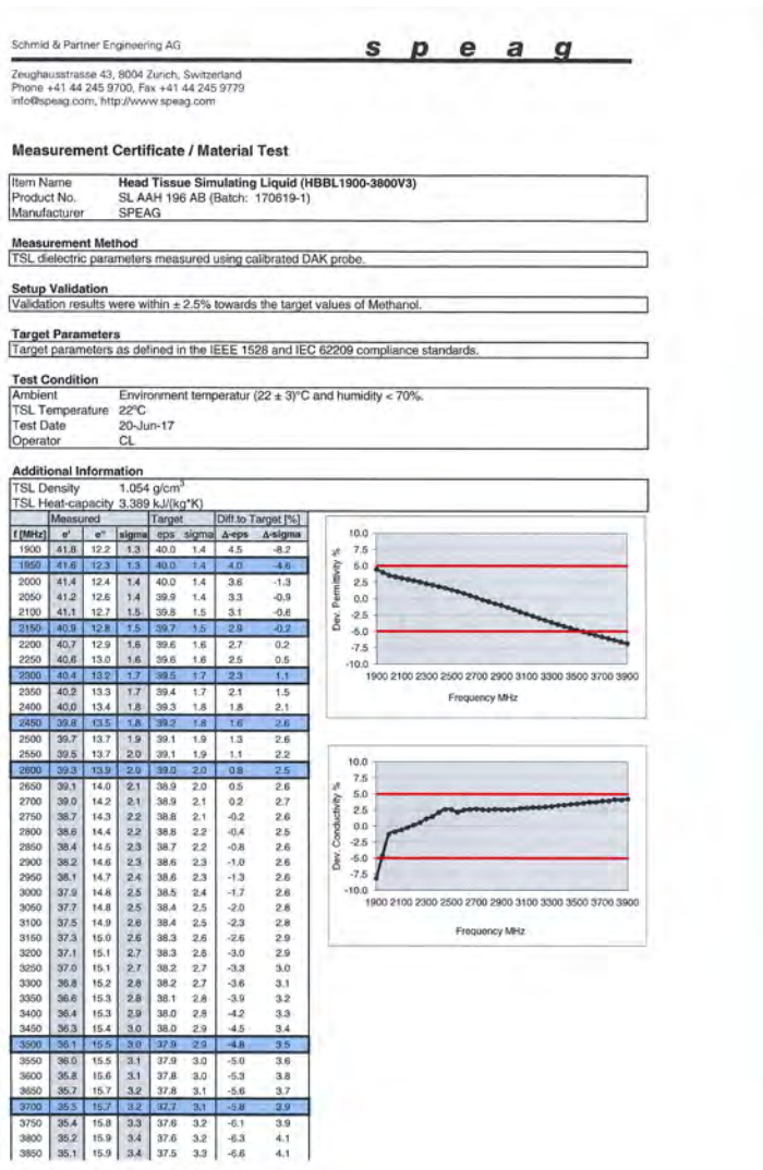
Figure D-5 2.45 GHz Head Tissue Equivalent Matter
