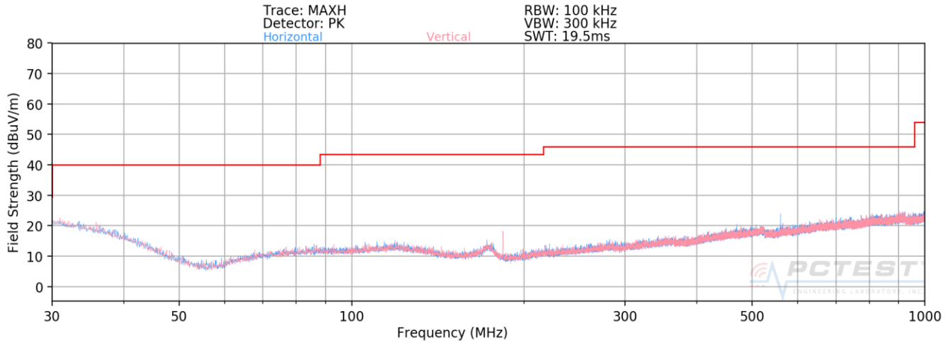
Plot 7-47. Radiated Spurious Plot below 1GHz
