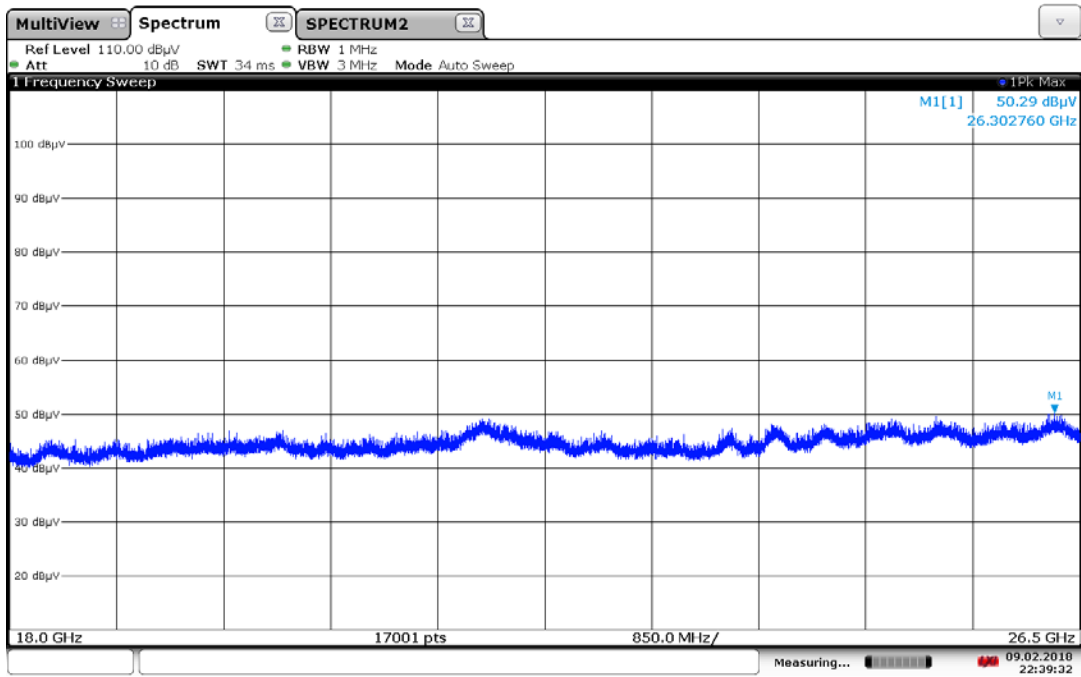
Plot 7-38. Radiated Spurious Plot above 18GHz, Ant. Pol. V
