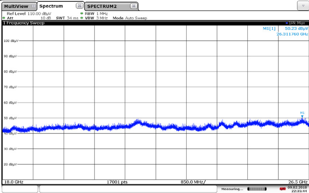
Plot 7-37. Radiated Spurious Plot above 18GHz, Ant. Pol. H
