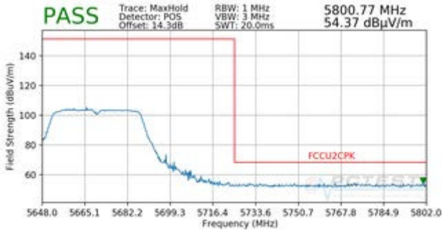
Plot 7-102. Radiated Upper Band Edge Plot (Peak – UNII Band 2C)
