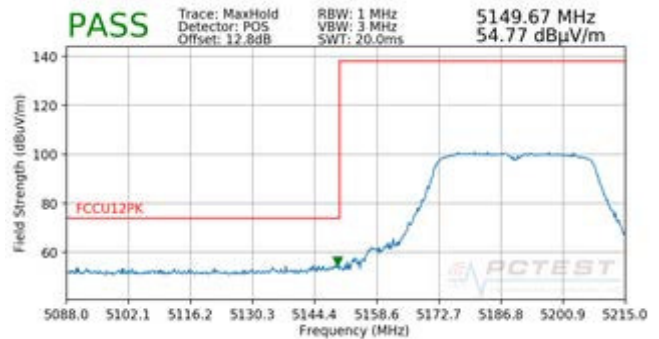
Plot 7-97. Radiated Lower Band Edge Plot (Peak – UNII Band 1)
