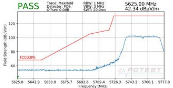
Plot 7-103. Radiated Lower Band Edge Plot (Peak – UNII Band 3)
