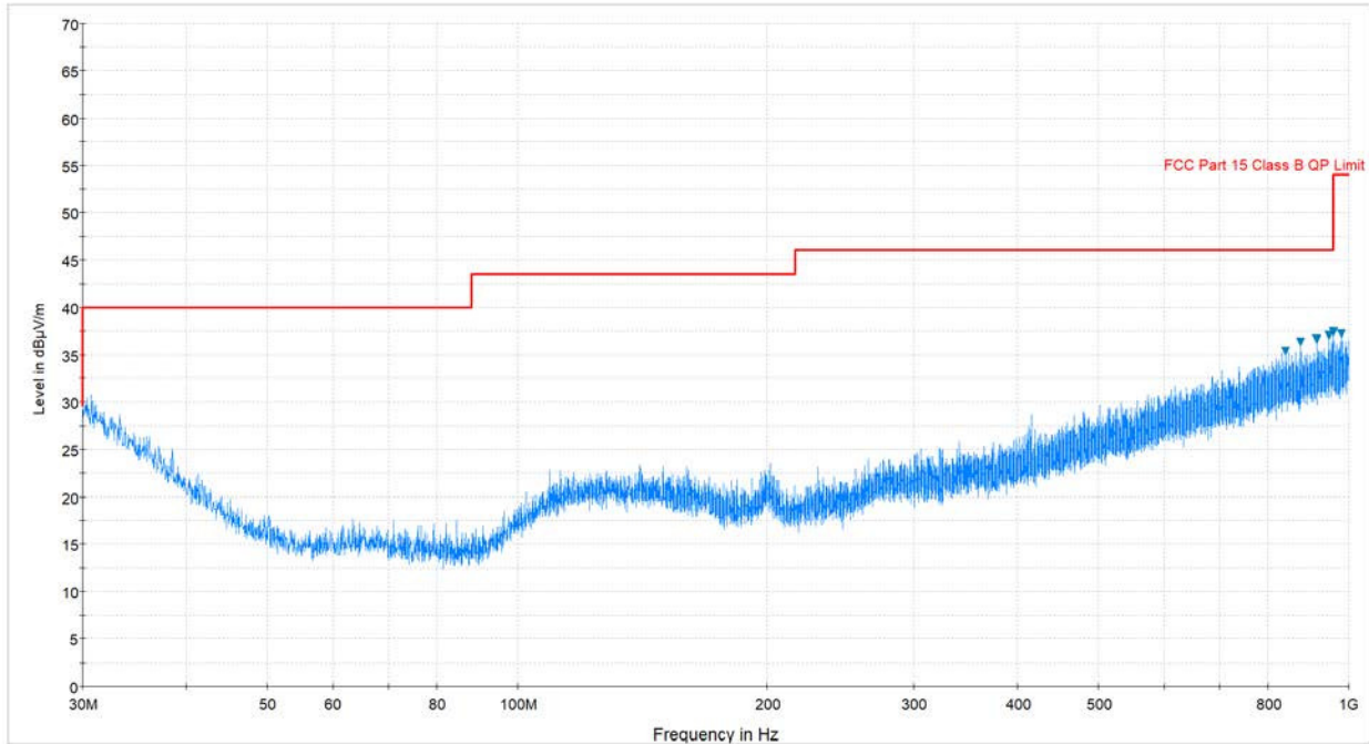
Plot 7-113. Radiated Spurious Plot below 1GHz (802.11a – U3 Ch. 157, Ant. Pol. H)
