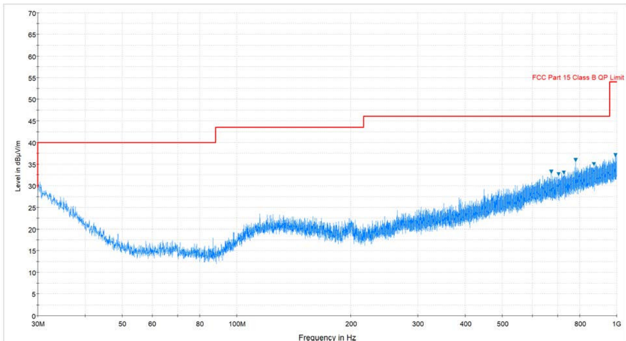
Plot 7-114. Radiated Spurious Plot below 1GHz (802.11a – U3 Ch. 157, Ant. Pol. V)
