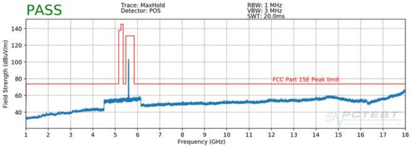
Plot 7-81. Radiated Spurious Plot above 1GHz (802.11a – U2C Ch. 120, Ant. Pol. H)
