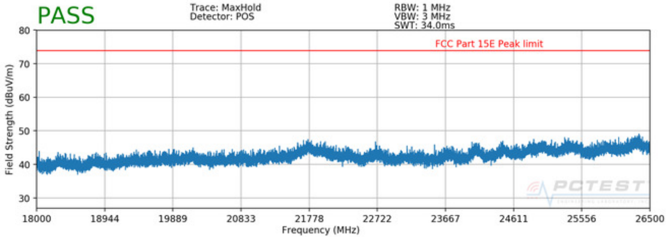
Plot 7-85. Radiated Spurious Plot 18GHz - 26.5GHz (802.11a)
