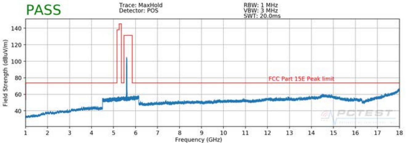
Plot 7-82. Radiated Spurious Plot above 1GHz (802.11a – U2C Ch. 120, Ant. Pol. V)
