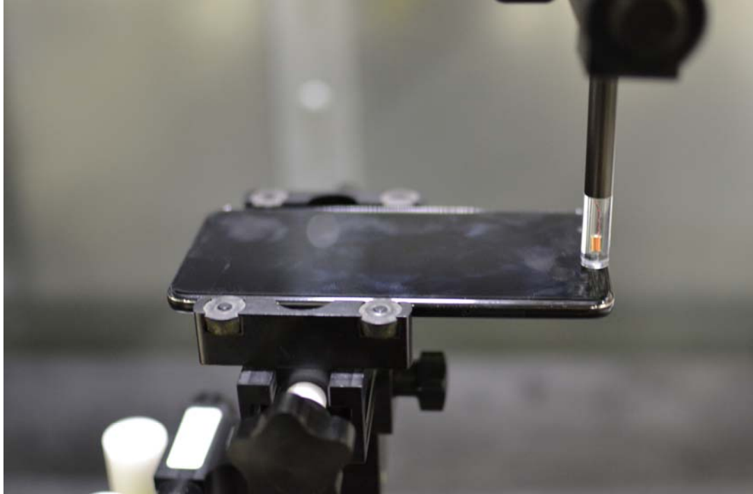
Figure 16-1 Test Setup for Wireless Device
