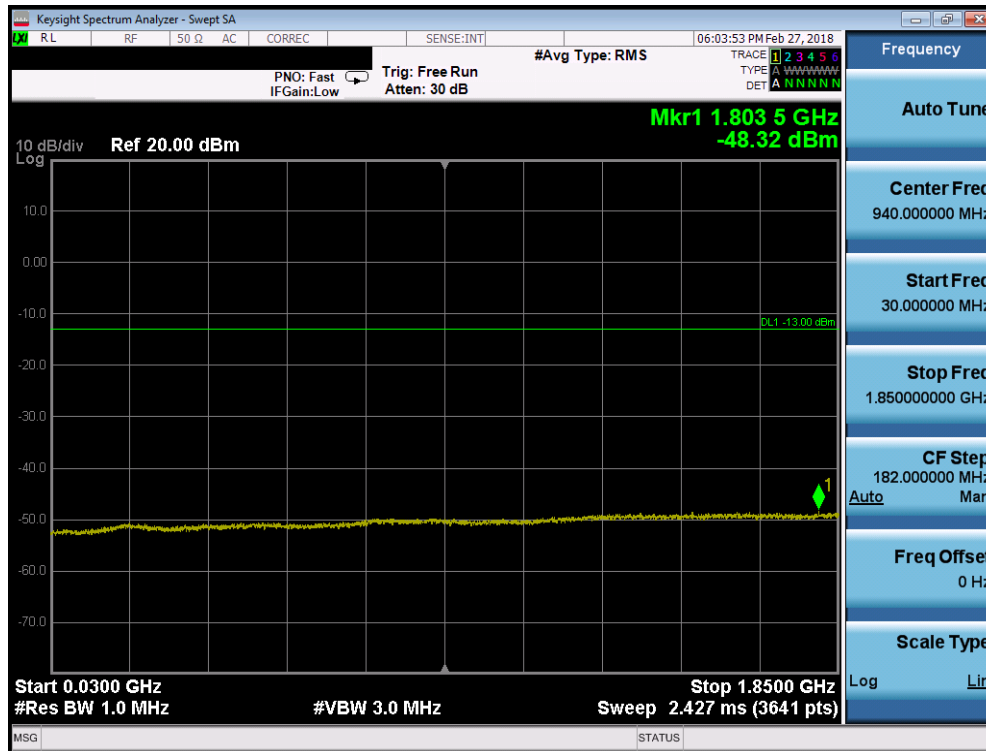
Plot 7-50. Conducted Spurious Plot (PCS WCDMA Mode - High Channel)
