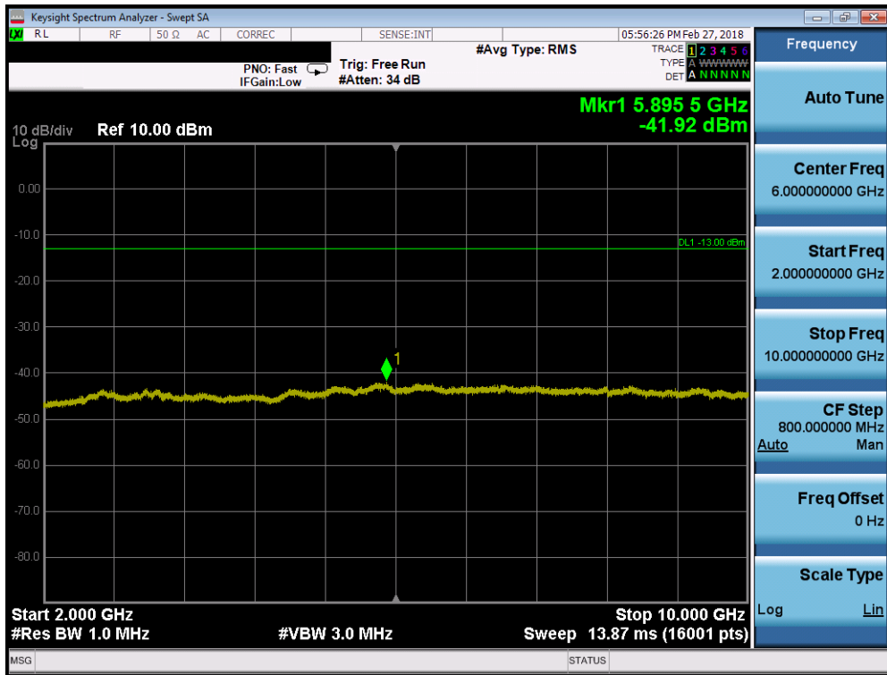
Plot 7-28. Conducted Spurious Plot (Cellular WCDMA Mode - Low Channel)
