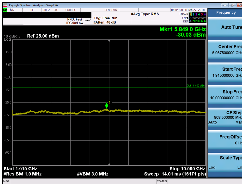
Plot 7-51. Conducted Spurious Plot (PCS WCDMA Mode - High Channel)
