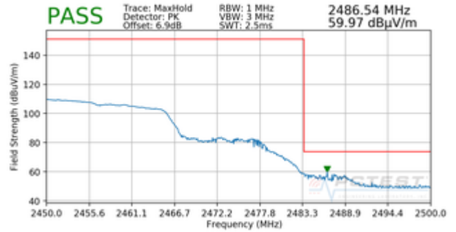
Plot 7-10. Radiated Restricted Upper Band Edge Measurement (Peak)
