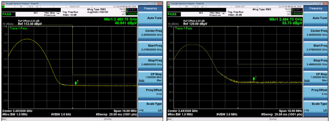
Plot 7-18. Radiated Restricted Upper Band Edge Measurement (Average & Peak)
