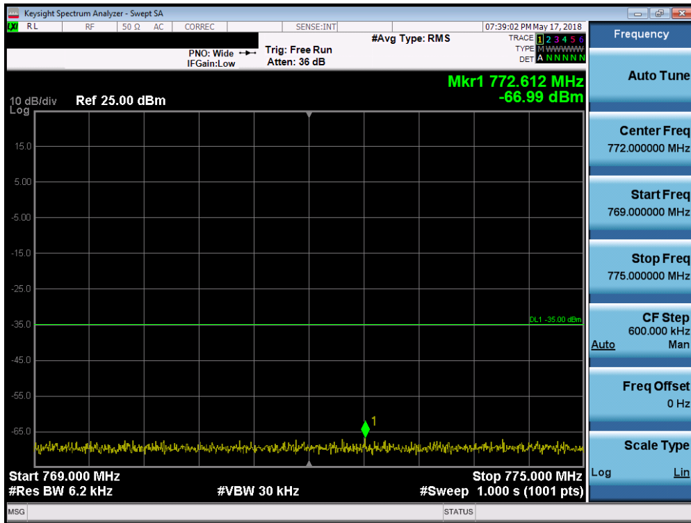
Plot 7-9. Lower Emission Mask Plot (LTE B14 5MHz QPSK – RB Size 25)
