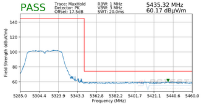
Plot 7-83. Radiated Upper Band Edge Plot (Peak – UNII Band 2A)
