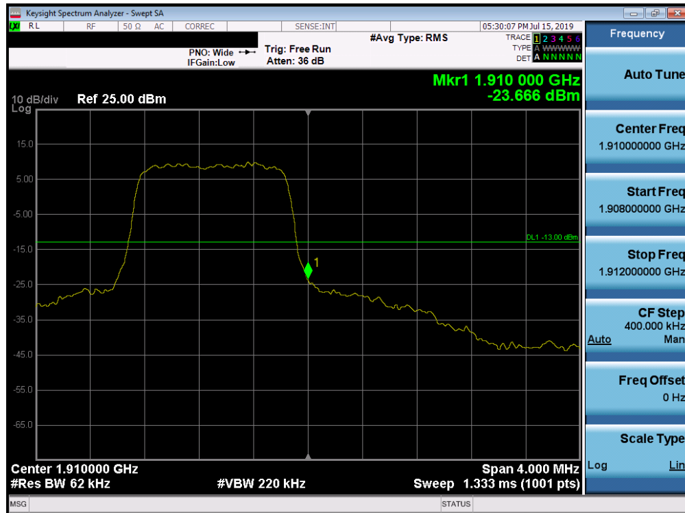
Plot 7-235. Upper Band Edge Plot (Band 2 - 1.4MHz QPSK - Full RB Configuration)
