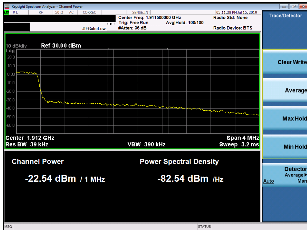
Plot 7-242. Upper Extended Band Edge Plot (Band 2 - 3.0MHz QPSK - Full RB Configuration)
