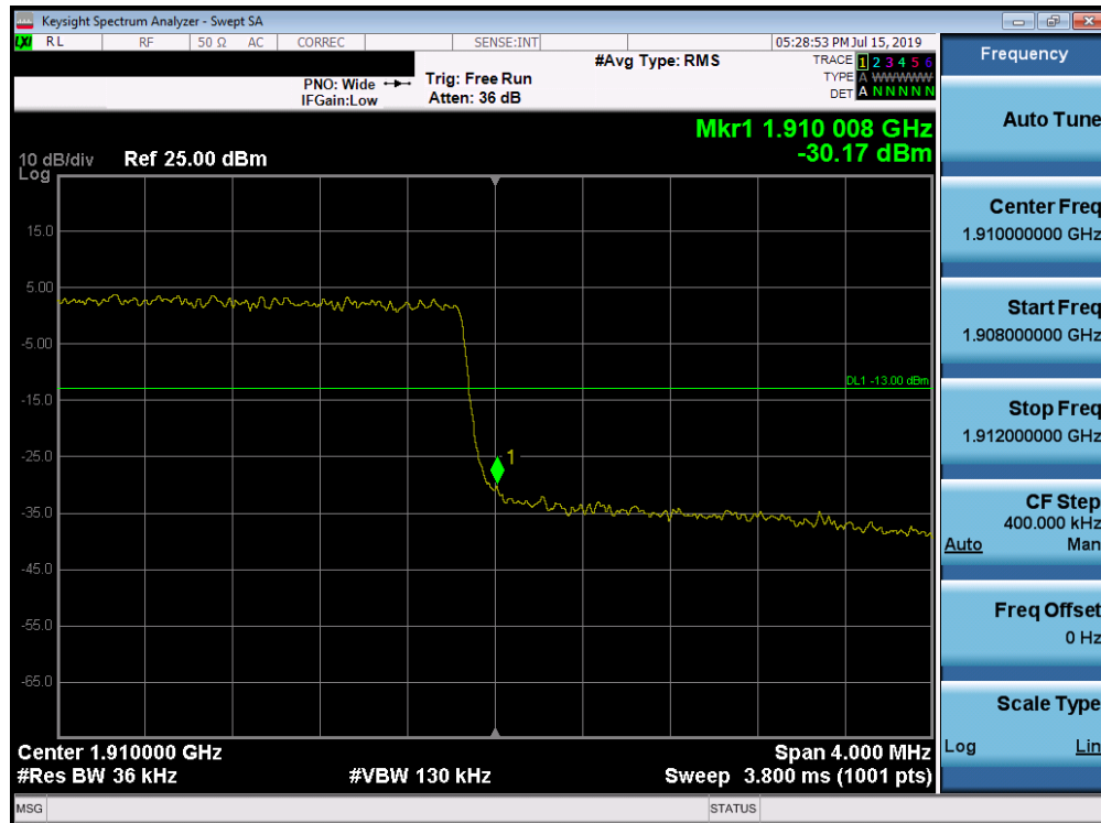
Plot 7-241. Upper Band Edge Plot (Band 2 - 3.0MHz QPSK - Full RB Configuration)
