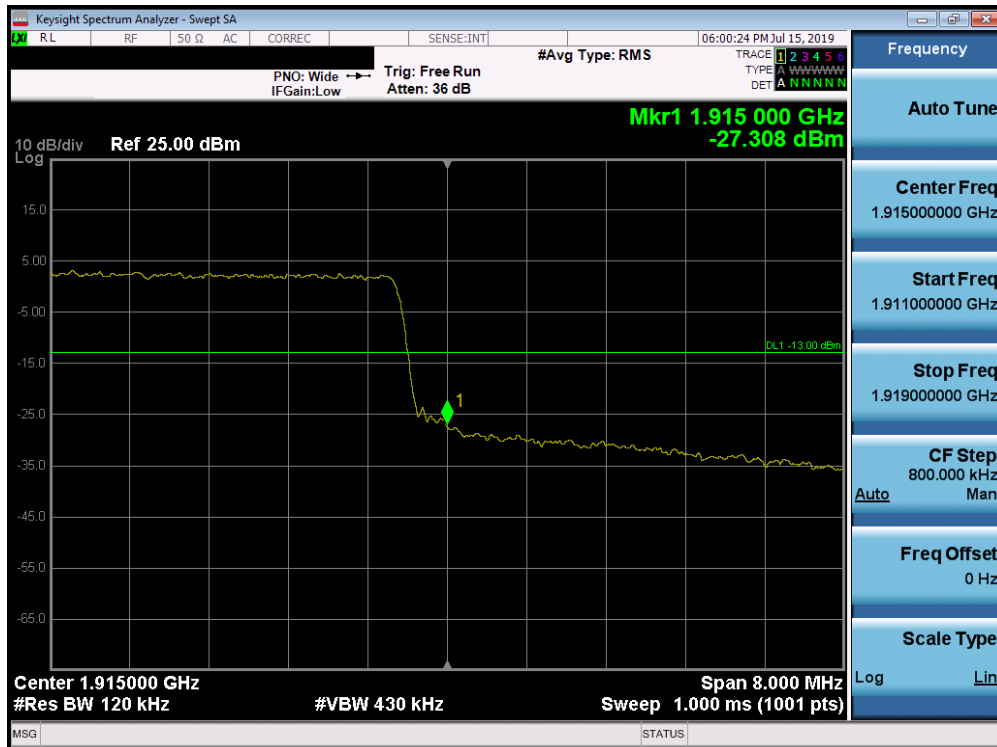
Plot 7-255. Upper Band Edge Plot (Band 25 - 10.0MHz QPSK - Full RB Configuration)
