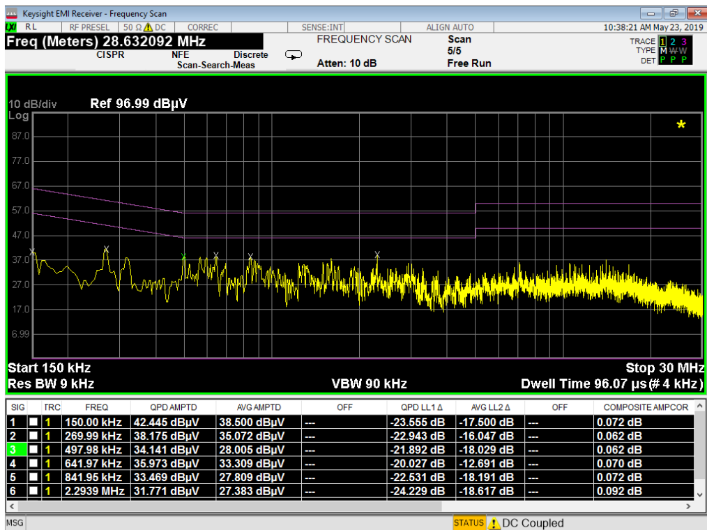
Plot 7-22. Line Conducted Plot with Bluetooth LE (N)
