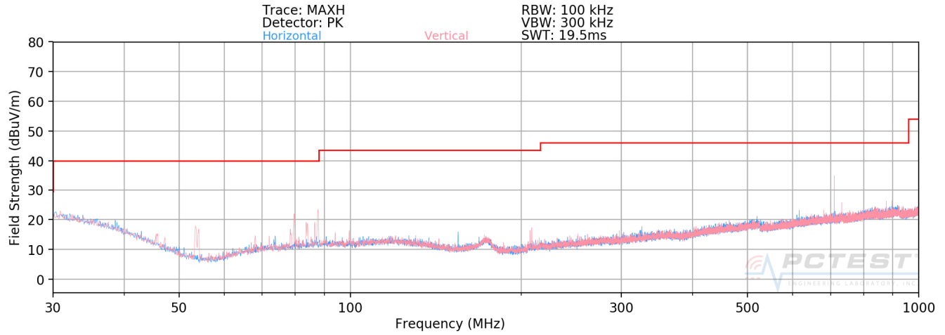
Plot 7-20. Radiated Spurious Plot below 1GHz
