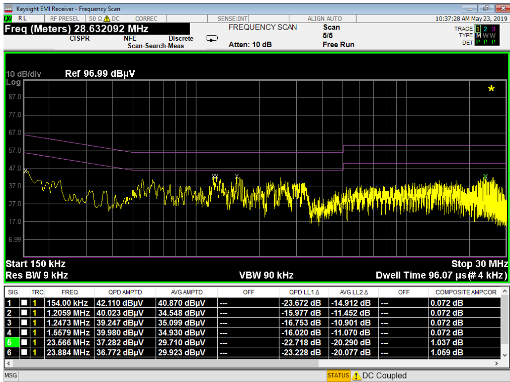
Plot 7-21. Line Conducted Plot with Bluetooth LE (L1)
