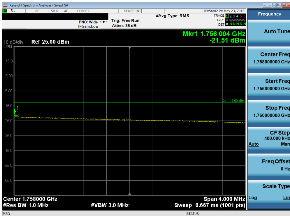
Plot 7-109. Upper Extended Band Edge Plot (Band 4 - 10.0MHz QPSK - Full RB Configuration)
