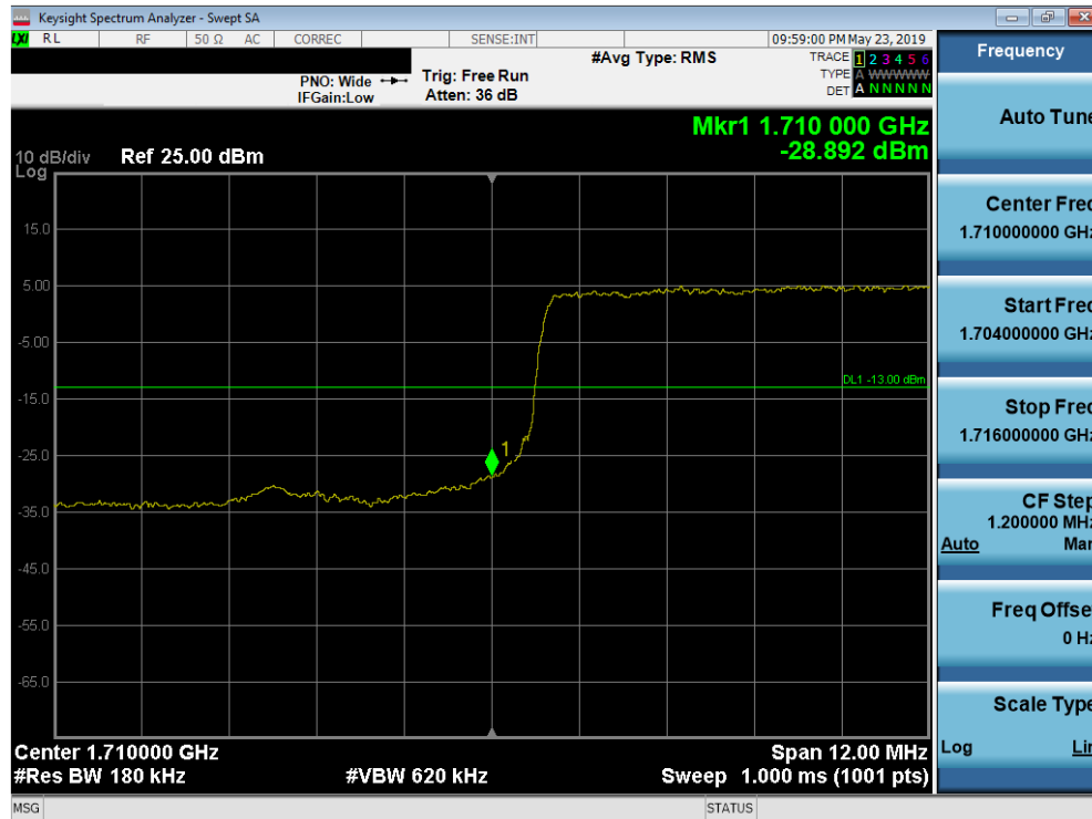
Plot 7-114. Lower Band Edge Plot (Band 4 - 20.0MHz QPSK - Full RB Configuration)
