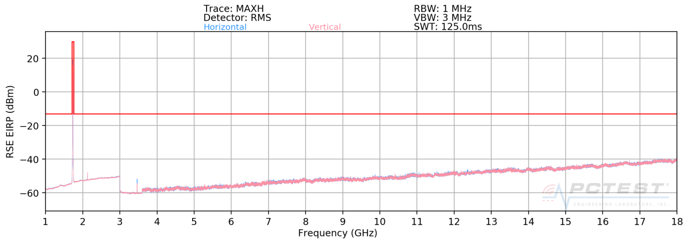
Plot 7-72. Radiated Spurious Plot above 1GHz (AWS WCDMA Mode)
