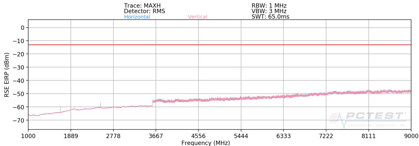
Plot 7-70. Radiated Spurious Plot above 1GHz (Cellular GPRS Mode)
