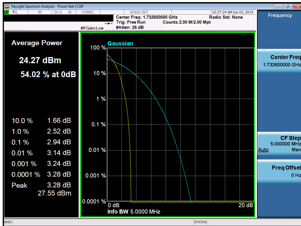
Plot 7-68. Peak-Average Ratio Plot (AWS WCDMA Mode)
