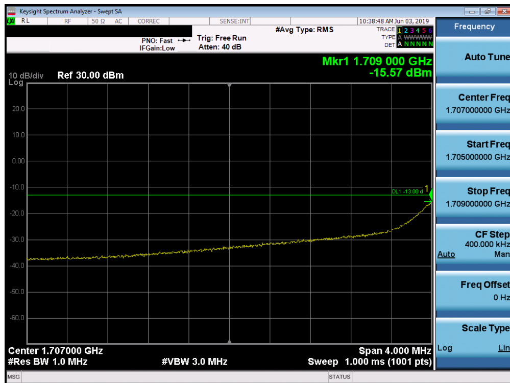
Plot 7-59. 4MHz Span Plot (AWS WCDMA Mode - Low Channel)
