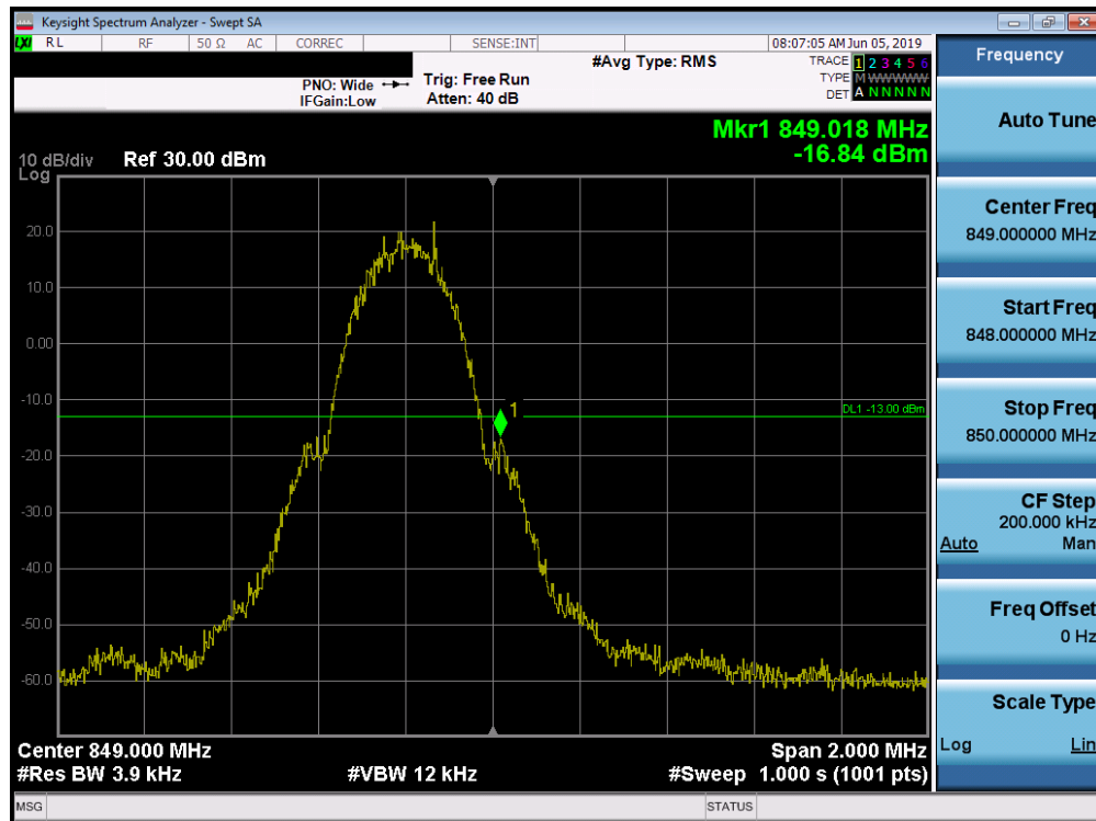
Plot 7-51. Band Edge Plot (Cellular GPRS Mode - High Channel)
