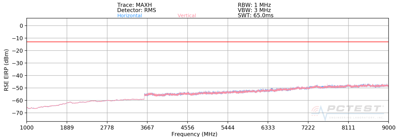
Plot 7-71. Radiated Spurious Plot above 1GHz (Cellular WCDMA Mode)
