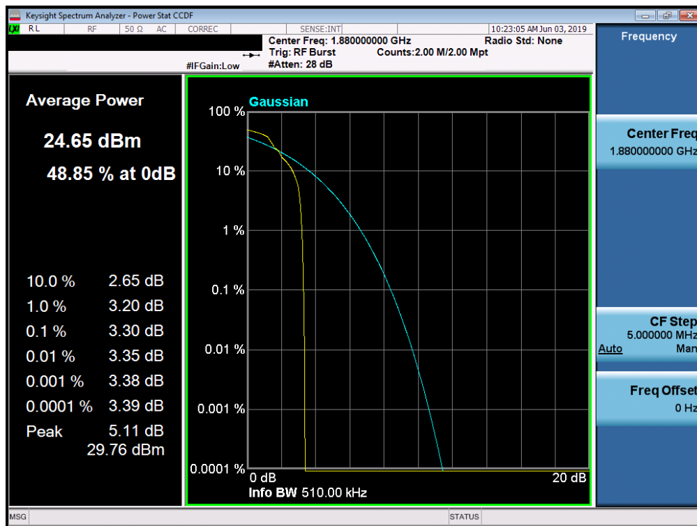
Plot 7-67. Peak-Average Ratio Plot (PCS GPRS EDGE Mode)
