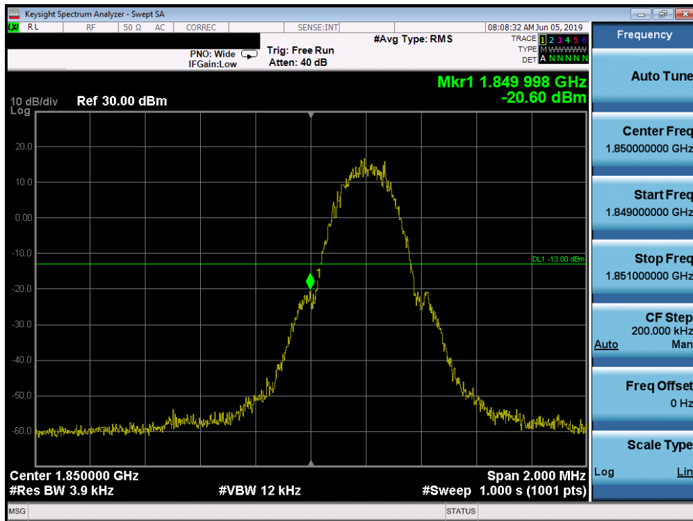
Plot 7-52. Band Edge Plot (PCS GPRS Mode - Low Channel)
