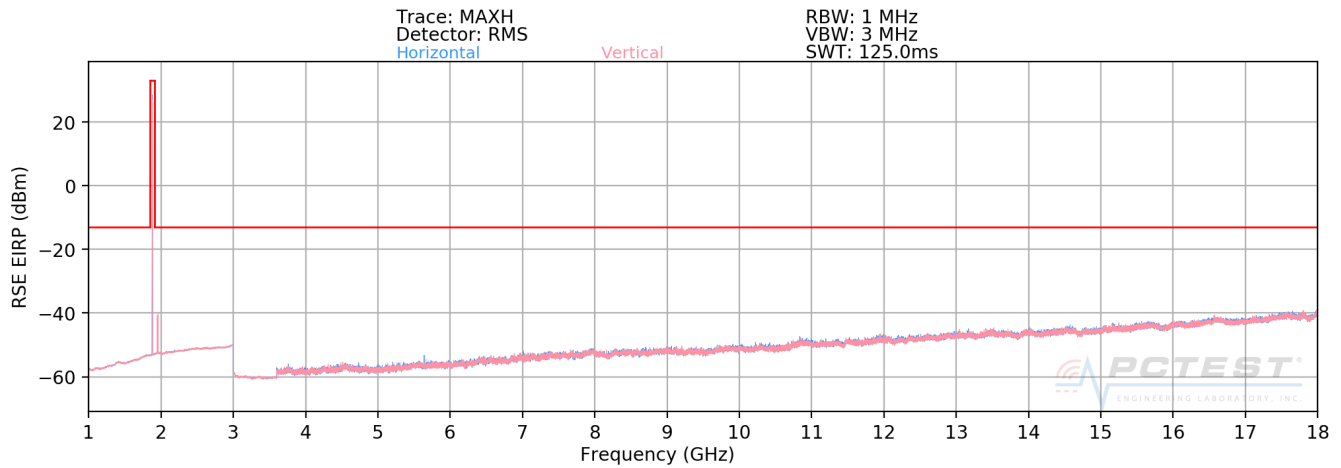
Plot 7-73. Radiated Spurious Plot above 1GHz (PCS GPRS Mode)
