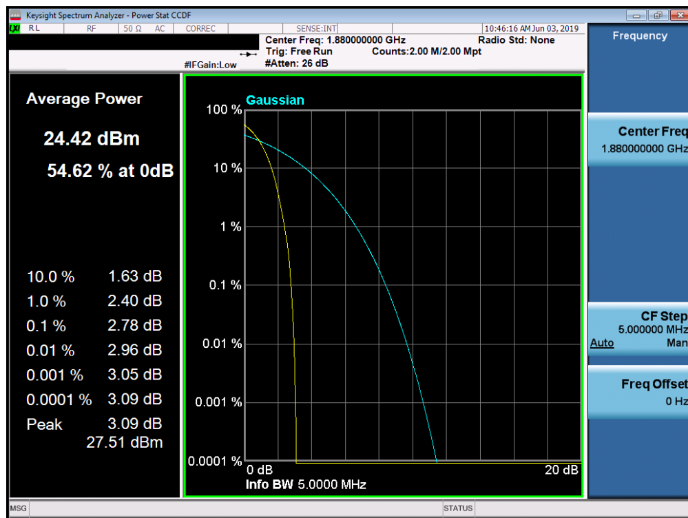
Plot 7-69. Peak-Average Ratio Plot (PCS WCDMA Mode)
