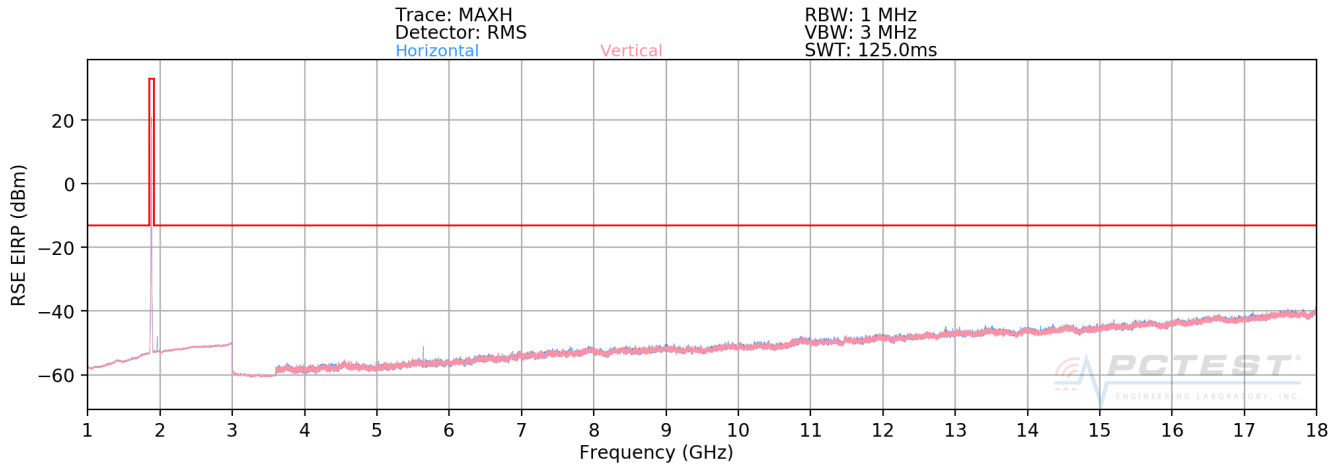
Plot 7-74. Radiated Spurious Plot above 1GHz (PCS WCDMA Mode)
