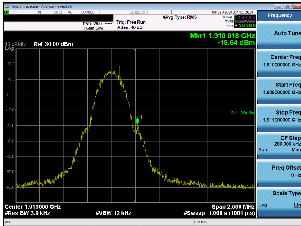
Plot 7-54. Band Edge Plot (PCS GPRS Mode - High Channel)
