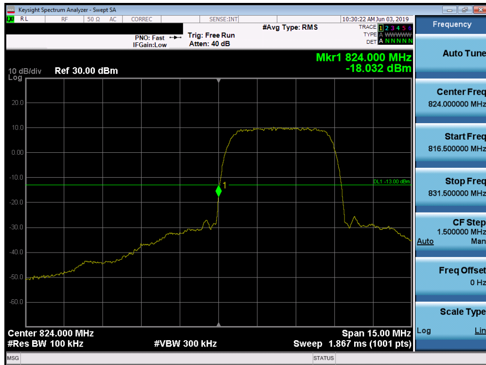
Plot 7-56. Band Edge Plot (Cellular WCDMA Mode - Low Channel)
