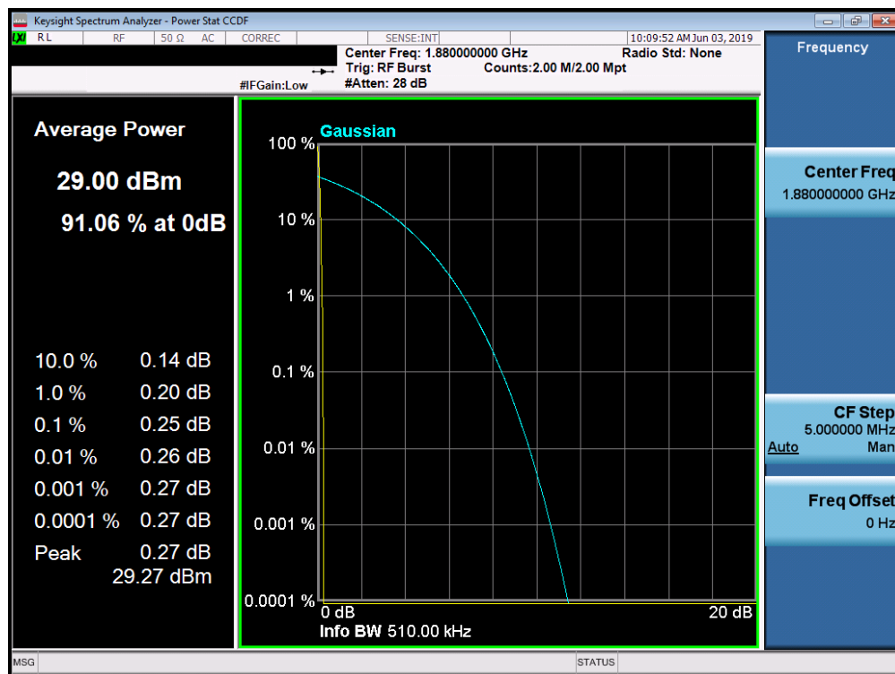
Plot 7-66. Peak-Average Ratio Plot (PCS GPRS Mode)
