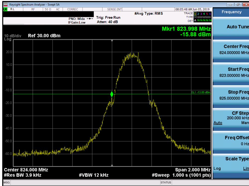
Plot 7-50. Band Edge Plot (Cellular GPRS Mode - Low Channel)
