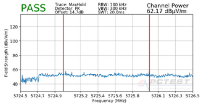
Plot 7-79. Radiated Upper Band Edge Plot (Peak – UNII Band 2C)
