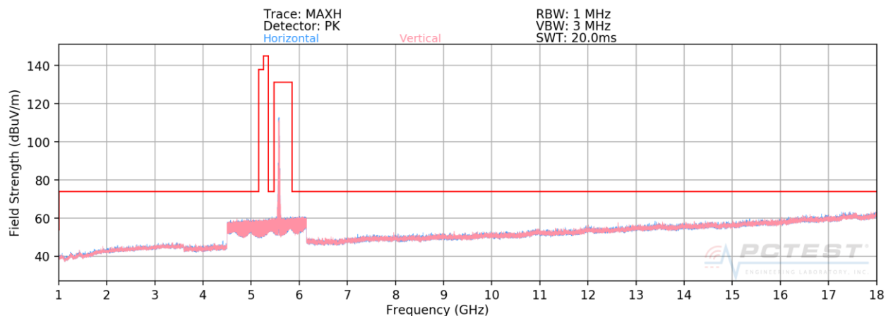
Plot 7-69. Radiated Spurious Plot above 1GHz (802.11a – U2C Ch. 116)
