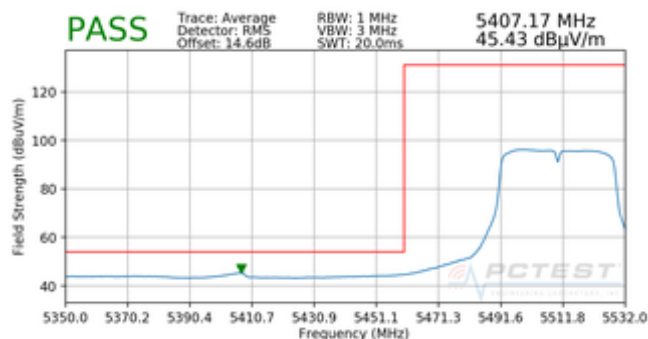
Plot 7-86. Radiated Lower Band Edge Plot (Average – UNII Band 2C)
