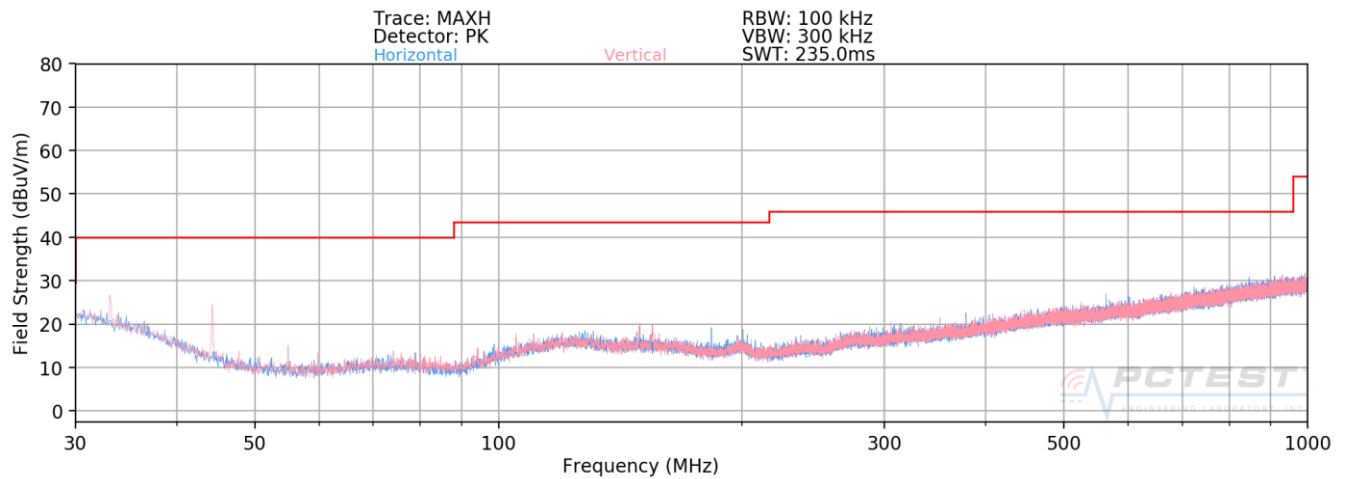
Plot 7-91. Radiated Spurious Plot below 1GHz (802.11a – U3 Ch. 157)
