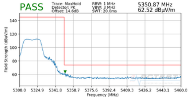
Plot 7-76. Radiated Upper Band Edge Plot (Peak – UNII Band 2A)
