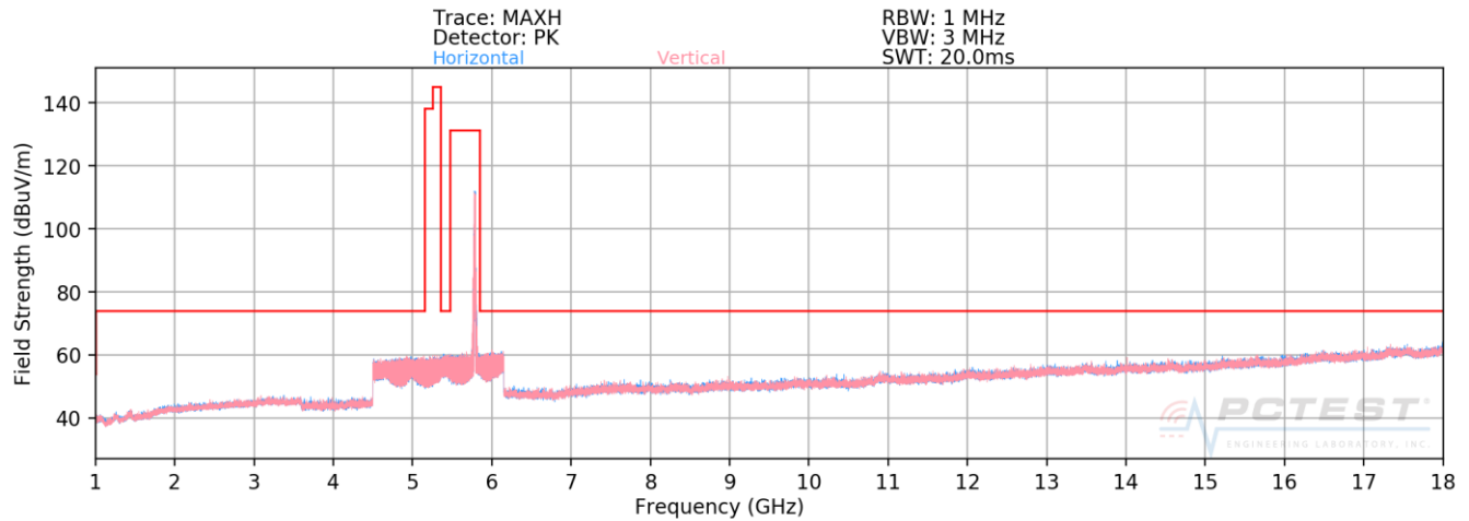
Plot 7-70. Radiated Spurious Plot above 1GHz (802.11a – U3 Ch. 157)
