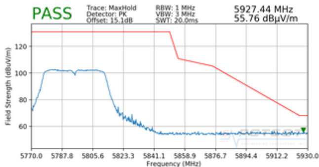
Plot 7-90. Radiated Upper Band Edge Plot (Peak – UNII Band 3)
