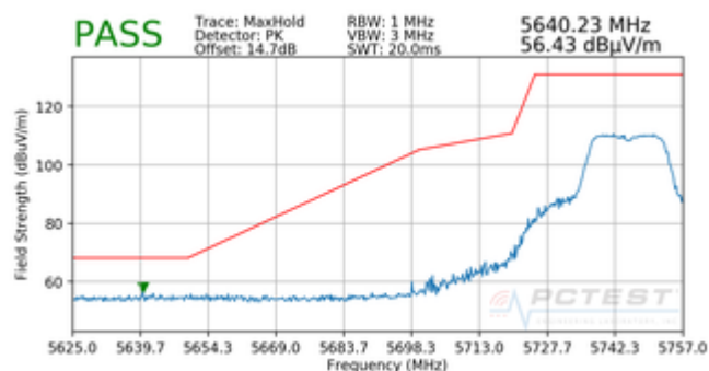
Plot 7-80. Radiated Lower Band Edge Plot (Peak – UNII Band 3)
