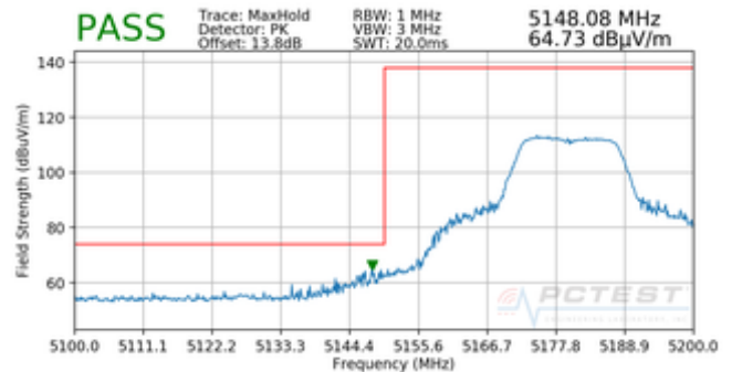
Plot 7-74. Radiated Lower Band Edge Plot (Peak – UNII Band 1)
