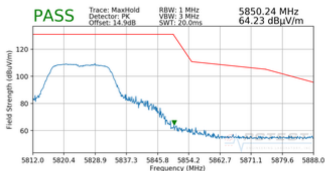
Plot 7-81. Radiated Upper Band Edge Plot (Peak – UNII Band 3)
