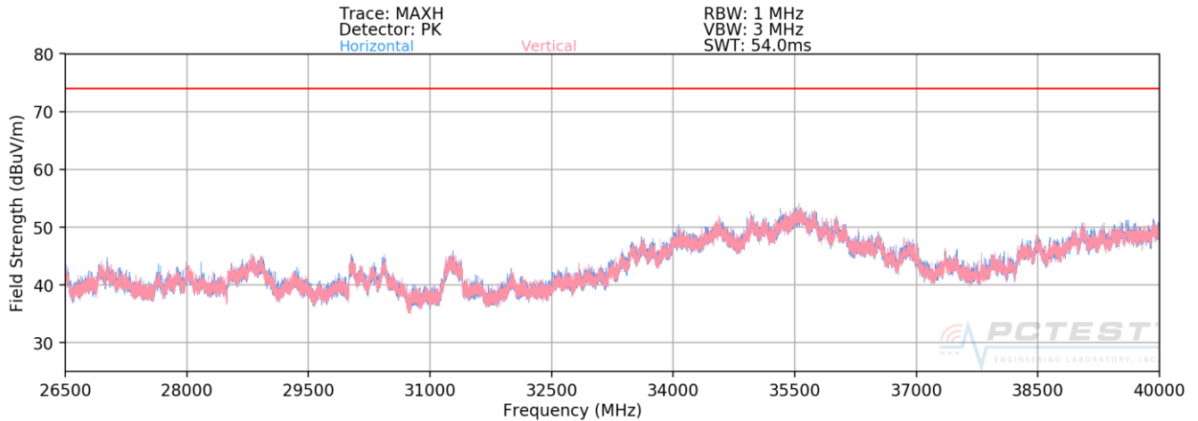
Plot 7-72. Radiated Spurious Plot 26.5GHz - 40GHz (802.11a)
