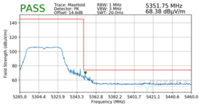
Plot 7-85. Radiated Upper Band Edge Plot (Peak – UNII Band 2A)
