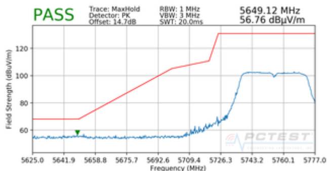
Plot 7-89. Radiated Lower Band Edge Plot (Peak – UNII Band 3)
