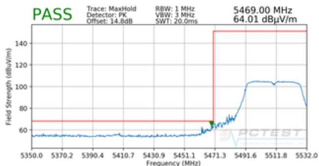
Plot 7-87. Radiated Lower Band Edge Plot (Peak – UNII Band 2C)
