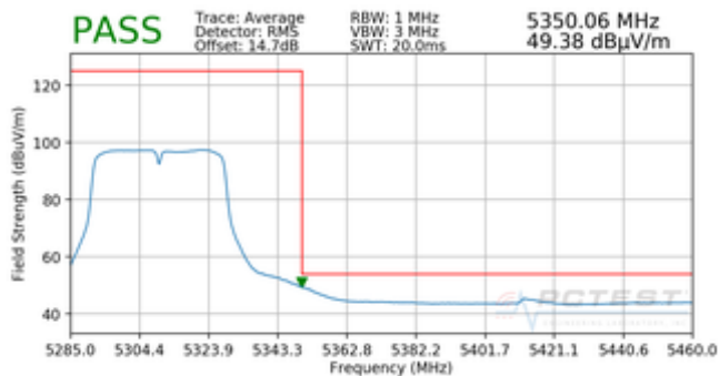
Plot 7-84. Radiated Upper Band Edge Plot (Average – UNII Band 2A)
