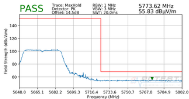
Plot 7-88. Radiated Upper Band Edge Plot (Peak – UNII Band 2C)
