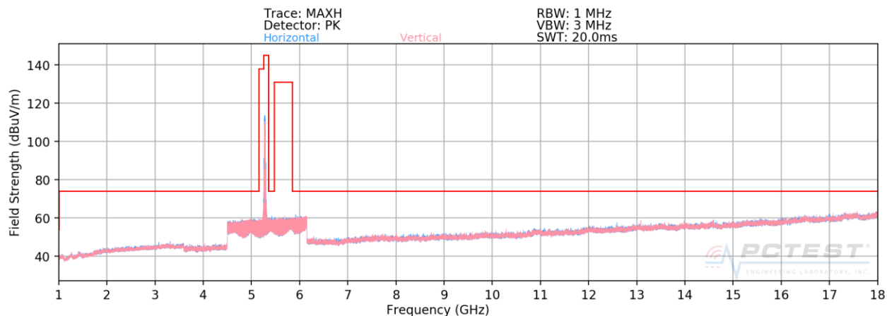
Plot 7-68. Radiated Spurious Plot above 1GHz (802.11a – U2A Ch. 56)
