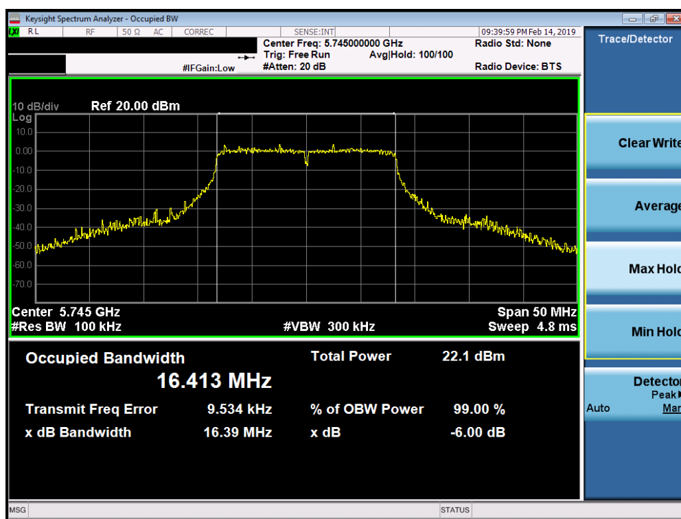
Plot 7-26. 6dB Bandwidth Plot (802.11a (UNII Band 3) – Ch. 149)
