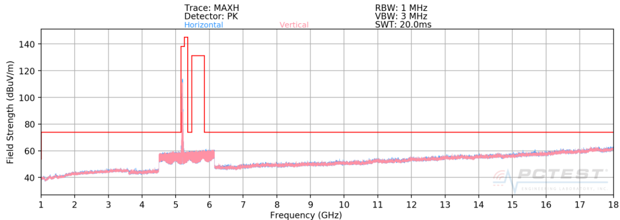
Plot 7-67. Radiated Spurious Plot above 1GHz (802.11a – U1 Ch. 40)
