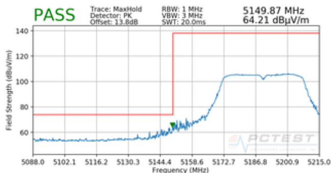
Plot 7-83. Radiated Lower Band Edge Plot (Peak – UNII Band 1)
