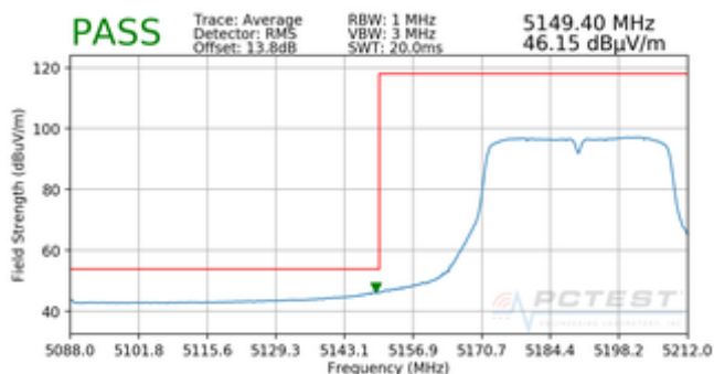
Plot 7-82. Radiated Lower Band Edge Plot (Average – UNII Band 1)
