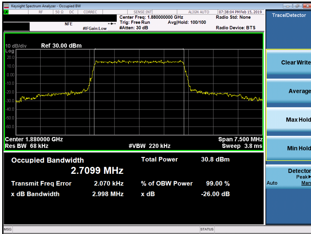
Plot 7-41. Occupied Bandwidth Plot (Band 25/2 - 3.0MHz QPSK - Full RB Configuration)
