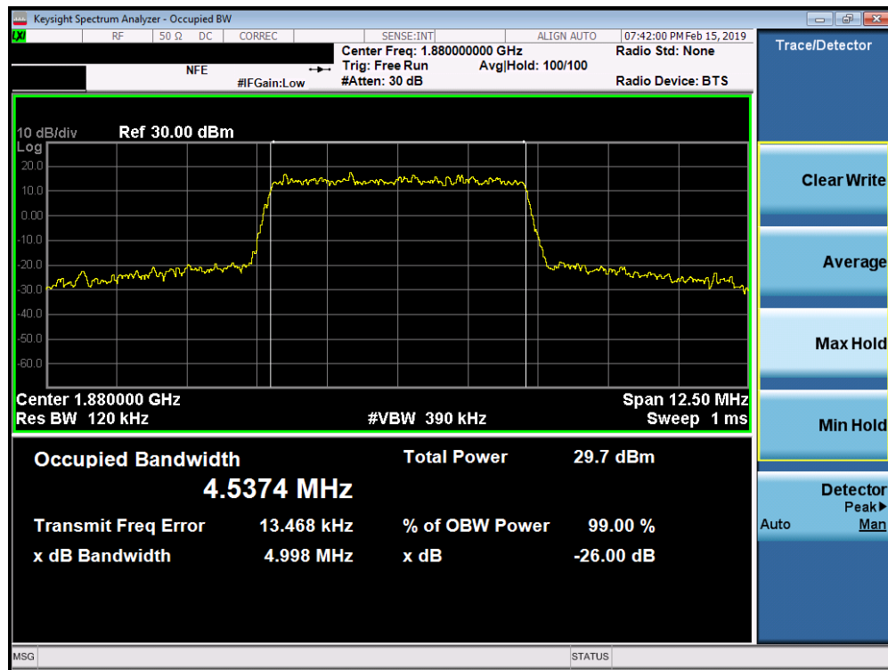
Plot 7-44. Occupied Bandwidth Plot (Band 25/2 - 5.0MHz 16-QAM - Full RB Configuration)
