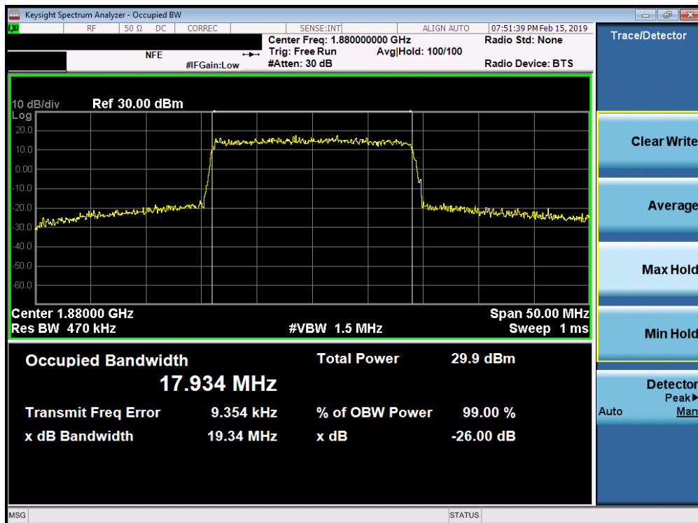
Plot 7-50. Occupied Bandwidth Plot (Band 25/2 - 20.0MHz 16-QAM - Full RB Configuration)
