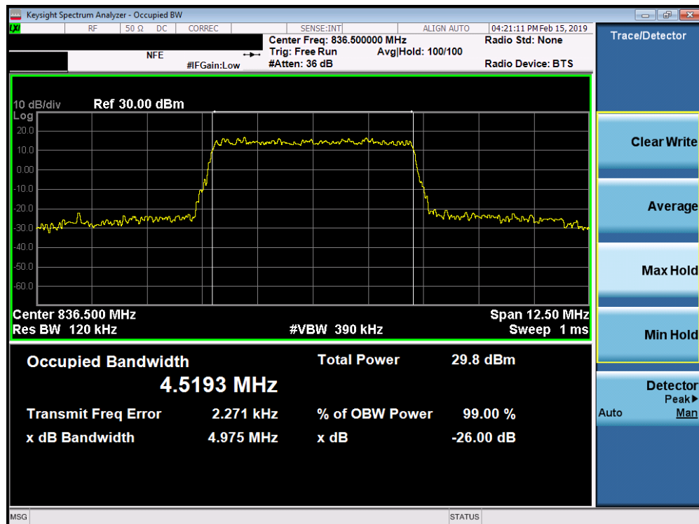
Plot 7-22. Occupied Bandwidth Plot (Band 26/5 - 5.0MHz 16-QAM - Full RB Configuration)
