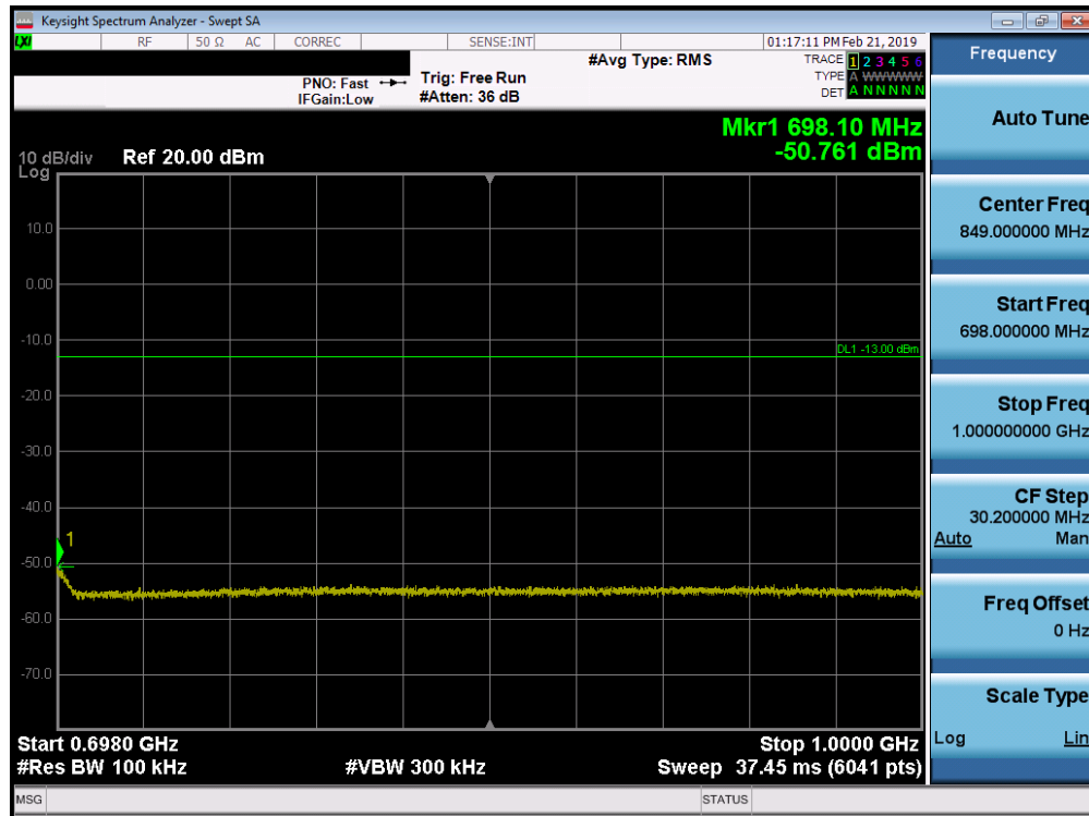
Plot 7-55. Conducted Spurious Plot (Band 71 - 10.0MHz QPSK - RB Size 1, RB Offset 0 - Mid Channel)
