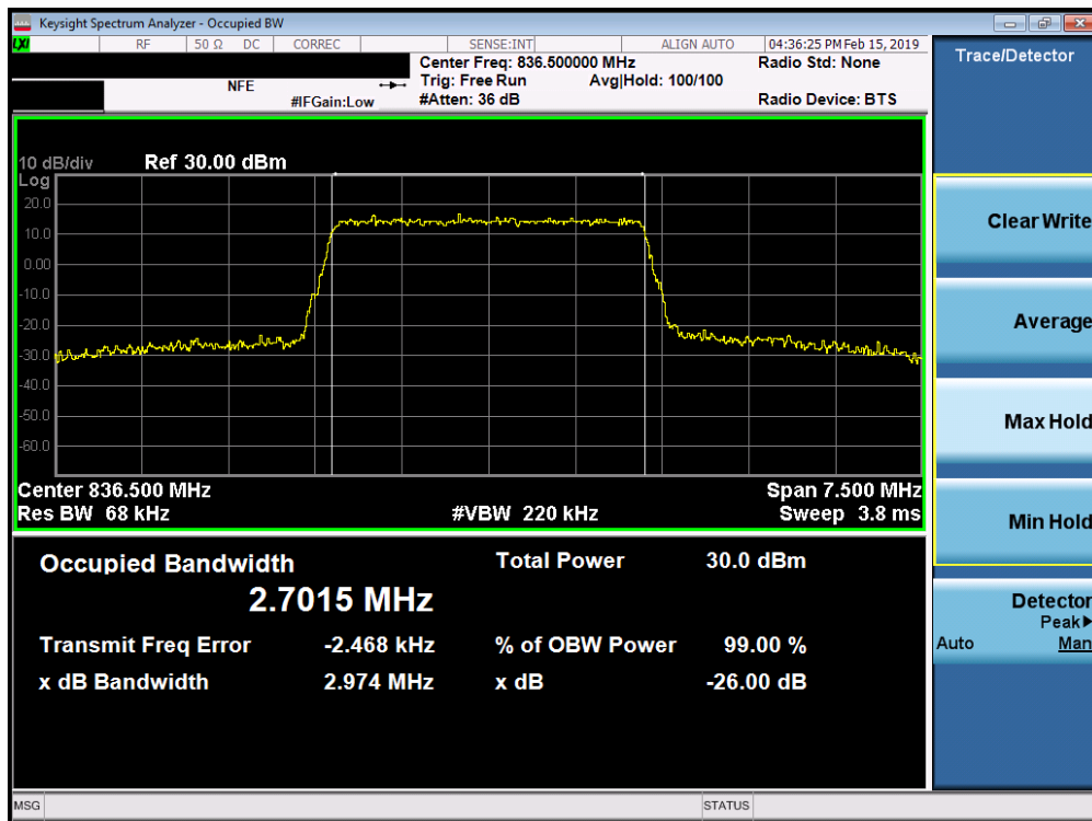
Plot 7-20. Occupied Bandwidth Plot (Band 26/5 - 3.0MHz 16-QAM - Full RB Configuration)
