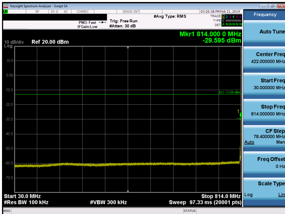
Plot 7-78. Conducted Spurious Plot (Band 26 - 15.0MHz QPSK - RB Size 1, RB Offset 0 - Mid Channel)
