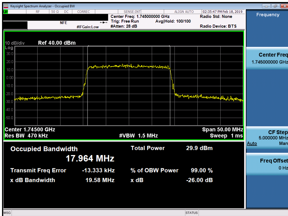
Plot 7-38. Occupied Bandwidth Plot (Band 66/4 - 20.0MHz 16-QAM - Full RB Configuration)
