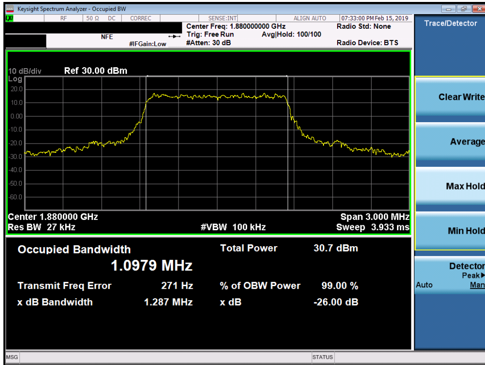
Plot 7-39. Occupied Bandwidth Plot (Band 25/2 - 1.4MHz QPSK - Full RB Configuration)
