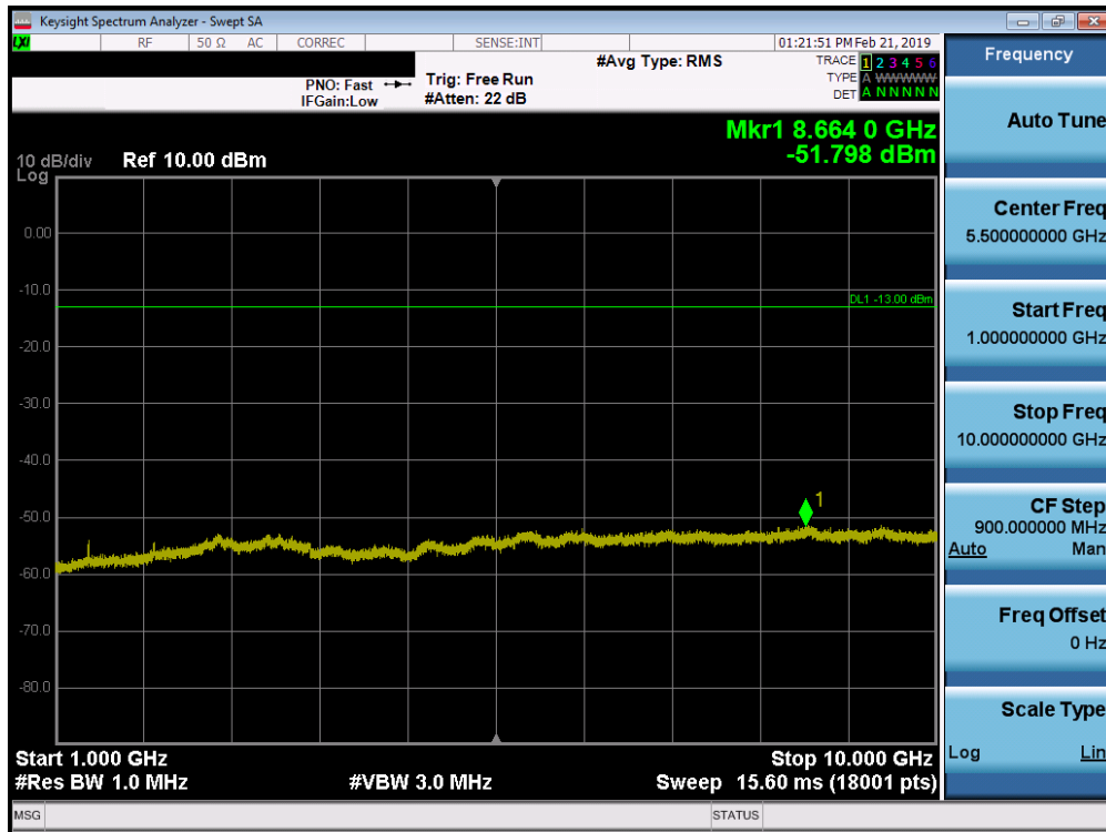
Plot 7-53. Conducted Spurious Plot (Band 71 - 10.0MHz QPSK - RB Size 1, RB Offset 0 - Low Channel)
