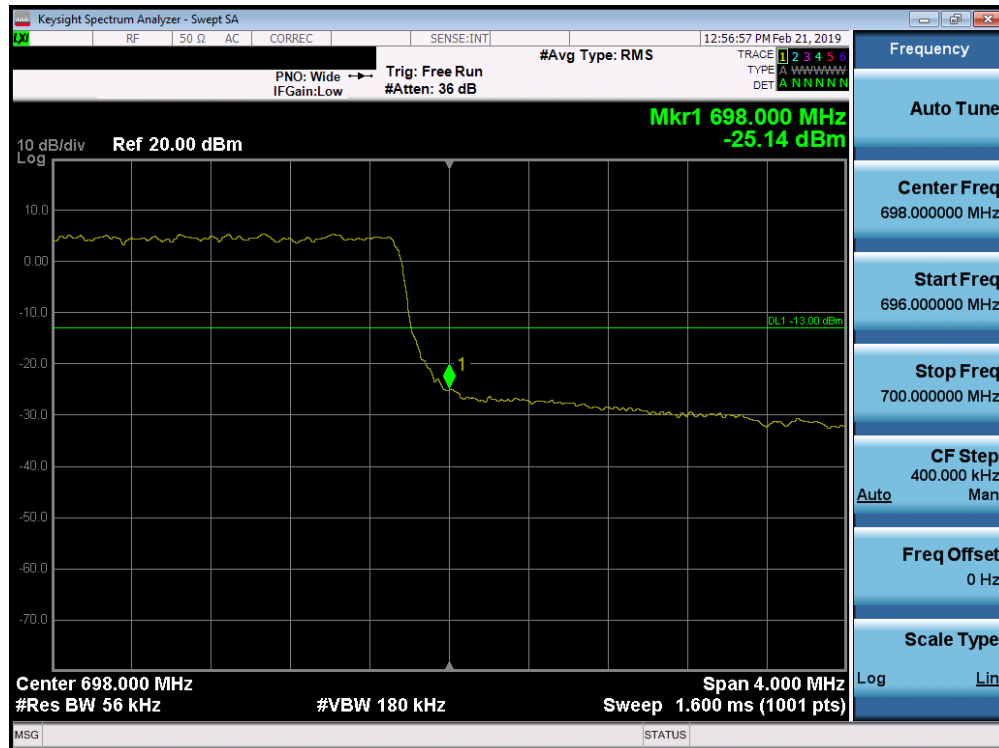
Plot 7-100. Upper Band Edge Plot (Band 71 - 5.0MHz QPSK - Full RB Configuration)
