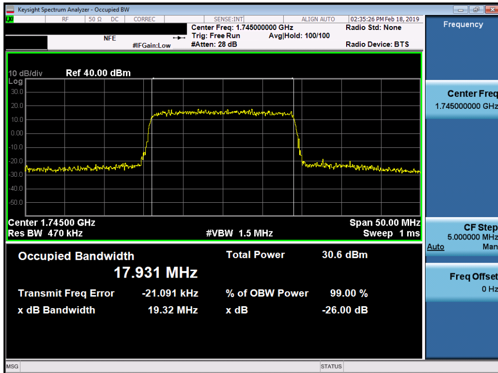
Plot 7-37. Occupied Bandwidth Plot (Band 66/4 - 20.0MHz QPSK - Full RB Configuration)
