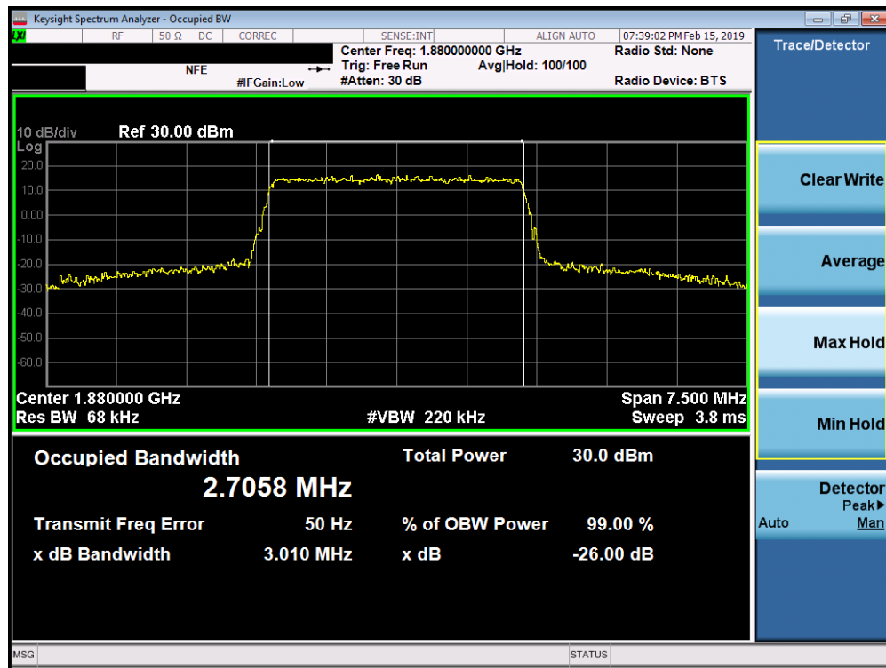
Plot 7-42. Occupied Bandwidth Plot (Band 25/2 - 3.0MHz 16-QAM - Full RB Configuration)
