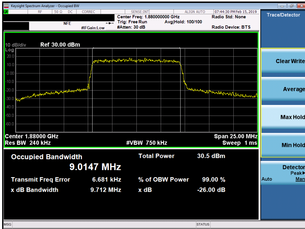
Plot 7-45. Occupied Bandwidth Plot (Band 25/2 - 10.0MHz QPSK - Full RB Configuration)
