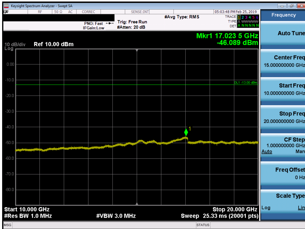
Plot 7-94. Conducted Spurious Plot (Band 25/2 - 20.0MHz QPSK - RB Size 1, RB Offset 0 - Mid Channel)
