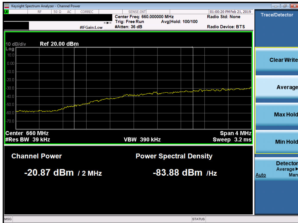
Plot 7-99. Lower Extended Band Edge Plot (Band 71 - 5.0MHz QPSK - Full RB Configuration)
