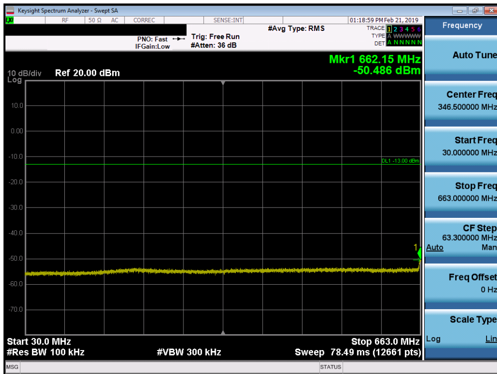
Plot 7-54. Conducted Spurious Plot (Band 71 - 10.0MHz QPSK - RB Size 1, RB Offset 0 - Mid Channel)
