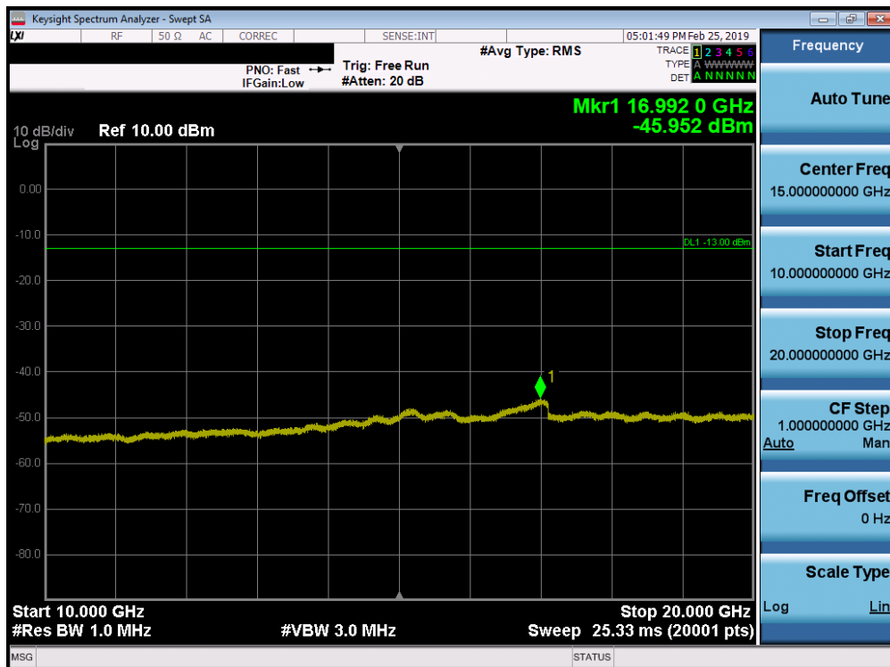
Plot 7-97. Conducted Spurious Plot (Band 25/2 - 20.0MHz QPSK - RB Size 1, RB Offset 0 - High Channel)
