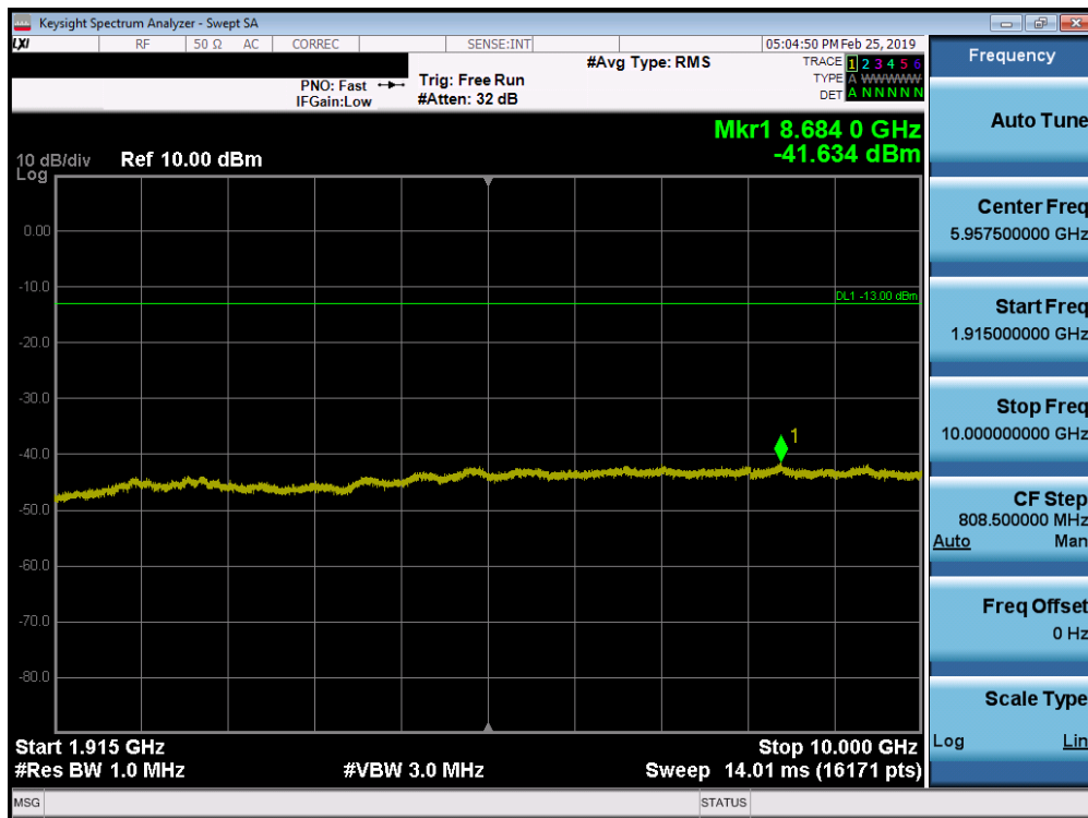
Plot 7-93. Conducted Spurious Plot (Band 25/2 - 20.0MHz QPSK - RB Size 1, RB Offset 0 - Mid Channel)
