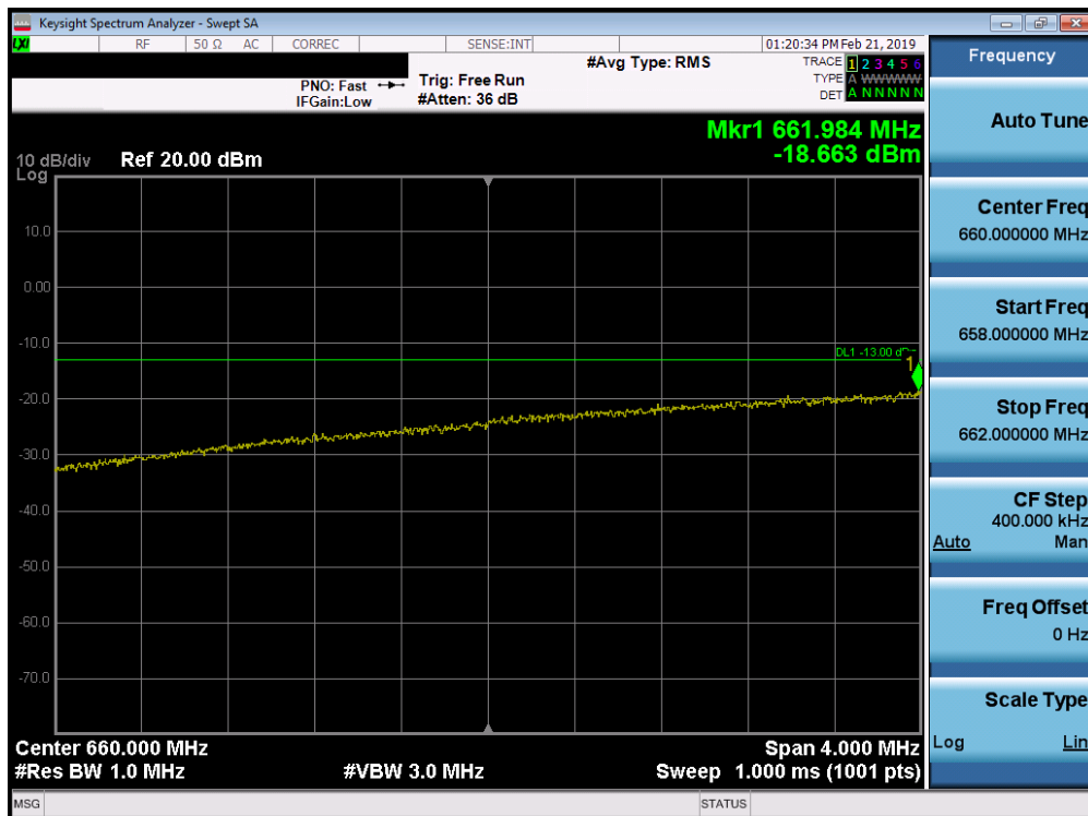
Plot 7-103. Lower Extended Band Edge Plot (Band 71 - 10.0MHz QPSK - Full RB Configuration)
