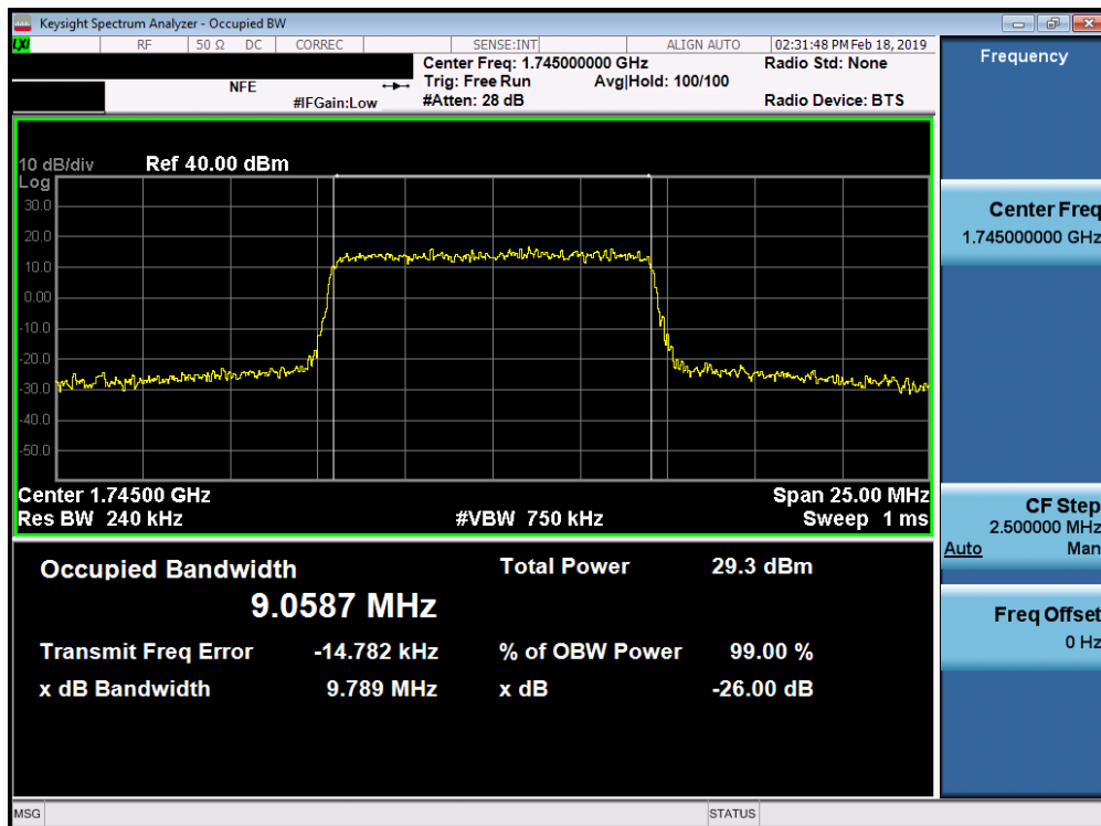
Plot 7-34. Occupied Bandwidth Plot (Band 66/4 - 10.0MHz 16-QAM - Full RB Configuration)
