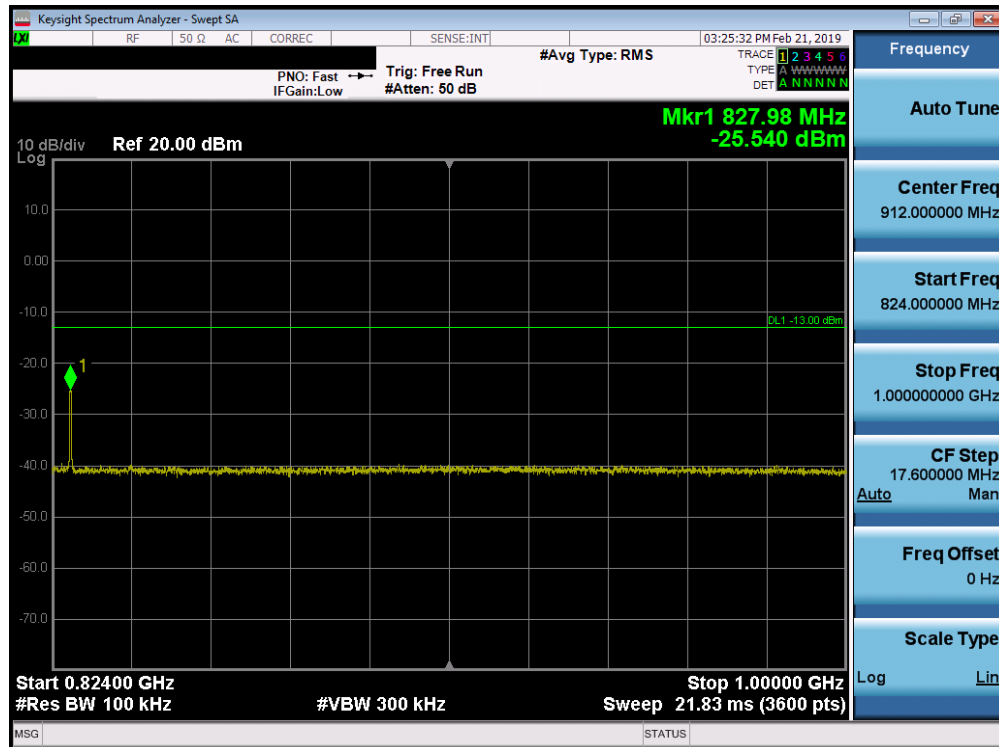
Plot 7-79. Conducted Spurious Plot (Band 26 - 15.0MHz QPSK - RB Size 1, RB Offset 0 - Mid Channel)
