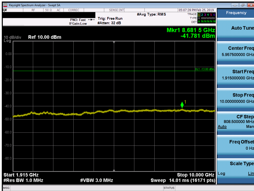
Plot 7-91. Conducted Spurious Plot (Band 25/2 - 20.0MHz QPSK - RB Size 1, RB Offset 0 - Low Channel)
