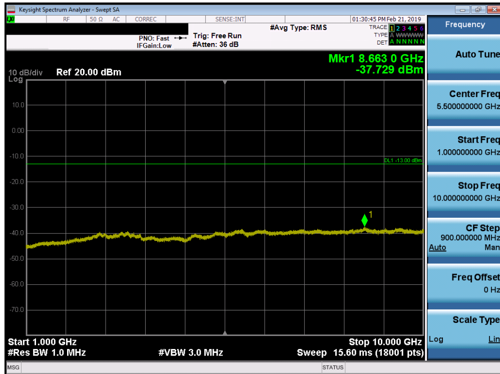
Plot 7-59. Conducted Spurious Plot (Band 71 - 10.0MHz QPSK - RB Size 1, RB Offset 0 - High Channel)
