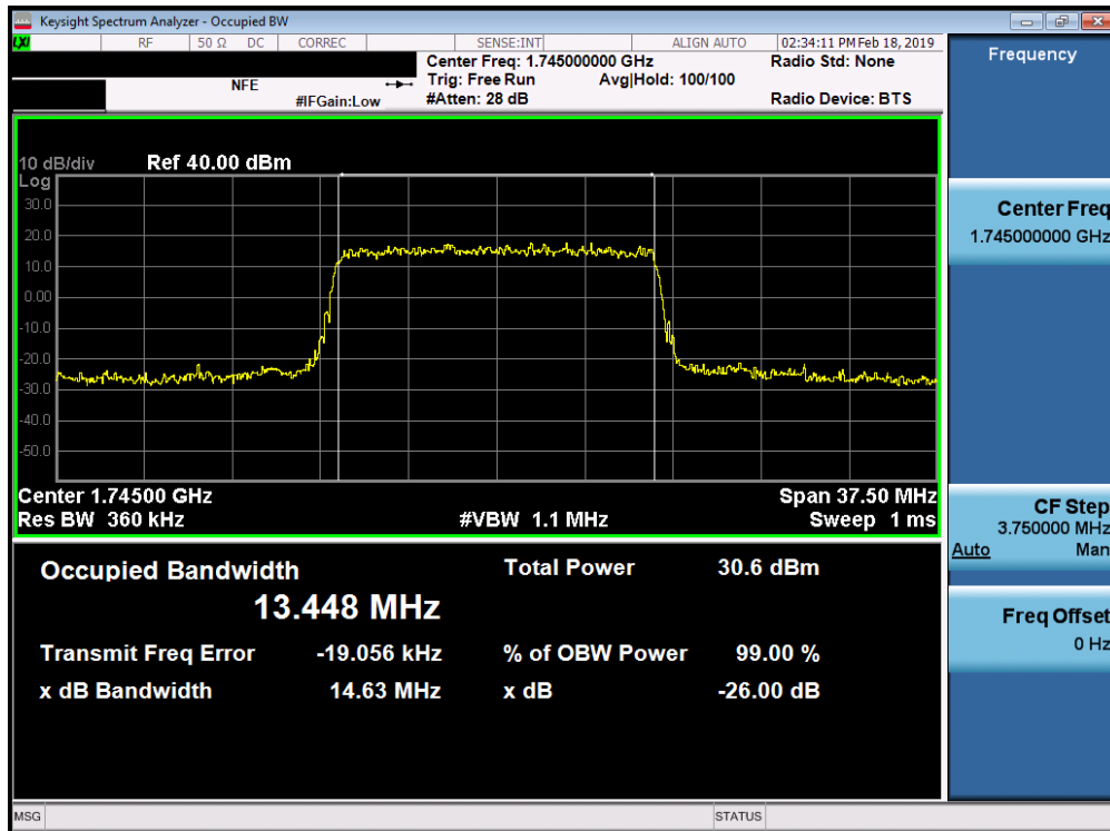
Plot 7-35. Occupied Bandwidth Plot (Band 66/4 - 15.0MHz QPSK - Full RB Configuration)
