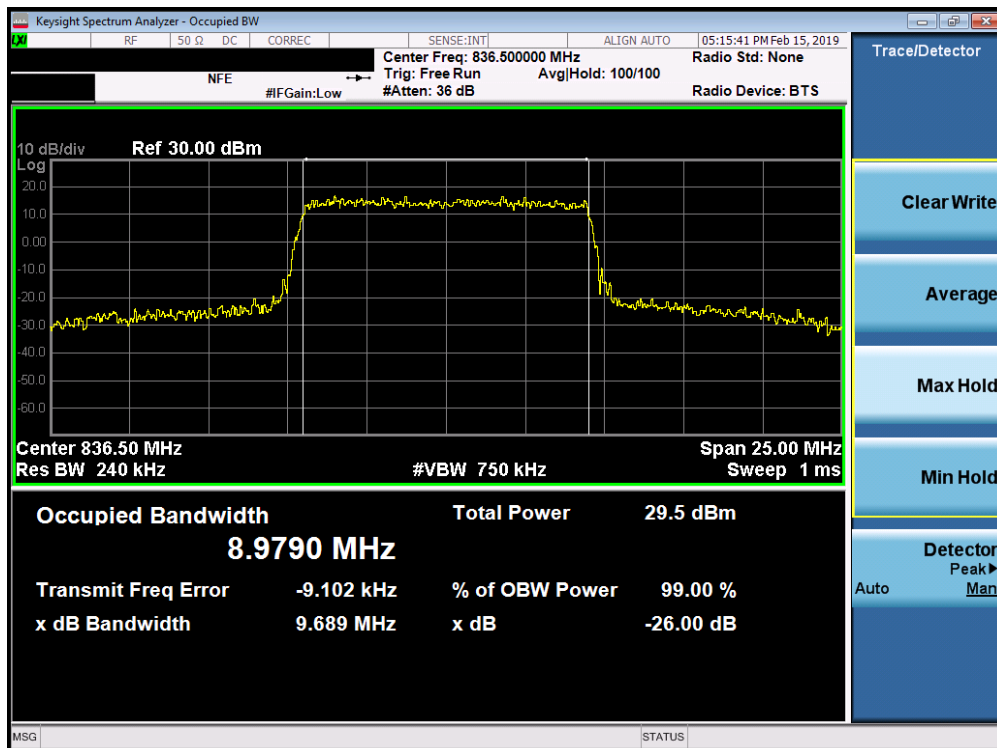
Plot 7-24. Occupied Bandwidth Plot (Band 26/5 - 10.0MHz 16-QAM - Full RB Configuration)
