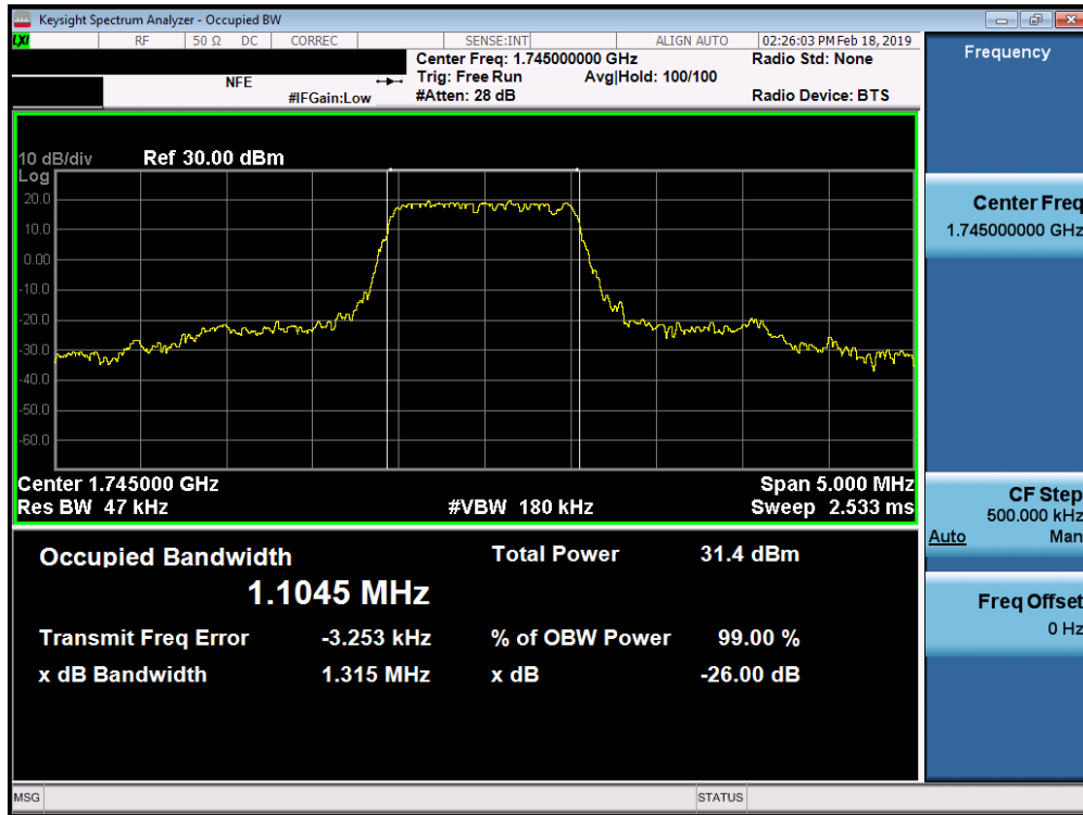
Plot 7-27. Occupied Bandwidth Plot (Band 66/4 - 1.4MHz QPSK - Full RB Configuration)
