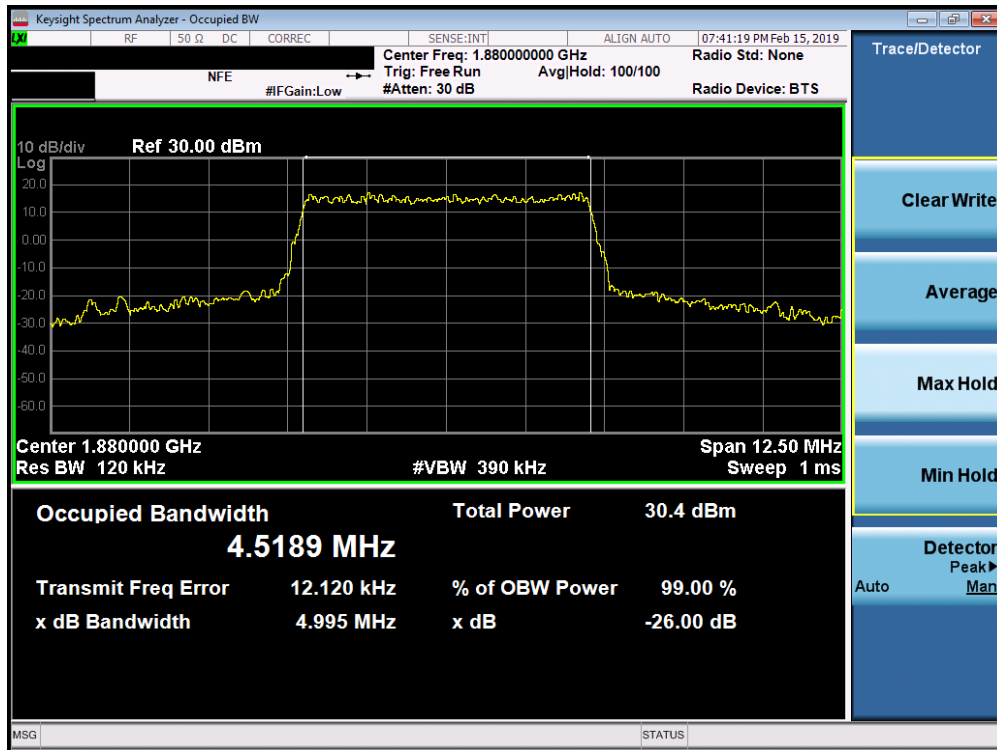
Plot 7-43. Occupied Bandwidth Plot (Band 25/2 - 5.0MHz QPSK - Full RB Configuration)
