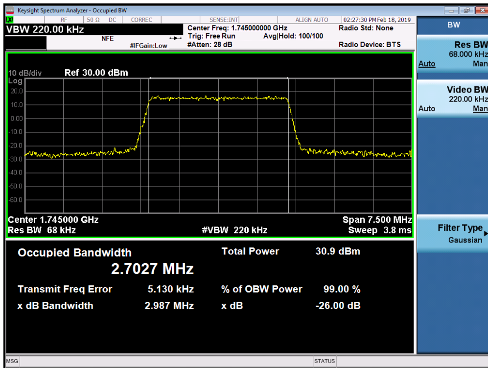
Plot 7-29. Occupied Bandwidth Plot (Band 66/4 - 3.0MHz QPSK - Full RB Configuration)
