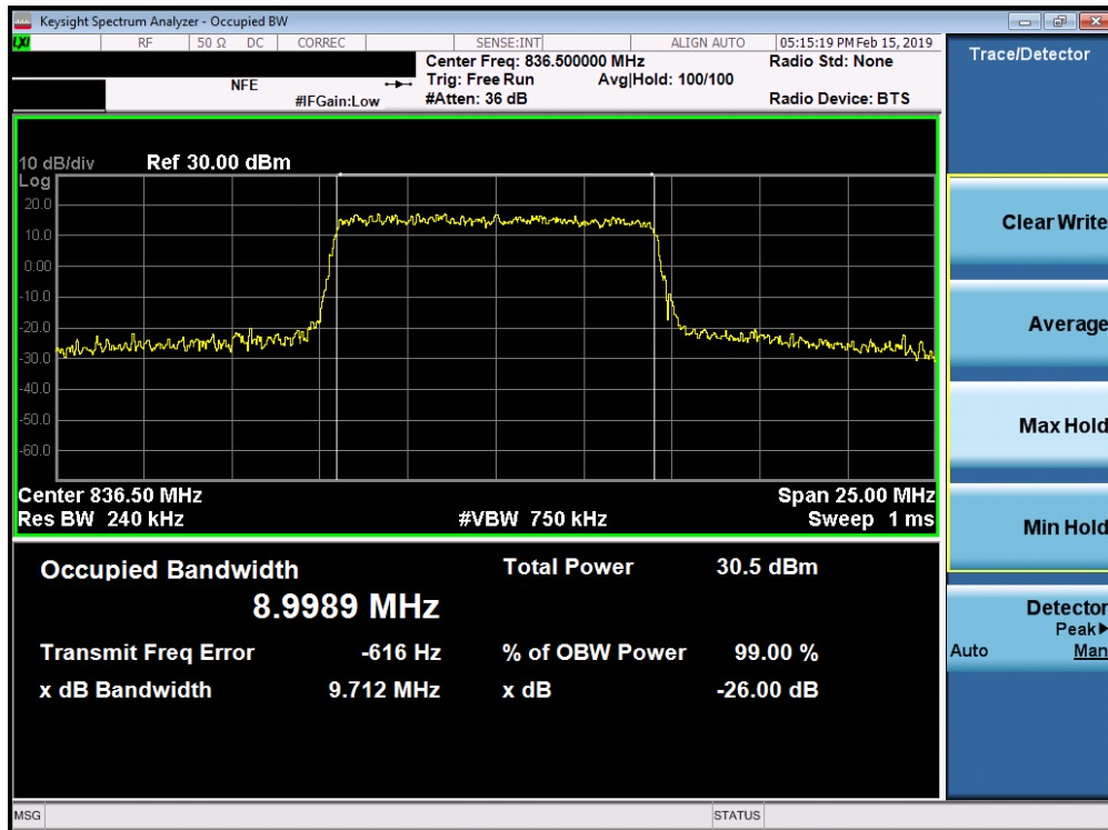
Plot 7-23. Occupied Bandwidth Plot (Band 26/5 - 10.0MHz QPSK - Full RB Configuration)
