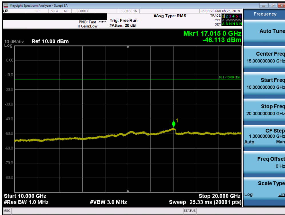
Plot 7-92. Conducted Spurious Plot (Band 25/2 - 20.0MHz QPSK - RB Size 1, RB Offset 0 - Low Channel)
