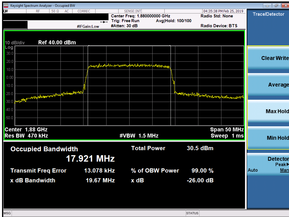
Plot 7-49. Occupied Bandwidth Plot (Band 25/2 - 20.0MHz QPSK - Full RB Configuration)
