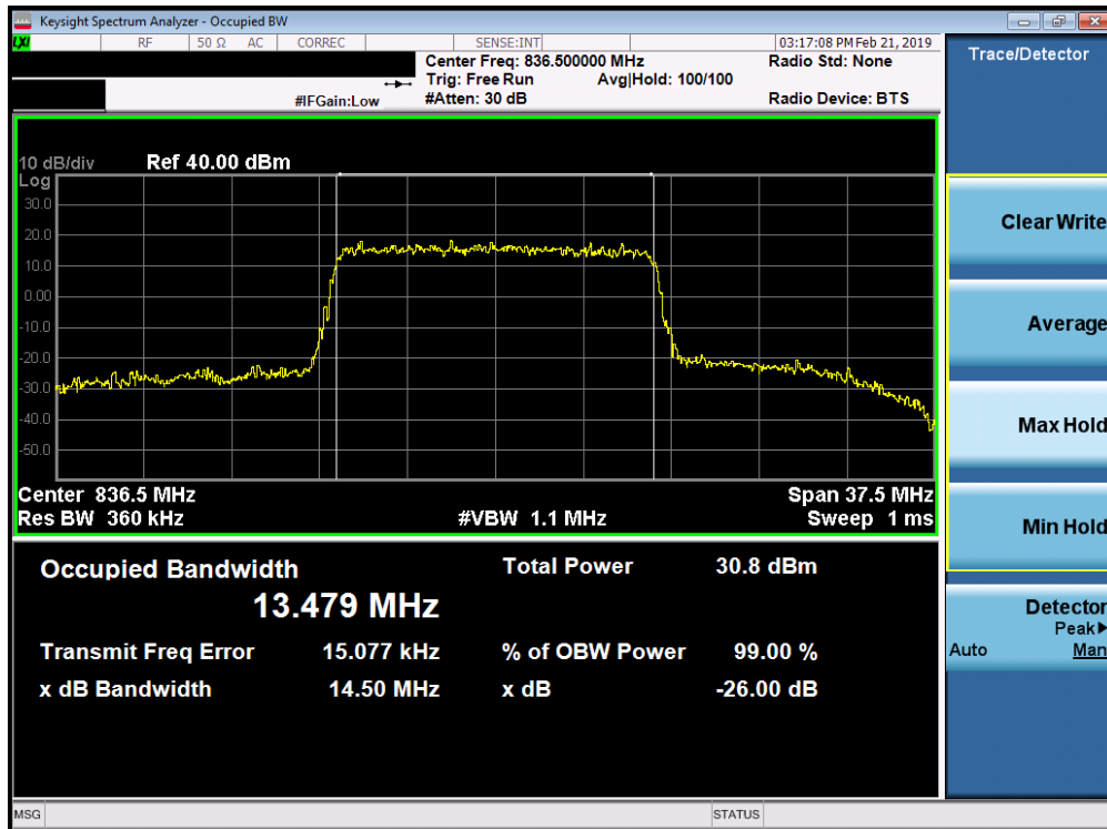
Plot 7-25. Occupied Bandwidth Plot (Band 26 - 15.0MHz QPSK - Full RB Configuration)
