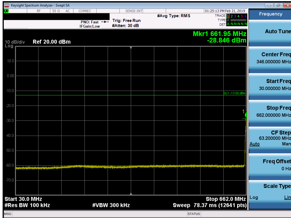
Plot 7-51. Conducted Spurious Plot (Band 71 - 10.0MHz QPSK - RB Size 1, RB Offset 0 - Low Channel)
