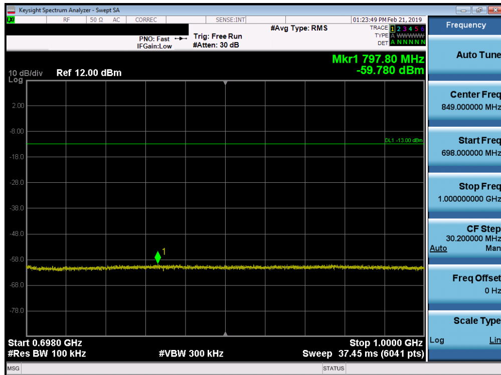
Plot 7-52. Conducted Spurious Plot (Band 71 - 10.0MHz QPSK - RB Size 1, RB Offset 0 - Low Channel)
