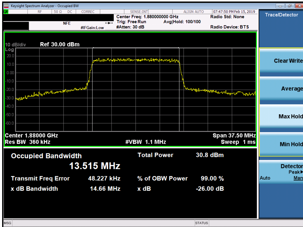
Plot 7-47. Occupied Bandwidth Plot (Band 25/2 - 15.0MHz QPSK - Full RB Configuration)
