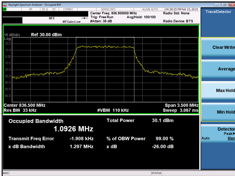
Plot 7-18. Occupied Bandwidth Plot (Band 26/5 - 1.4MHz 16-QAM - Full RB Configuration)
