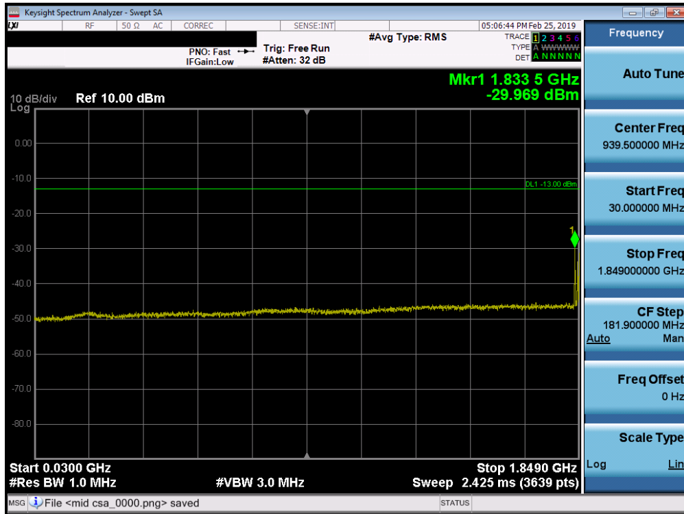
Plot 7-90. Conducted Spurious Plot (Band 25/2 - 20.0MHz QPSK - RB Size 1, RB Offset 0 - Low Channel)
