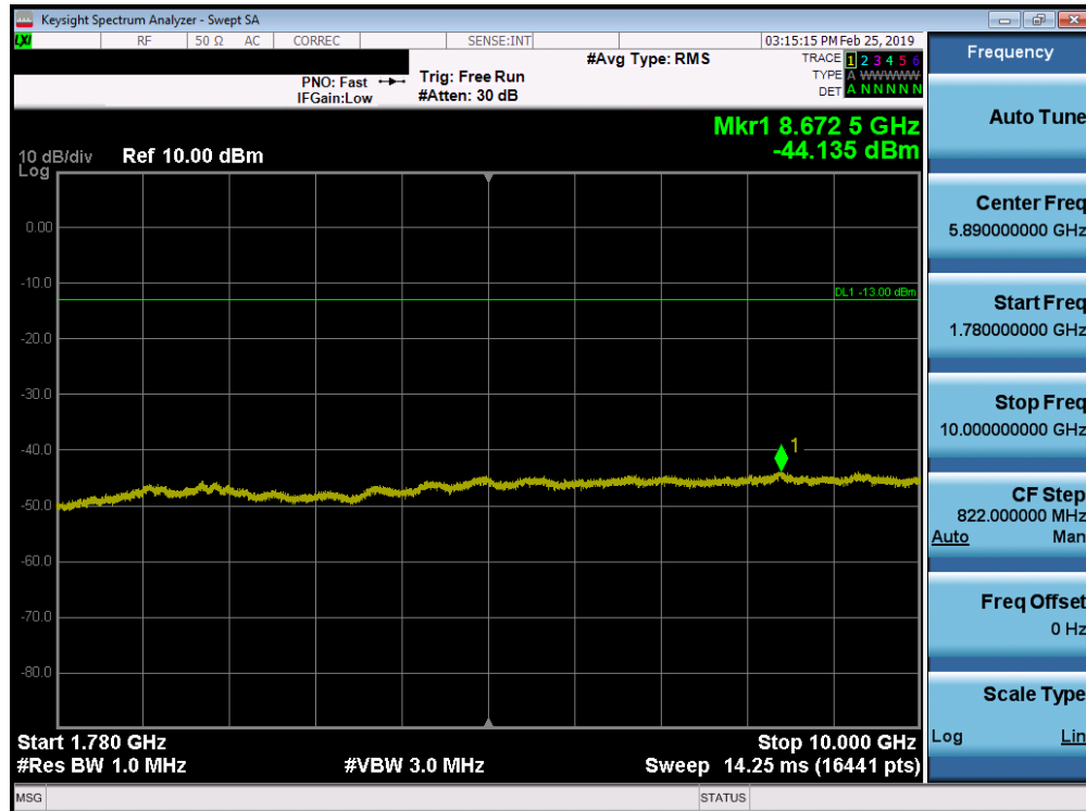
Plot 7-82. Conducted Spurious Plot (Band 66/4 - 20.0MHz QPSK - RB Size 1, RB Offset 0 - Low Channel)
