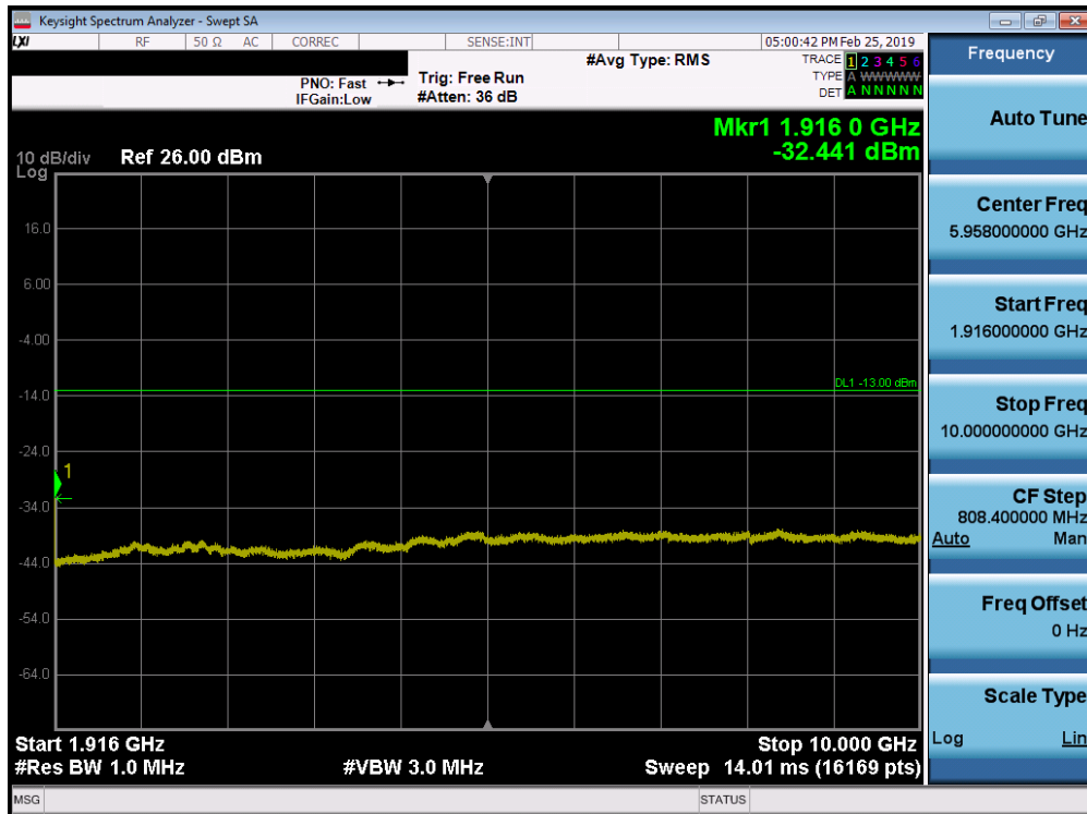
Plot 7-96. Conducted Spurious Plot (Band 25/2 - 20.0MHz QPSK - RB Size 1, RB Offset 0 - High Channel)
