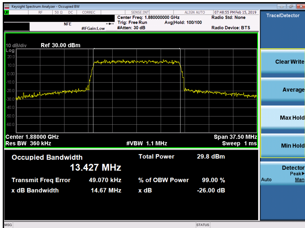
Plot 7-48. Occupied Bandwidth Plot (Band 25/2 - 15.0MHz 16-QAM - Full RB Configuration)
