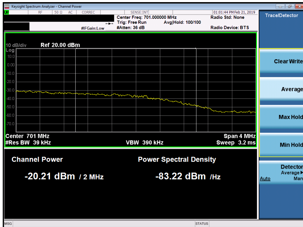
Plot 7-101. Upper Extended Band Edge Plot (Band 71 - 5.0MHz QPSK - Full RB Configuration)
