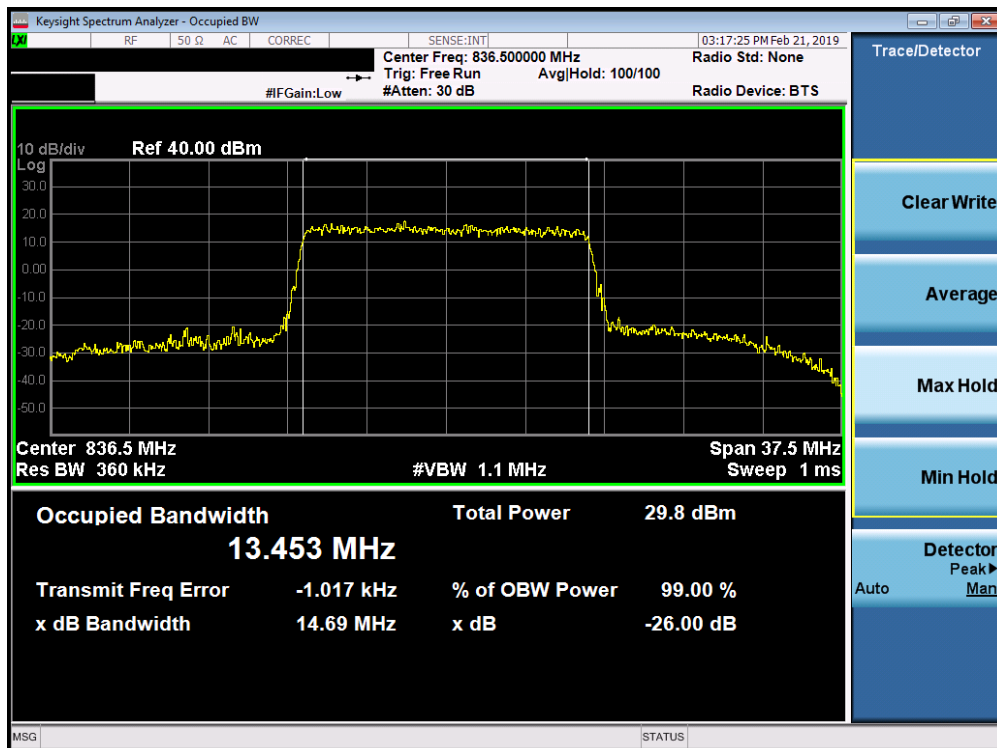
Plot 7-26. Occupied Bandwidth Plot (Band 26 - 15.0MHz 16-QAM - Full RB Configuration)
