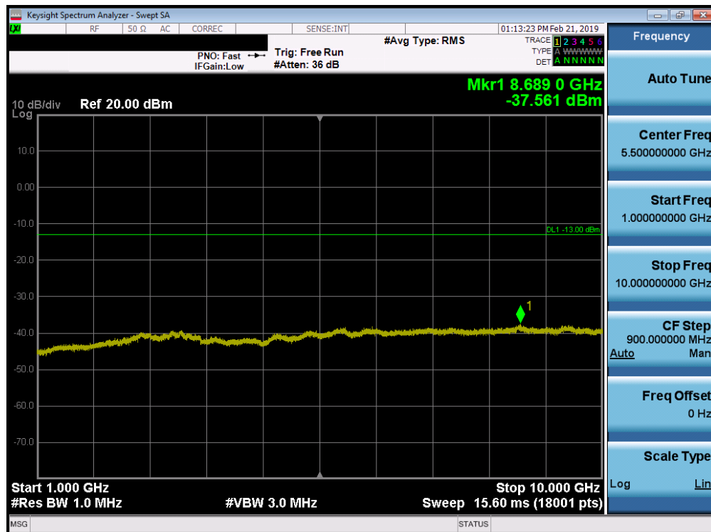
Plot 7-56. Conducted Spurious Plot (Band 71 - 10.0MHz QPSK - RB Size 1, RB Offset 0 - Mid Channel)
