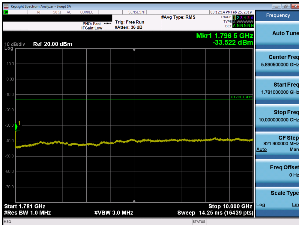
Plot 7-88. Conducted Spurious Plot (Band 66/4 - 20.0MHz QPSK - RB Size 1, RB Offset 0 - High Channel)
