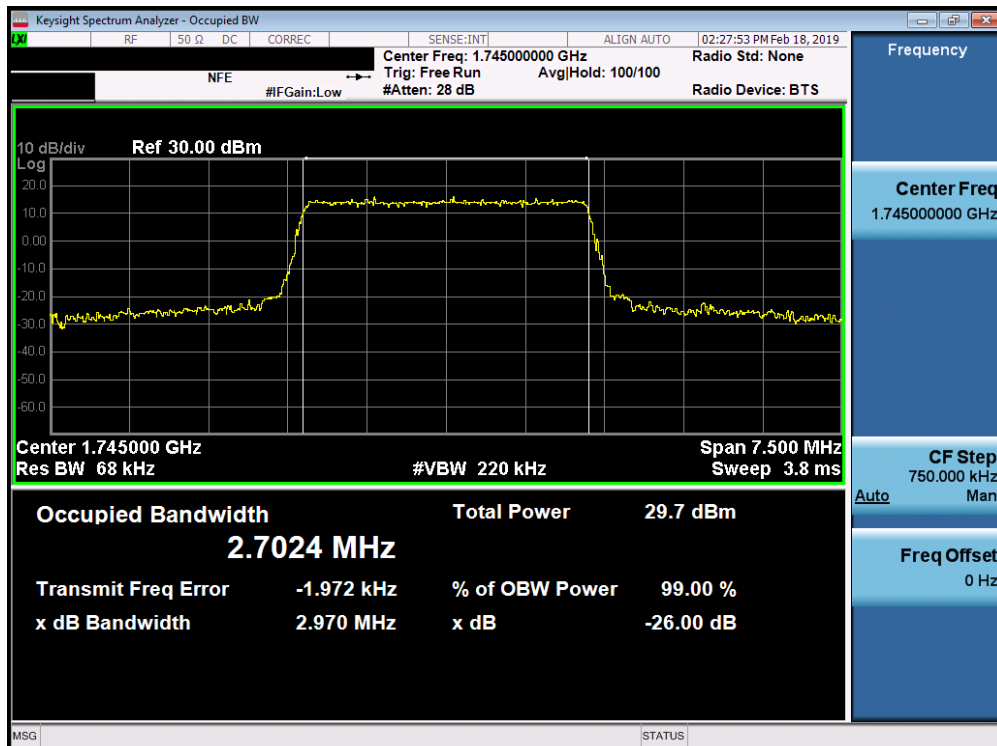
Plot 7-30. Occupied Bandwidth Plot (Band 66/4 - 3.0MHz 16-QAM - Full RB Configuration)
