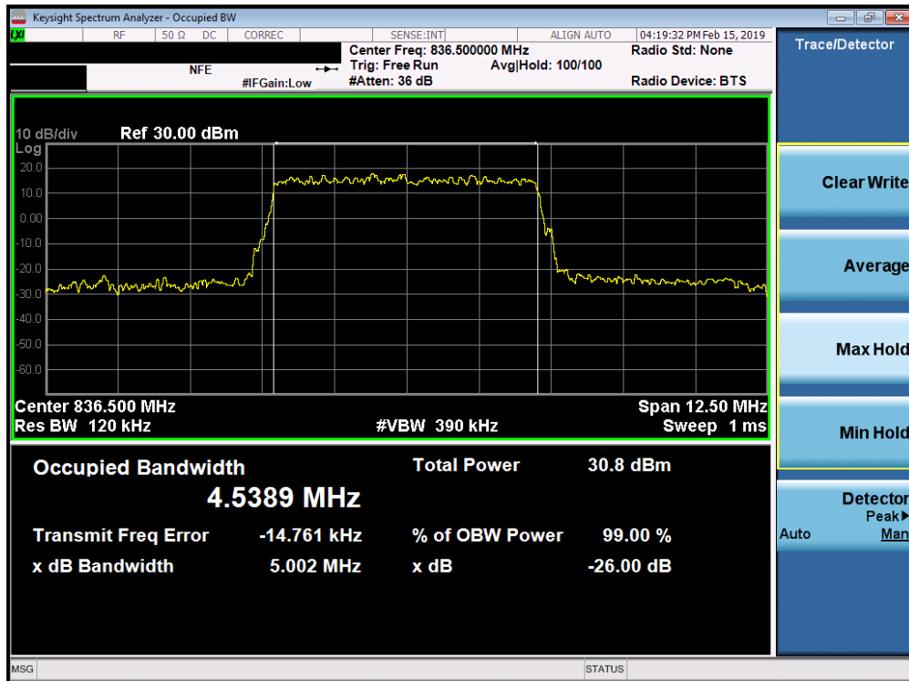
Plot 7-21. Occupied Bandwidth Plot (Band 26/5 - 5.0MHz QPSK - Full RB Configuration)
