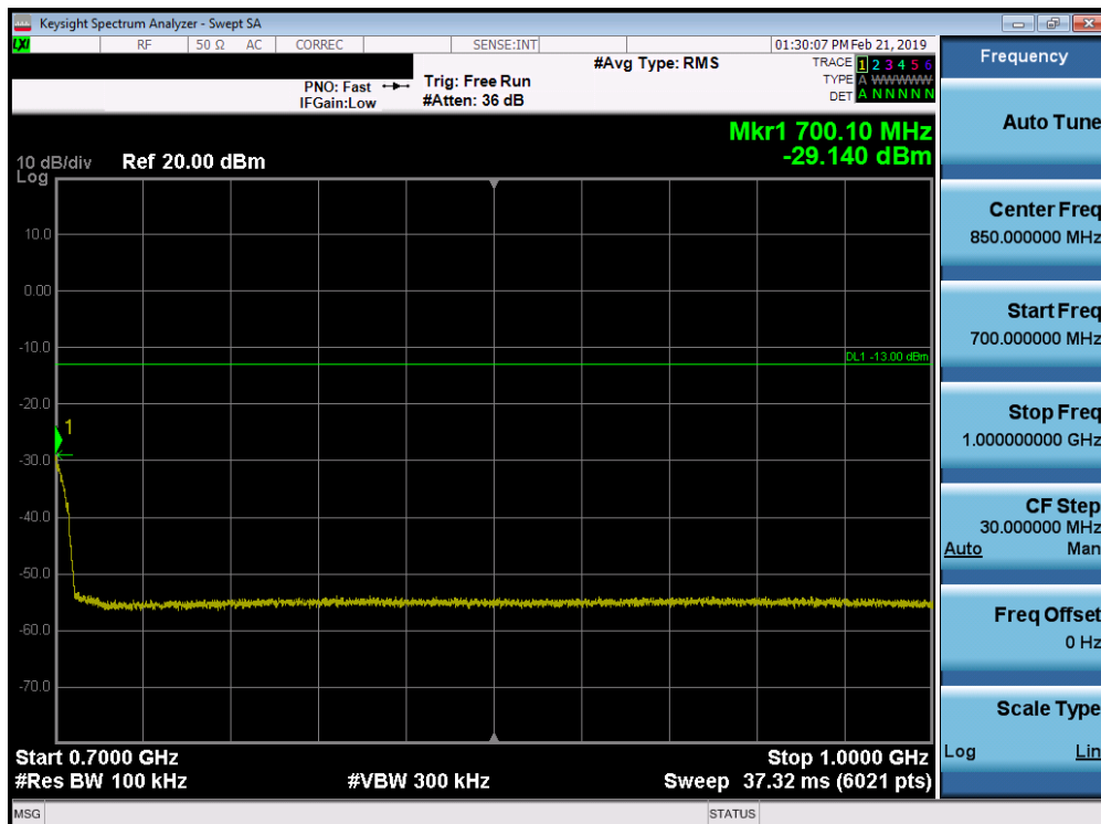
Plot 7-58. Conducted Spurious Plot (Band 71 - 10.0MHz QPSK - RB Size 1, RB Offset 0 - High Channel)
