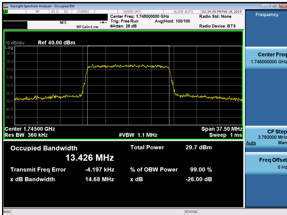
Plot 7-36. Occupied Bandwidth Plot (Band 66/4 - 15.0MHz 16-QAM - Full RB Configuration)
