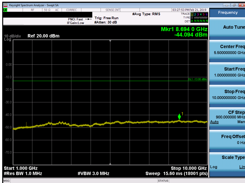
Plot 7-80. Conducted Spurious Plot (Band 26 - 15.0MHz QPSK - RB Size 1, RB Offset 0 - Mid Channel)
