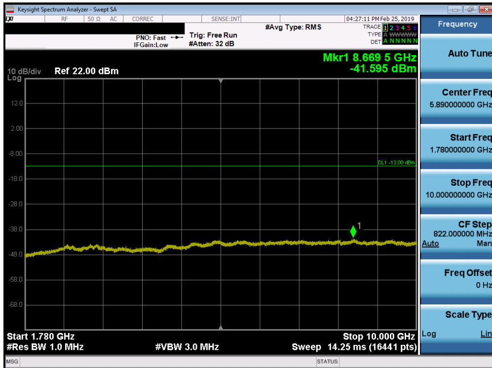
Plot 7-85. Conducted Spurious Plot (Band 66/4 - 20.0MHz QPSK - RB Size 1, RB Offset 0 - Mid Channel)
