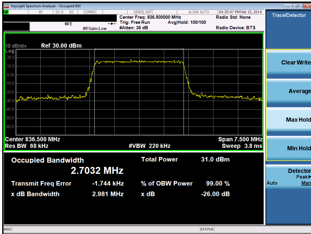
Plot 7-19. Occupied Bandwidth Plot (Band 26/5 - 3.0MHz QPSK - Full RB Configuration)
