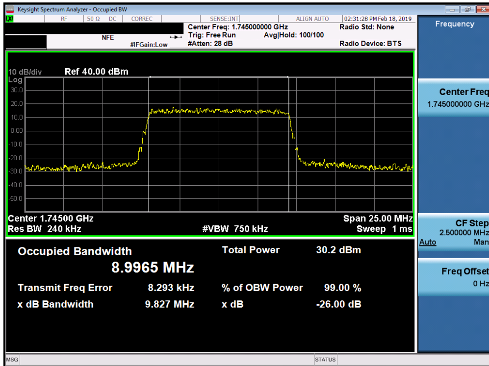
Plot 7-33. Occupied Bandwidth Plot (Band 66/4 - 10.0MHz QPSK - Full RB Configuration)
