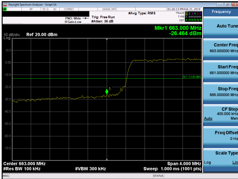
Plot 7-102. Lower Band Edge Plot (Band 71 - 10.0MHz QPSK - Full RB Configuration)
