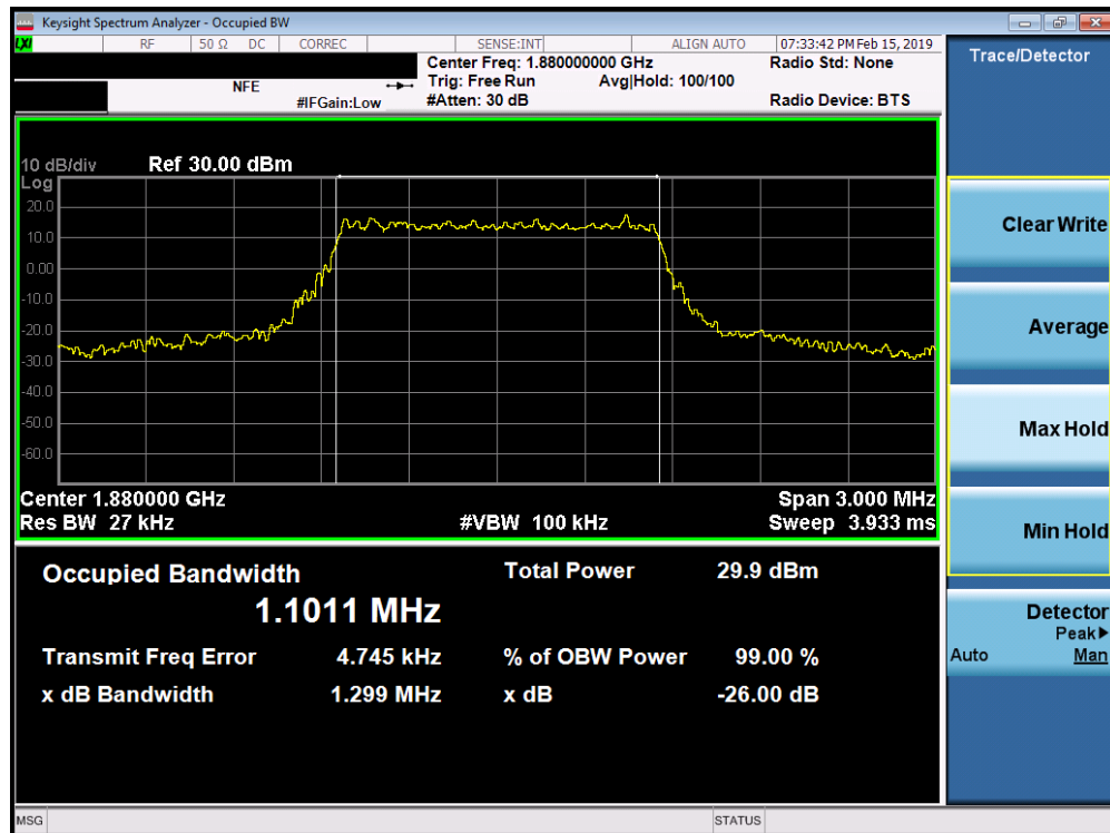
Plot 7-40. Occupied Bandwidth Plot (Band 25/2 - 1.4MHz 16-QAM - Full RB Configuration)
