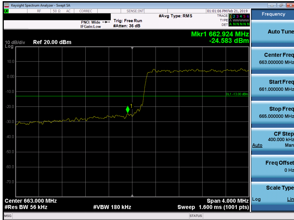
Plot 7-98. Lower Band Edge Plot (Band 71 - 5.0MHz QPSK - Full RB Configuration)
