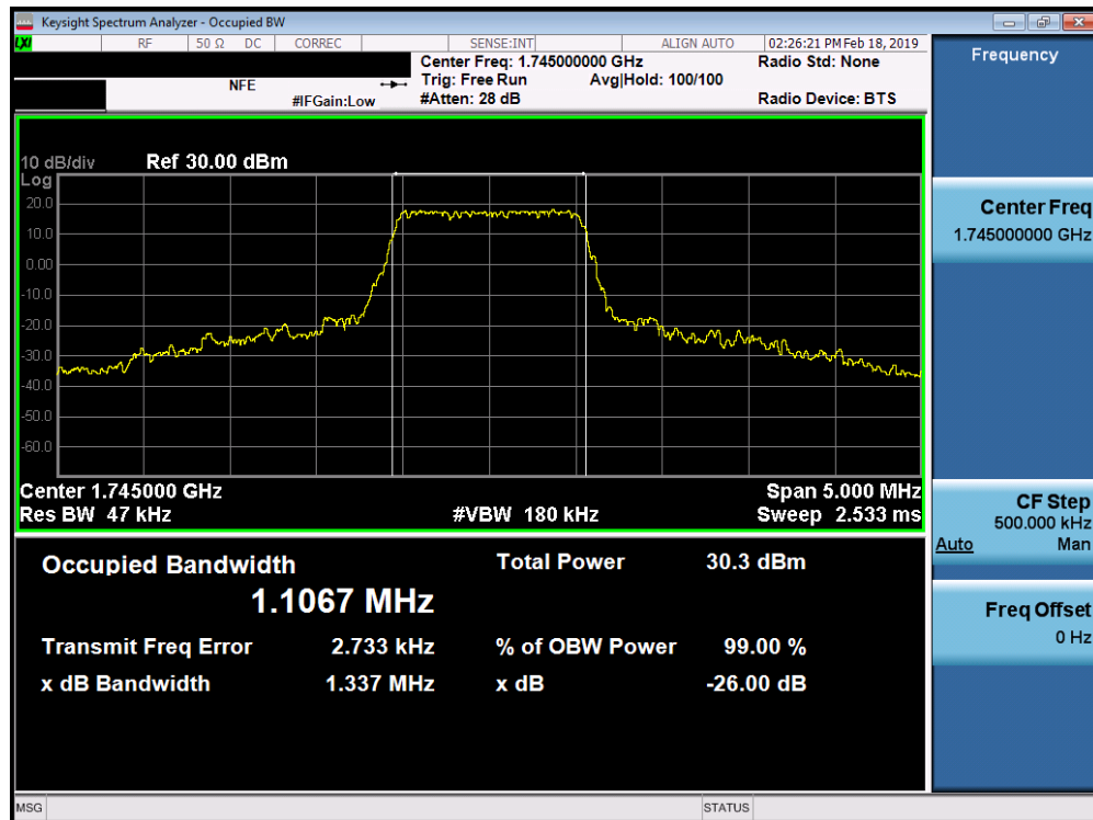
Plot 7-28. Occupied Bandwidth Plot (Band 66/4 - 1.4MHz 16-QAM - Full RB Configuration)
