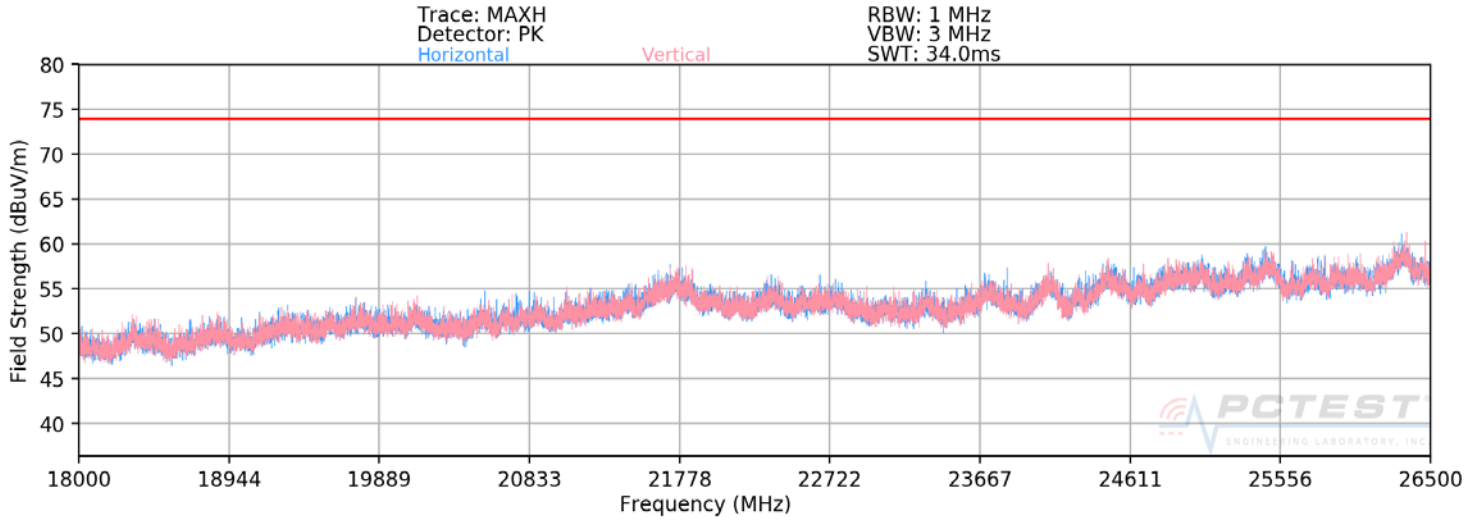
Plot 7-40. Radiated Spurious Plot above 18GHz
