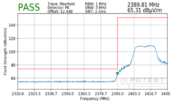
Plot 7-42. Radiated Restricted Lower Band Edge Measurement (Peak)
