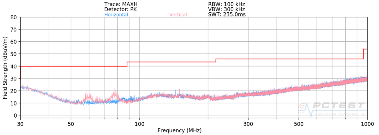
Plot 7-49. Radiated Spurious Plot below 1GHz
