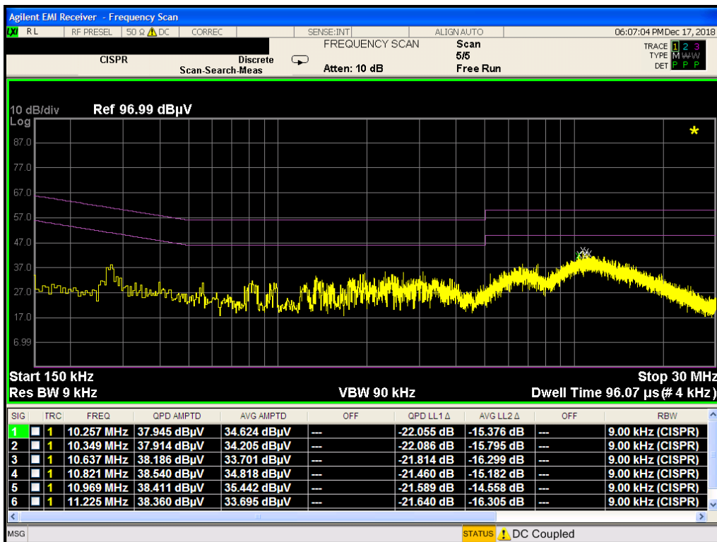
Plot 7-51. Line Conducted Plot with 802.11b (N)
