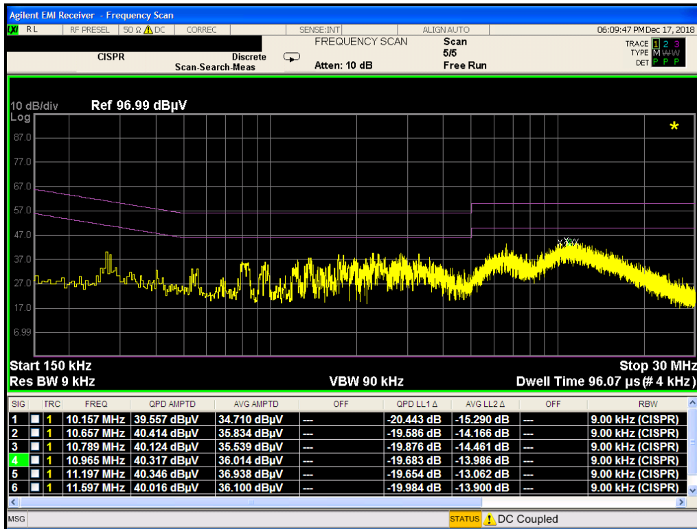
Plot 7-50. Line Conducted Plot with 802.11b (L1)
