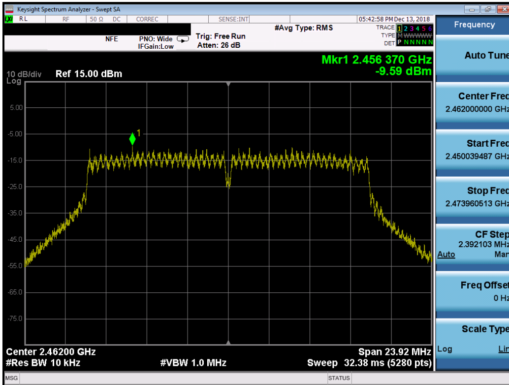
Plot 7-15. Power Spectral Density Plot (802.11g – Ch. 11)
