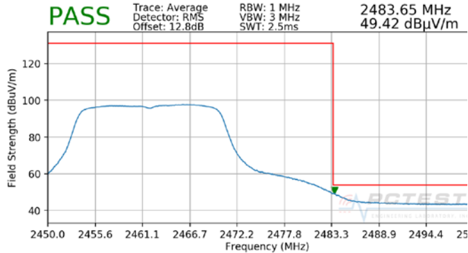
Plot 7-47. Radiated Restricted Upper Band Edge Measurement (Average)
