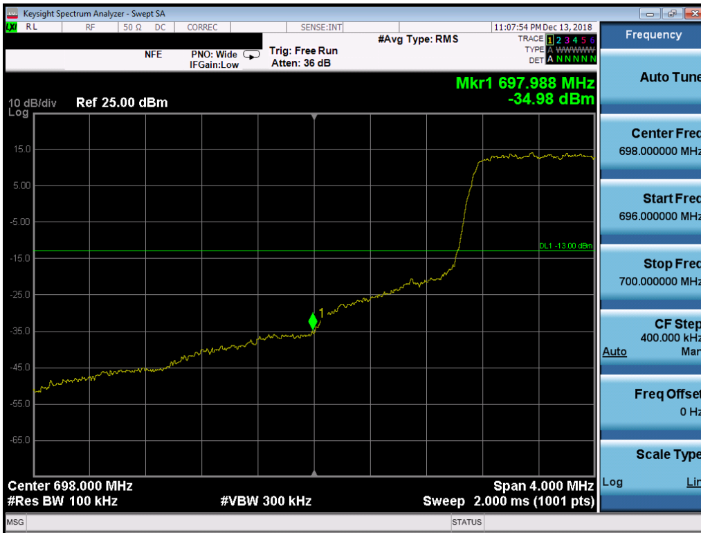
Plot 7-77. Lower Band Edge Plot (Band 12 - 1.4MHz QPSK - Full RB Configuration)
