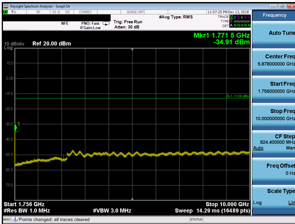
Plot 7-66. Conducted Spurious Plot (Band 4 - 20MHz QPSK - RB Size 1, RB Offset 0 - High Channel)
