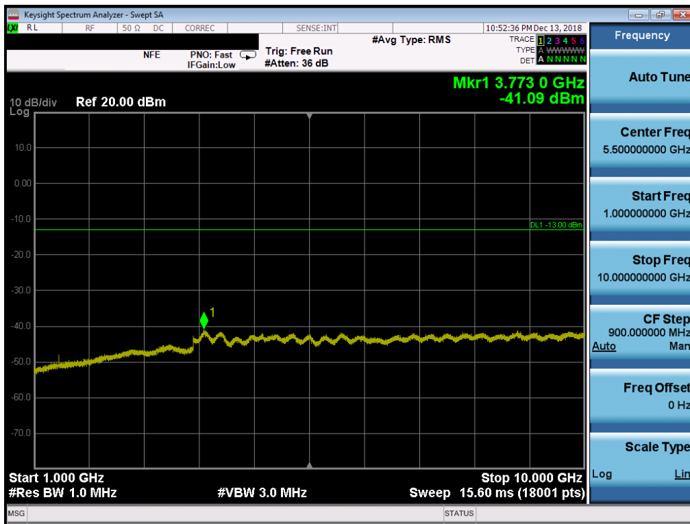
Plot 7-46. Conducted Spurious Plot (Band 12 - 10MHz QPSK - RB Size 1, RB Offset 0 - Mid Channel)
