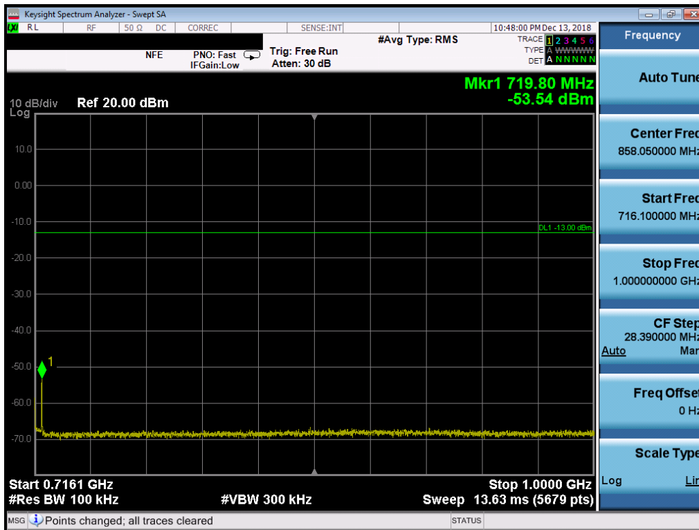
Plot 7-48. Conducted Spurious Plot (Band 12 - 10MHz QPSK - RB Size 1, RB Offset 0 - High Channel)
