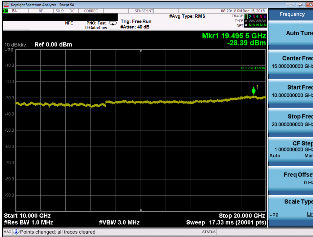
Plot 7-76. Conducted Spurious Plot (Band 25/2 - 20MHz QPSK - RB Size 1, RB Offset 0 - High Channel)
