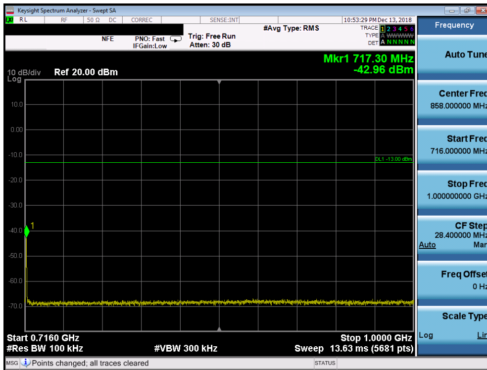
Plot 7-42. Conducted Spurious Plot (Band 12 - 10MHz QPSK - RB Size 1, RB Offset 0 - Low Channel)
