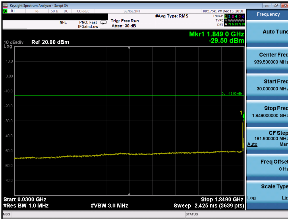
Plot 7-68. Conducted Spurious Plot (Band 25/2 - 20MHz QPSK - RB Size 1, RB Offset 0 - Low Channel)
