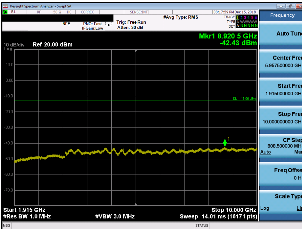
Plot 7-69. Conducted Spurious Plot (Band 25/2 - 20MHz QPSK - RB Size 1, RB Offset 0 - Low Channel)
