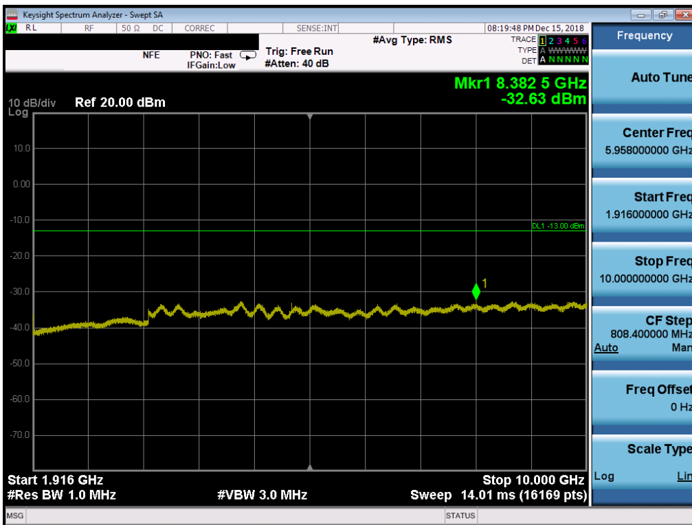
Plot 7-75. Conducted Spurious Plot (Band 25/2 - 20MHz QPSK - RB Size 1, RB Offset 0 - High Channel)
