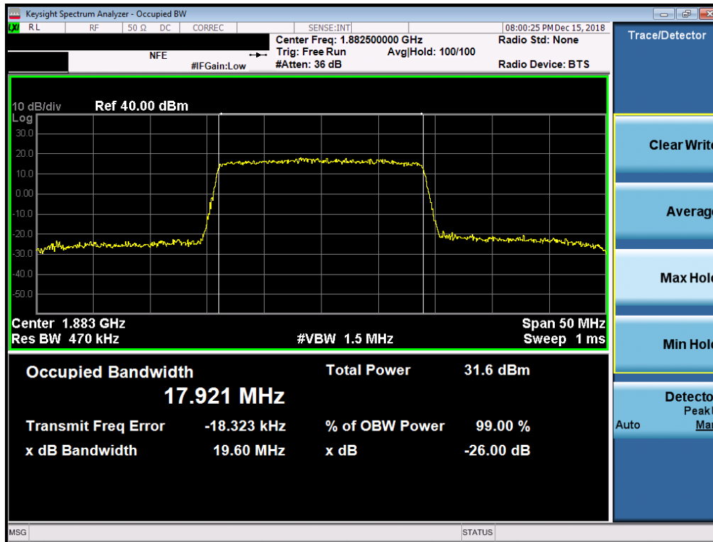
Plot 7-40. Occupied Bandwidth Plot (Band 25/2 - 20.0MHz 16-QAM - Full RB Configuration)
