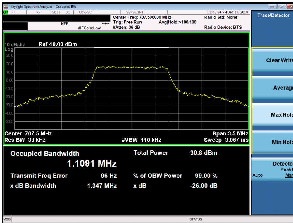
Plot 7-2. Occupied Bandwidth Plot (Band 12 - 1.4MHz 16-QAM - Full RB Configuration)
