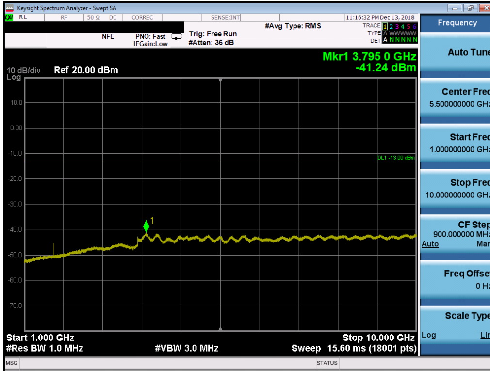
Plot 7-58. Conducted Spurious Plot (Band 5 - 10MHz QPSK - RB Size 1, RB Offset 0 - High Channel)
