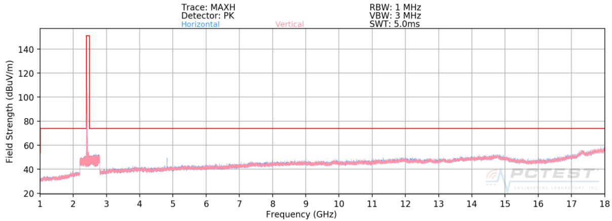
Plot 7-31. Radiated Spurious Plot above 1GHz (802.11b – Ch. 1)
