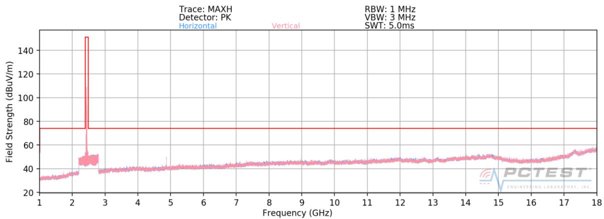
Plot 7-32. Radiated Spurious Plot above 1GHz (802.11b – Ch. 6)
