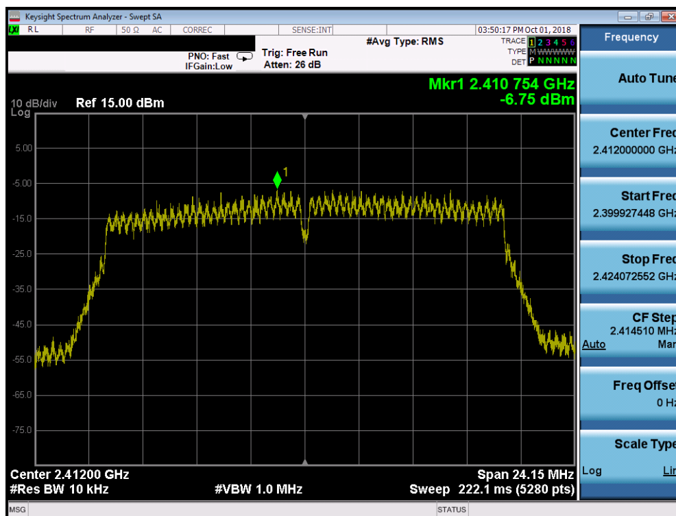
Plot 7-16. Power Spectral Density Plot (802.11n (2.4GHz) – Ch. 1)
