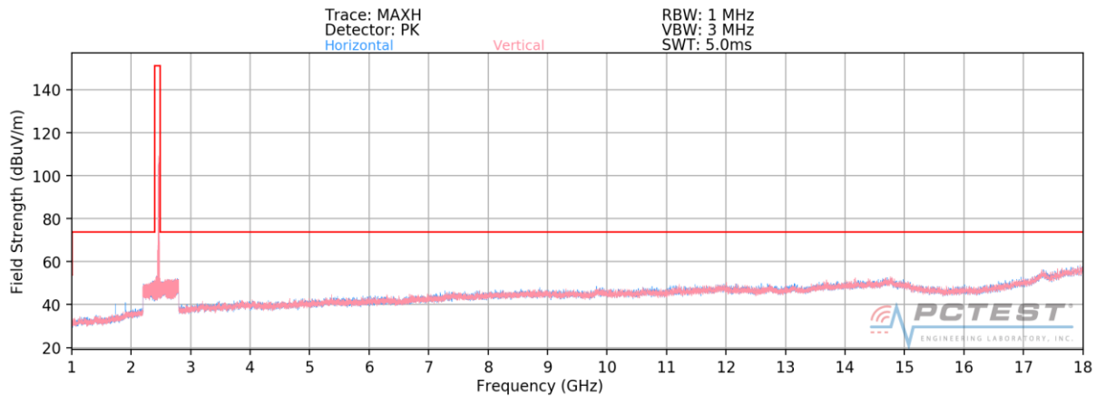
Plot 7-33. Radiated Spurious Plot above 1GHz (802.11b – Ch. 11)
